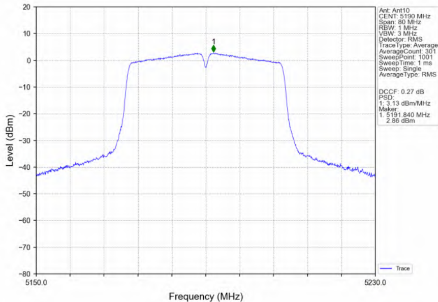
802.11ac(VHT40)_LCH_5190MHz_Ant10_NTNV
