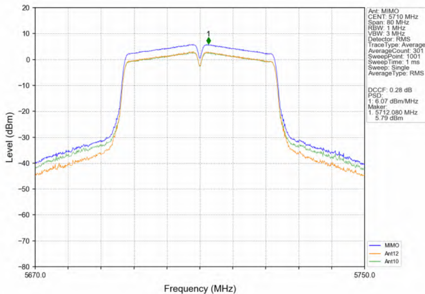
802.11n(HT40)_HCH_5710MHz_MIMO_NTNV
