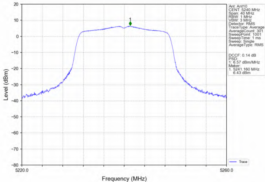
802.11ac(VHT20)_HCH_5240MHz_Ant10_NTNV
