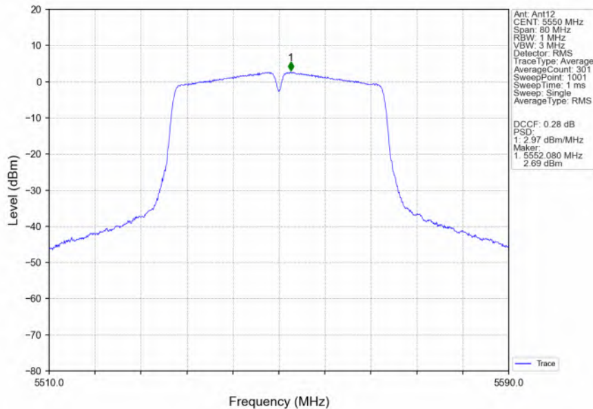
802.11ac(VHT40)_MCH_5550MHz_Ant12_NTNV
