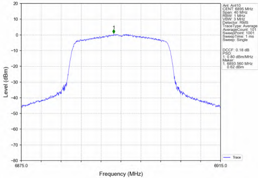
802.11ax(HEW20)_LCH_6895MHz_RU242_Left_MIMO_NTNV
