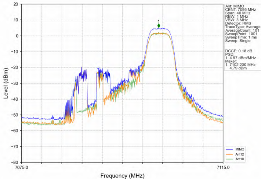
802.11ax(HEW20)_HCH_7095MHz_RU52_Right_MIMO_NTNV
