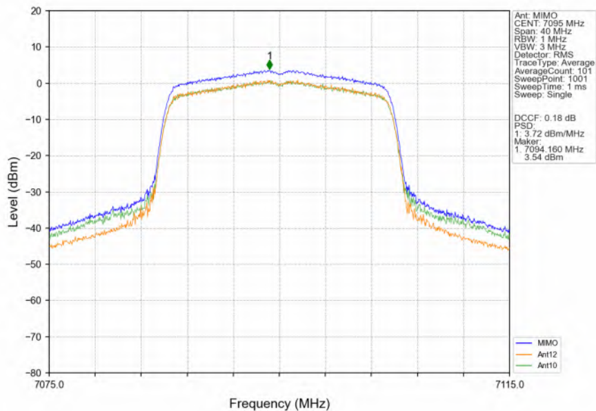
802.11ax(HEW20)_HCH_7095MHz_RU242_Left_MIMO_NTNV
