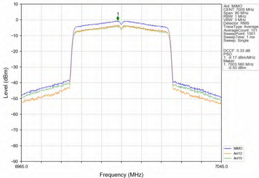
802.11ax(HEW40)_MCH_7005MHz_RU484_Left_MIMO_NTNV
