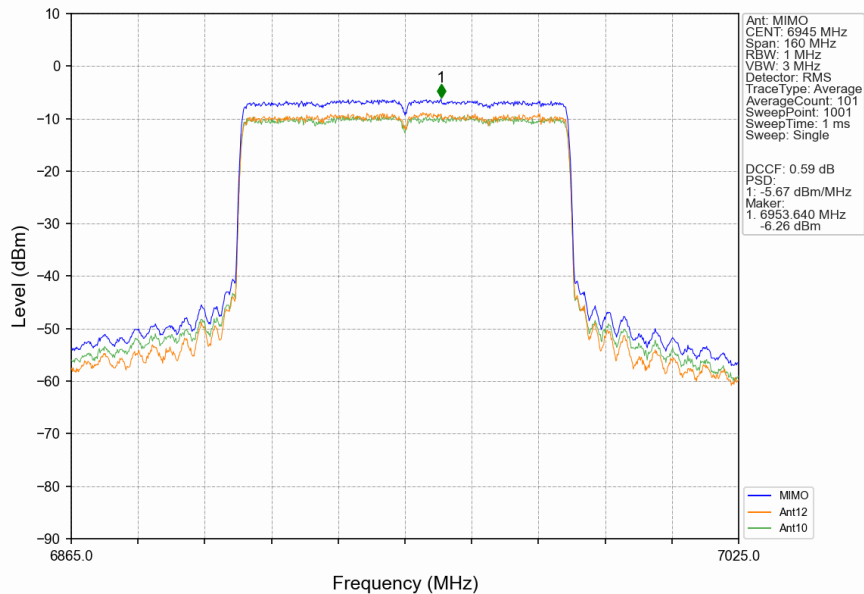
802.11ax(HEW80)_LCH_6945MHz_RU996_Left_MIMO_NTNV
