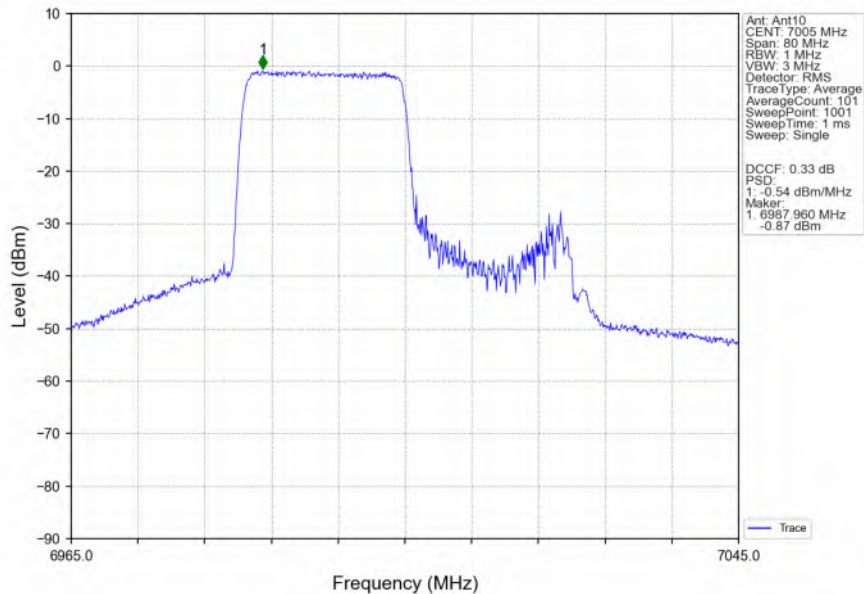
802.11ax(HEW40)_MCH_7005MHz_RU242_Left_Ant10_NTNV
