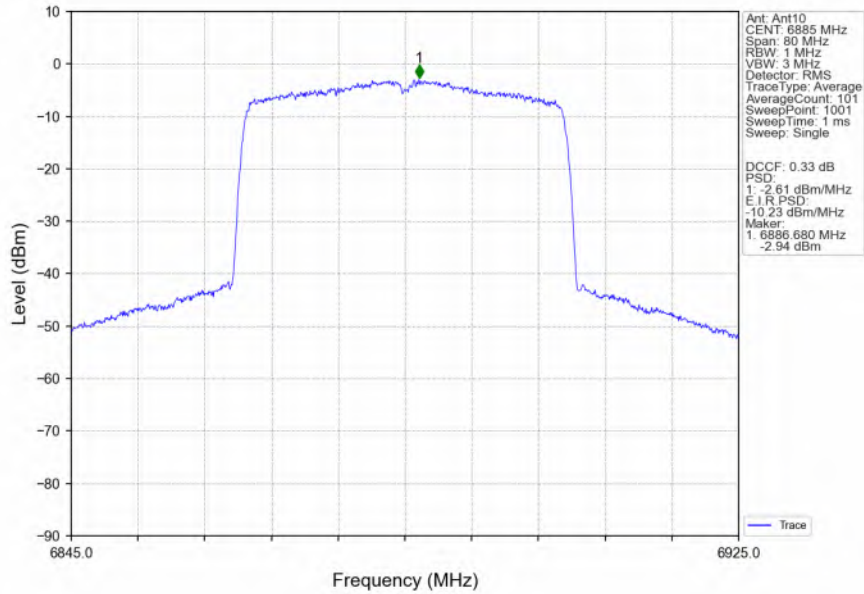
802.11ax(HEW40)_HCH_6885MHz_RU484_Left_MIMO_NTNV
