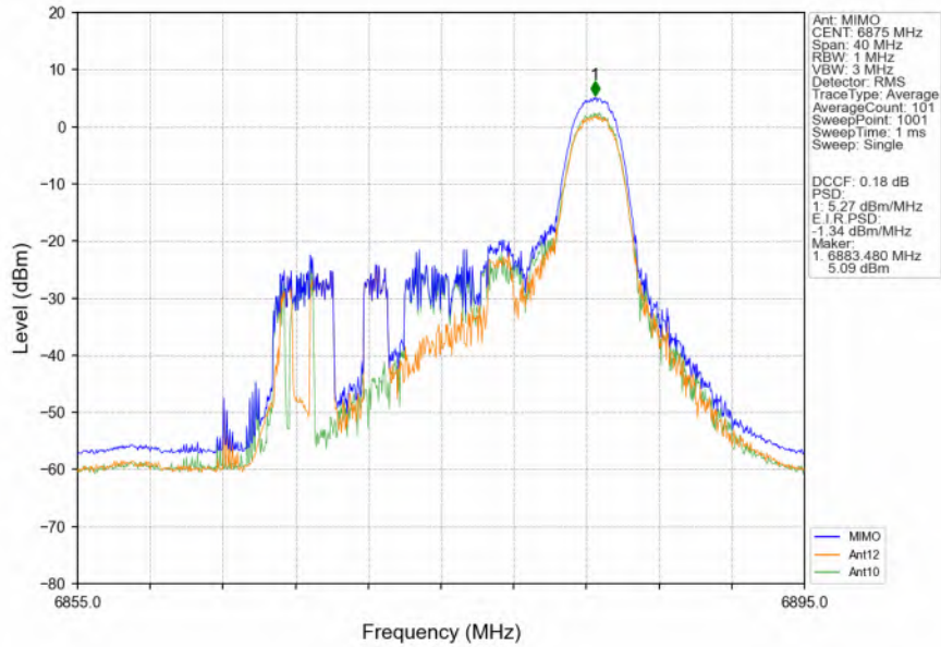
802.11ax(HEW20)_HCH_6875MHz_RU52_Right_Ant12_NTNV
