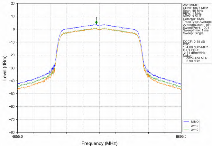
802.11ax(HEW20)_HCH_6875MHz_RU242_Left_MIMO_NTNV
