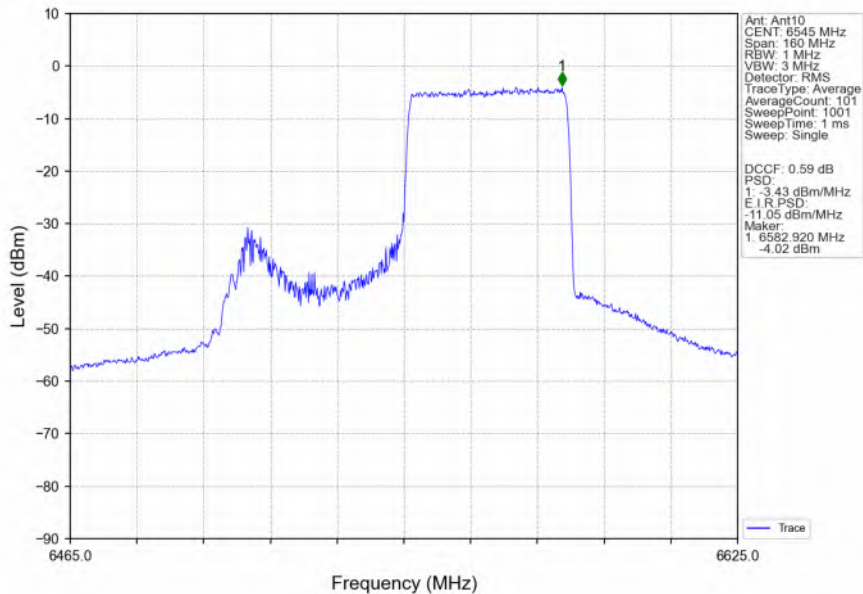
802.11ax(HEW80)_HCH_6545MHz_RU484_Right_Ant10_NTNV
