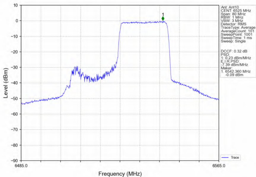
802.11ax(HEW40)_HCH_6525MHz_RU242_Right_Ant10_NTNV
