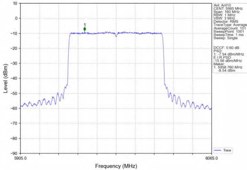
802.11ax(HEW80)_LCH_5985MHz_RU996_Left_MIMO_NTNV
