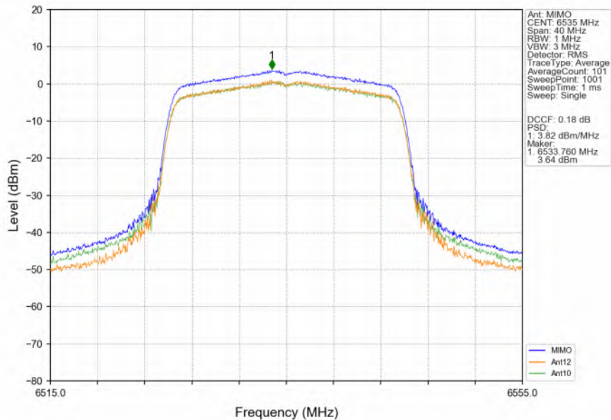
802.11ax(HEW20)_LCH_6535MHz_RU242_Left_MIMO_NTNV
