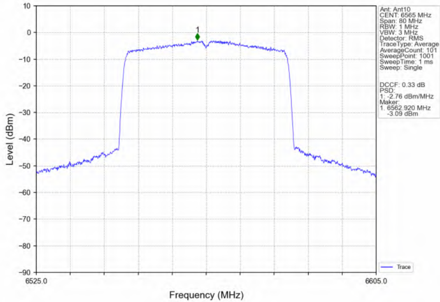
802.11ax(HEW40)_LCH_6565MHz_RU484_Left_MIMO_NTNV
