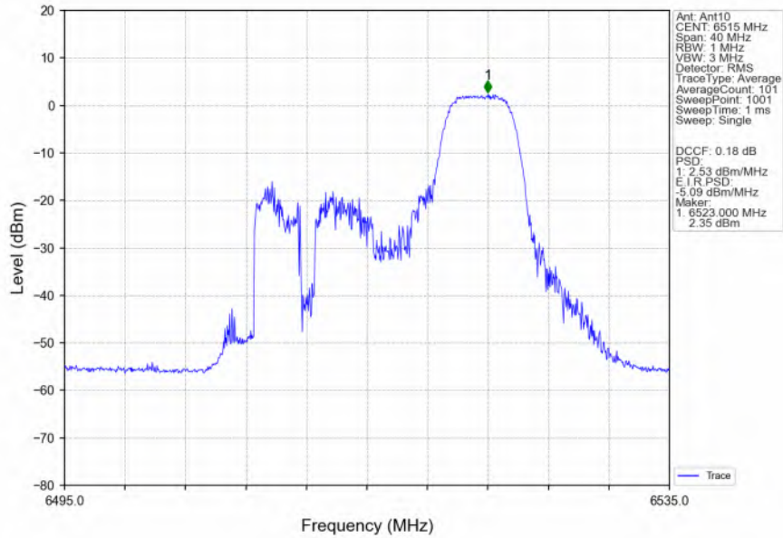
802.11ax(HEW20)_HCH_6515MHz_RU52_Right_MIMO_NTNV
