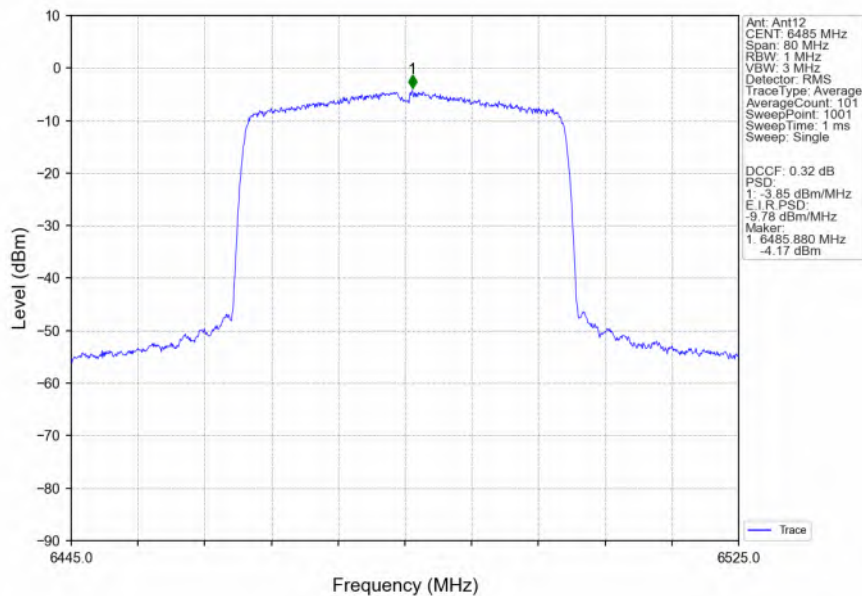
802.11ax(HEW40)_MCH_6485MHz_RU484_Left_Ant12_NTNV
