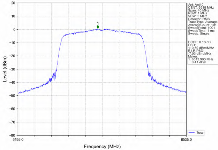
802.11ax(HEW20)_HCH_6515MHz_RU242_Left_MIMO_NTNV
