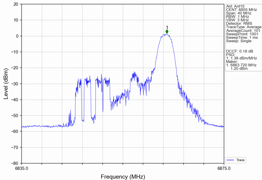
802.11ax(HEW20)_HCH_6855MHz_RU26_Right_Ant10_NTNV
