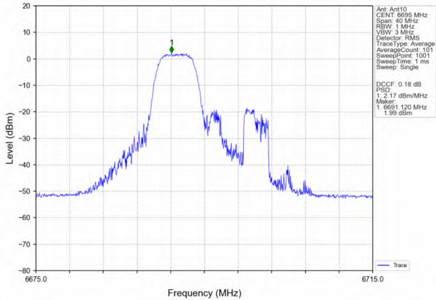
802.11ax(HEW20)_MCH_6695MHz_RU52_Mid_MIMO_NTNV
