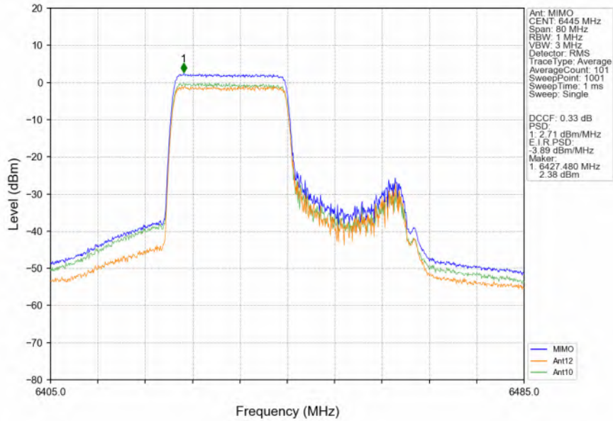
802.11ax(HEW40)_LCH_6445MHz_RU484_Left_Ant12_NTNV
