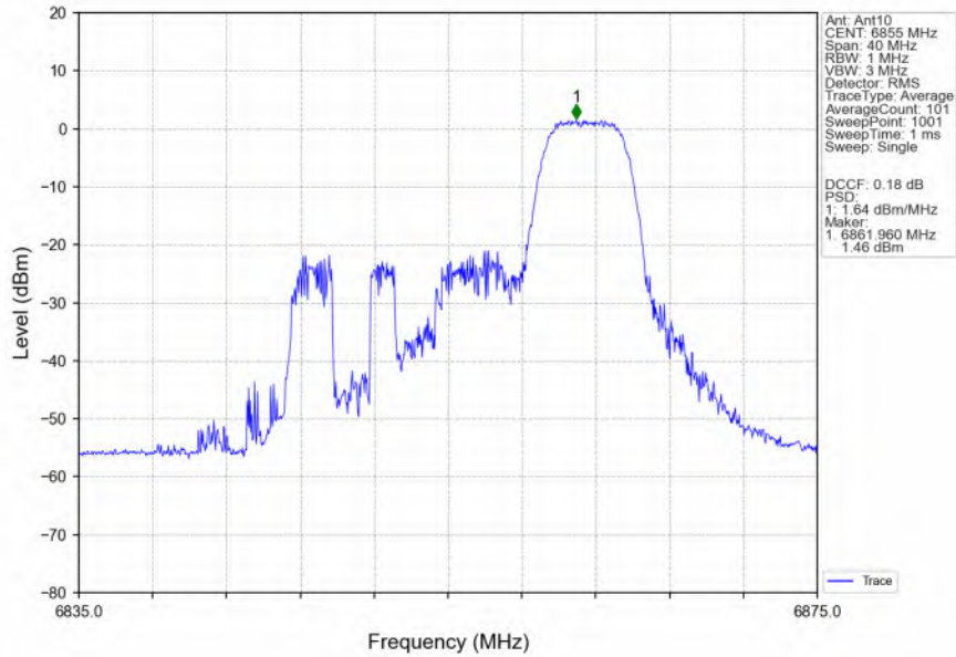
802.11ax(HEW20)_HCH_6855MHz_RU52_Right_MIMO_NTNV
