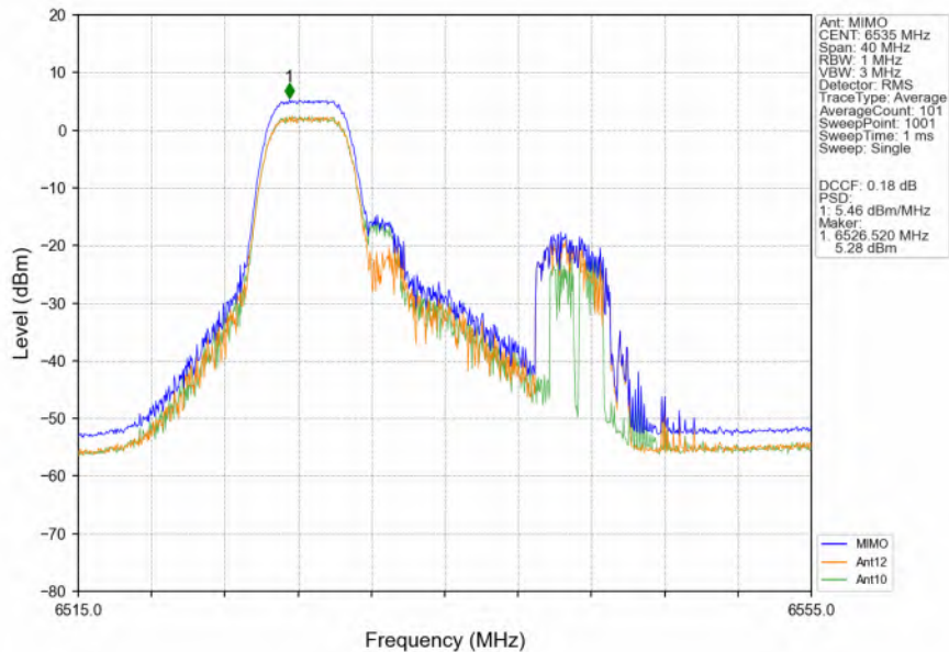
802.11ax(HEW20)_LCH_6535MHz_RU52_Left_MIMO_NTNV
