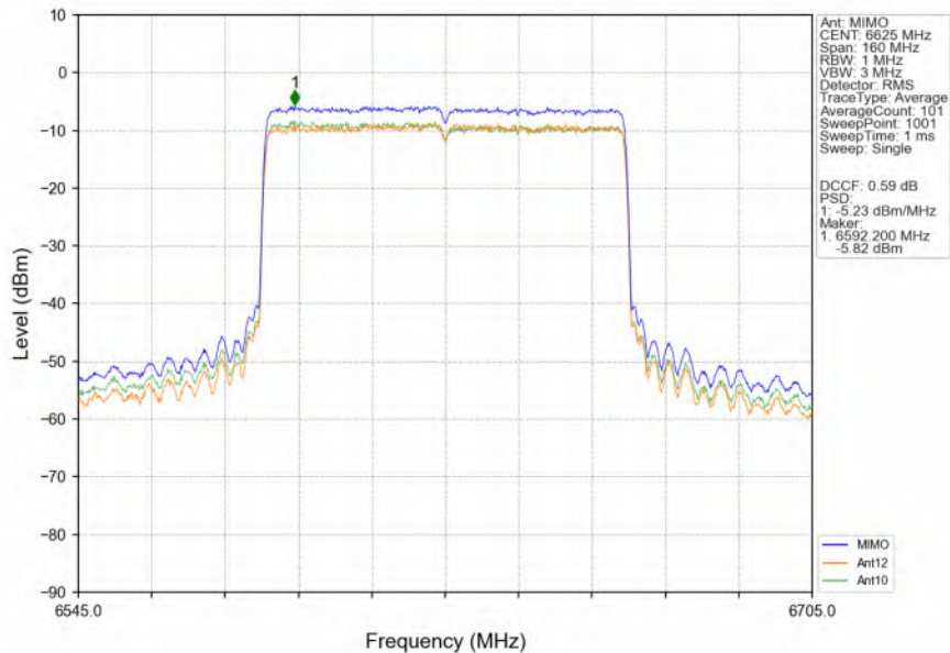
802.11ax(HEW80)_LCH_6625MHz_RU996_Left_MIMO_NTNV
