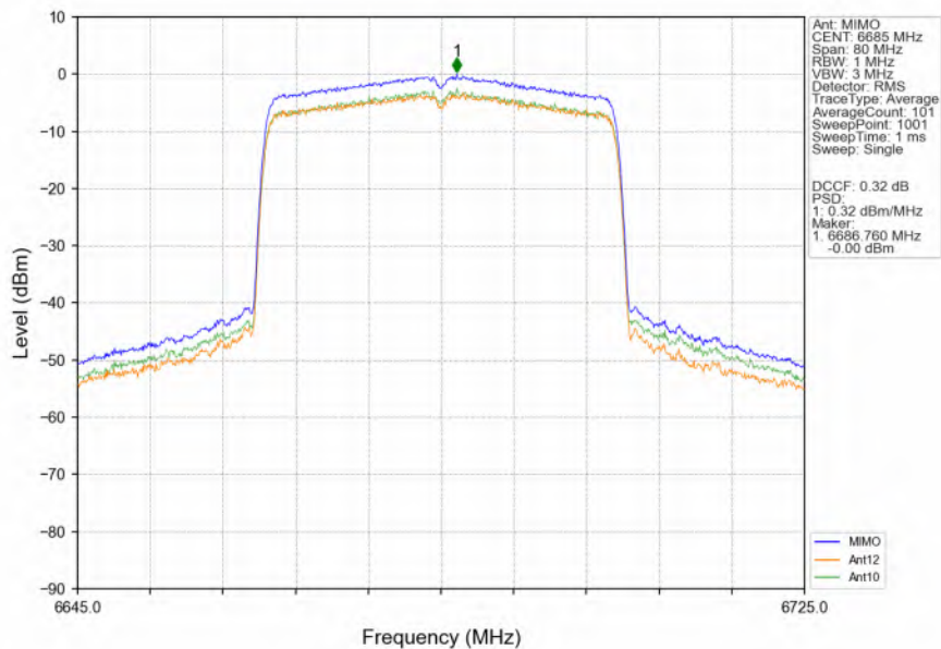
802.11ax(HEW40)_MCH_6685MHz_RU484_Left_MIMO_NTNV
