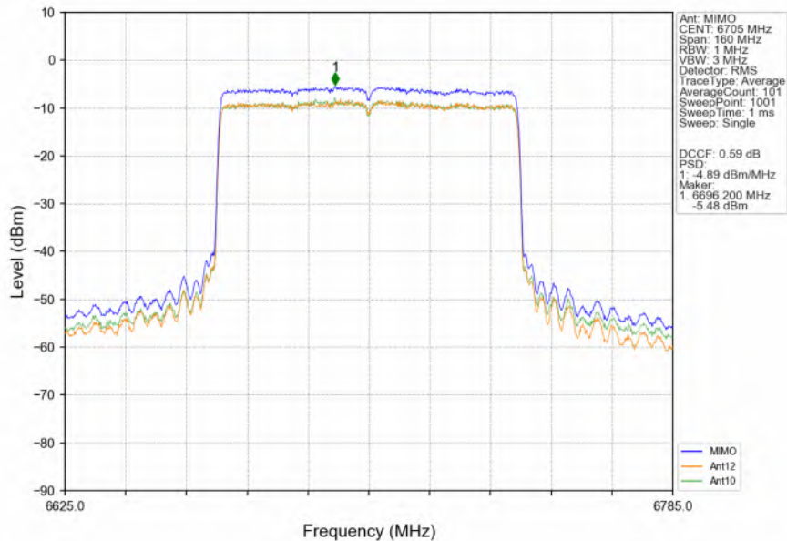
802.11ax(HEW80)_MCH_6705MHz_RU996_Left_MIMO_NTNV
