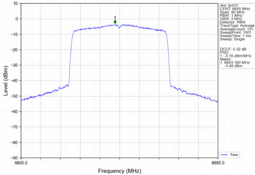
802.11ax(HEW40)_HCH_6845MHz_RU484_Left_MIMO_NTNV
