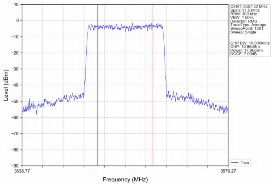
n48_30kHz_SISO_NTNV_15MHz_CP-OFDM_QPSK_3557.52MHz_Inner_Full_Ant4
