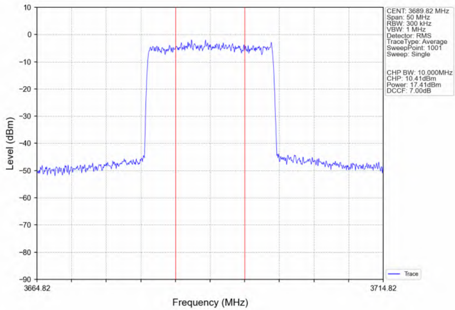
n48_30kHz_SISO_NTNV_20MHz_DFT-s-OFDM_QPSK_3690MHz_Inner_Full_Ant4
