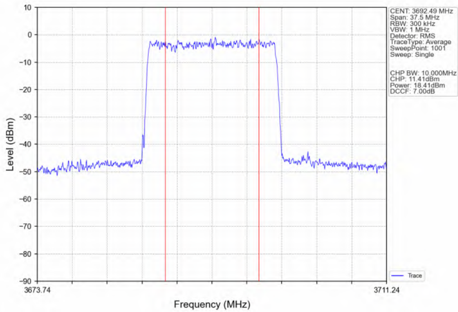
n48_30kHz_SISO_NTNV_15MHz_CP-OFDM_16_QAM_3692.49MHz_Inner_Full_Ant4
