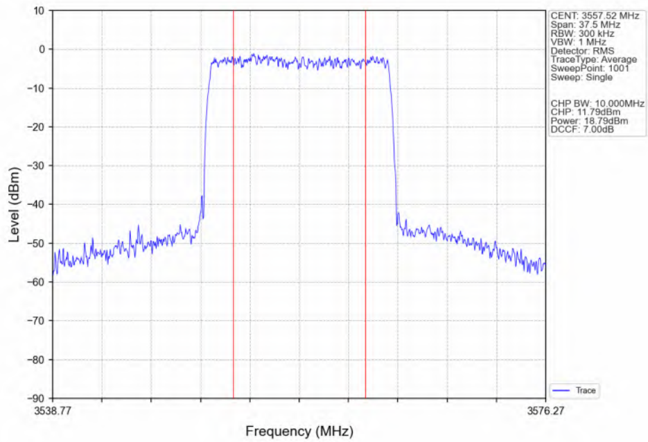
n48_30kHz_SISO_NTNV_15MHz_CP-OFDM_16QAM_3557.52MHz_Inner_Full_Ant4
