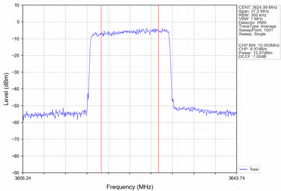
n48_30kHz_SISO_NTNV_15MHz_CP-OFDM_256_QAM_3624.99MHz_Inner_Full_Ant4
