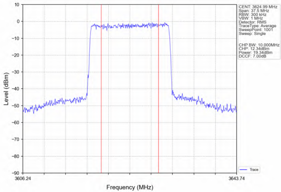
n48_30kHz_SISO_NTNV_15MHz_CP-OFDM_QPSK_3624.99MHz_Inner_Full_Ant4
