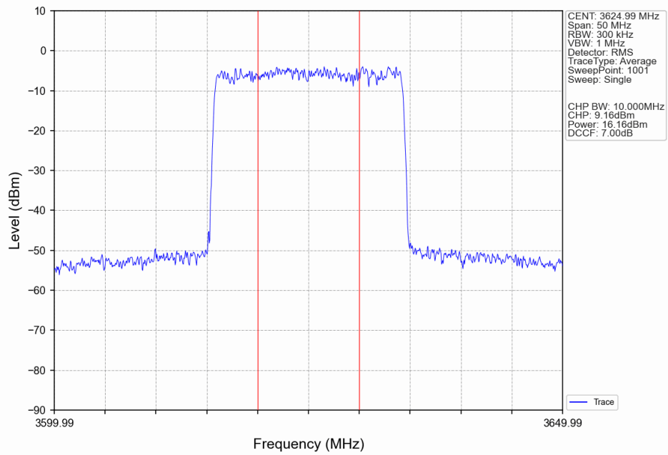
n48_30kHz_SISO_NTNV_20MHz_CP-OFDM_64_QAM_3624.99MHz_Inner_Full_Ant4
