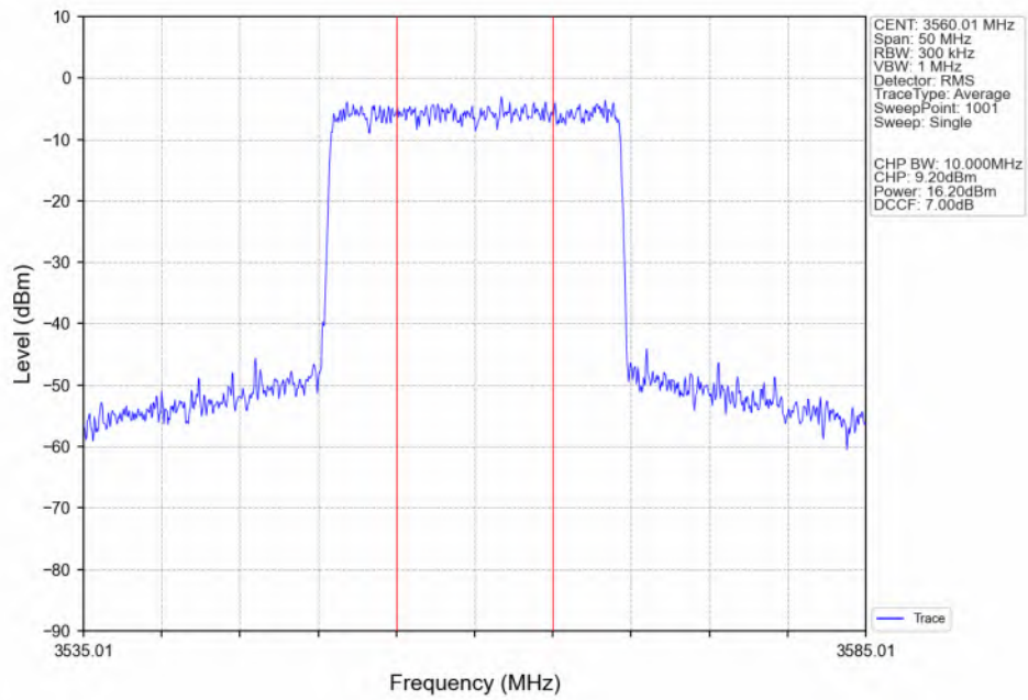
n48_30kHz_SISO_NTNV_20MHz_CP-OFDM_QPSK_3560.01MHz_Inner_Full_Ant4
