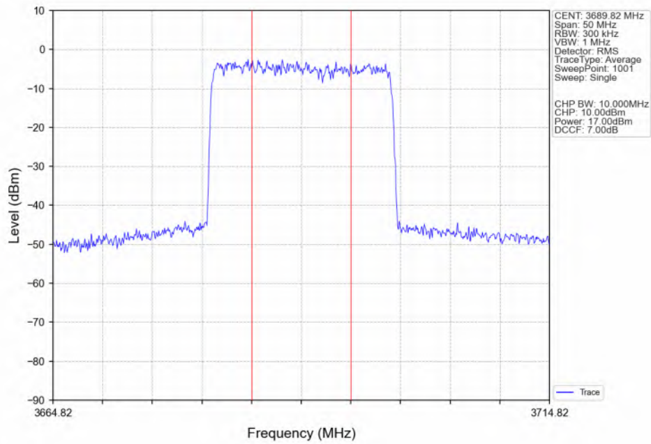
n48_30kHz_SISO_NTNV_20MHz_DFT-s-OFDM_16QAM_3690MHz_Inner_Full_Ant4
