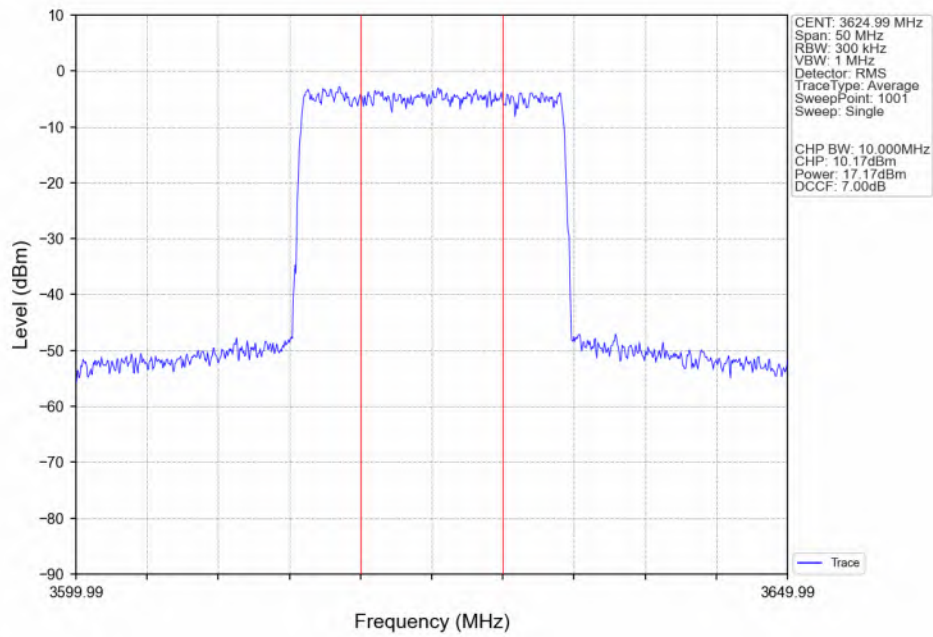
n48_30kHz_SISO_NTNV_20MHz_CP-OFDM_16_QAM_3624.99MHz_Inner_Full_Ant4
