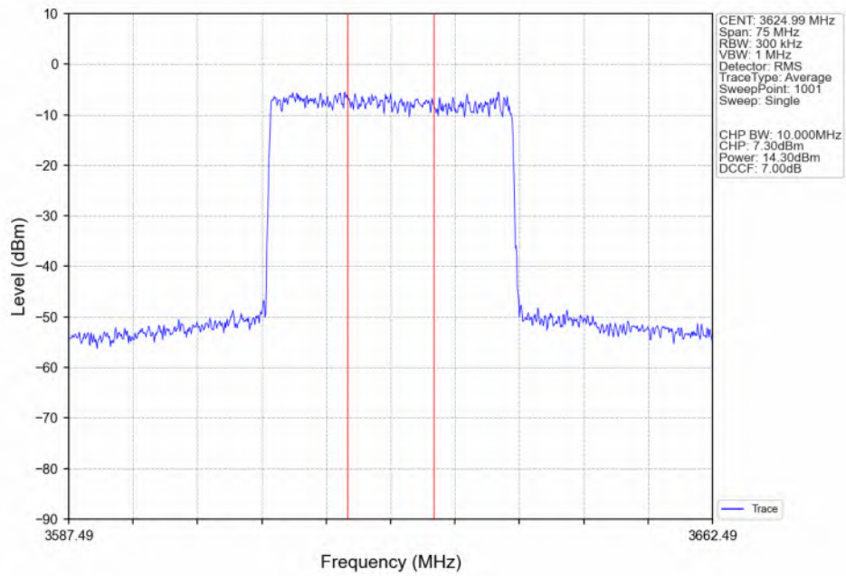
n48_30kHz_SISO_NTNV_30MHz_CP-OFDM_16_QAM_3624.99MHz_Inner_Full_Ant4
