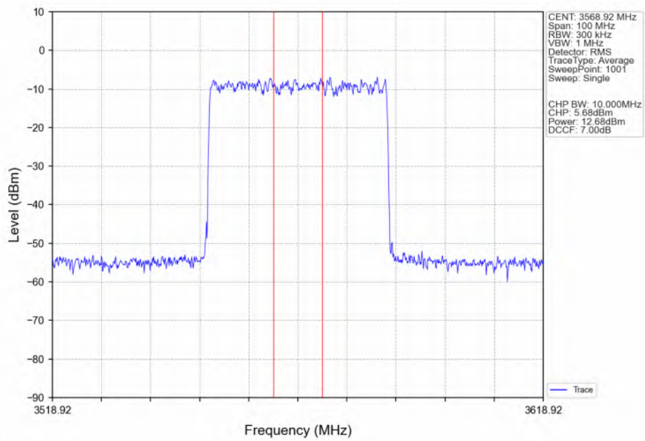
n48_30kHz_SISO_NTNV_40MHz_DFT-s-OFDM_256_QAM_3570MHz_Inner_Full_Ant4
