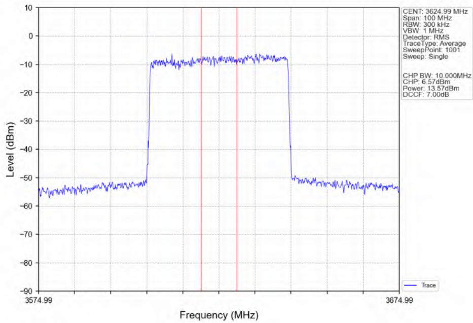
n48_30kHz_SISO_NTNV_40MHz_CP-OFDM_64_QAM_3624.99MHz_Inner_Full_Ant4
