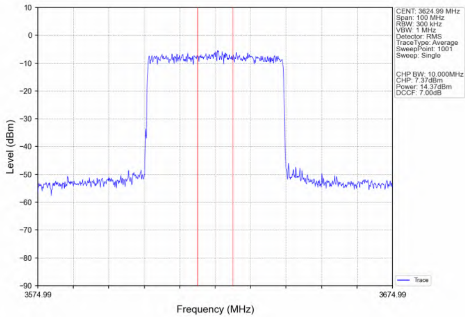
n48_30kHz_SISO_NTNV_40MHz_CP-OFDM_16_QAM_3624.99MHz_Inner_Full_Ant4
