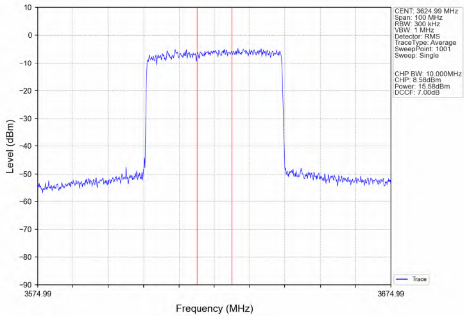
n48_30kHz_SISO_NTNV_40MHz_CP-OFDM_QPSK_3624.99MHz_Inner_Full_Ant4
