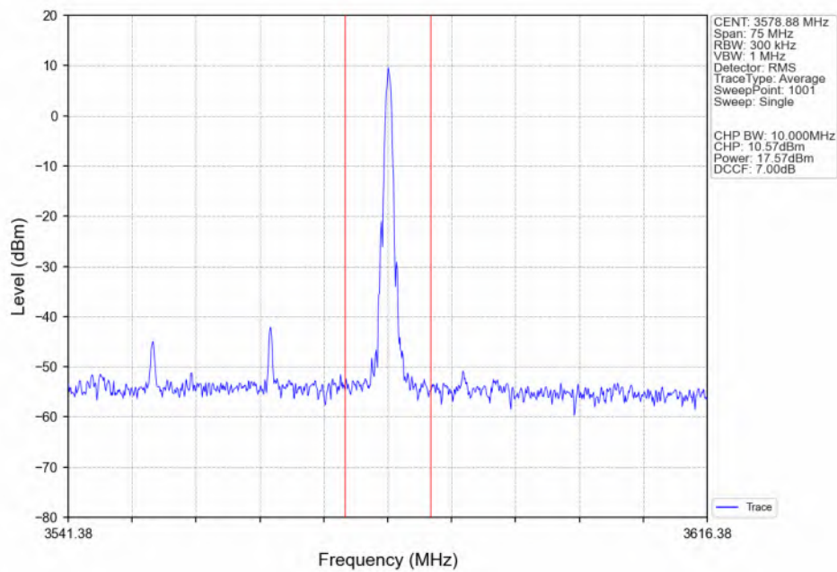
n48_30kHz_SISO_NTNV_30MHz_CP-OFDM_256_QAM_3565.02MHz_Edge_1RB_Right_Ant4
