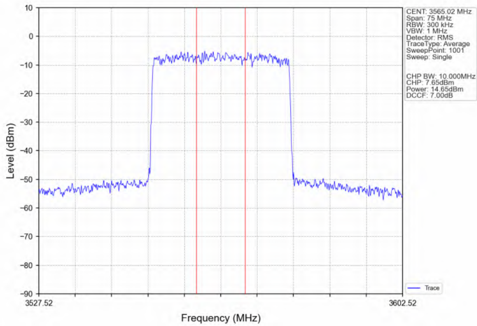
n48_30kHz_SISO_NTNV_30MHz_CP-OFDM_64_QAM_3565.02MHz_Inner_Full_Ant4
