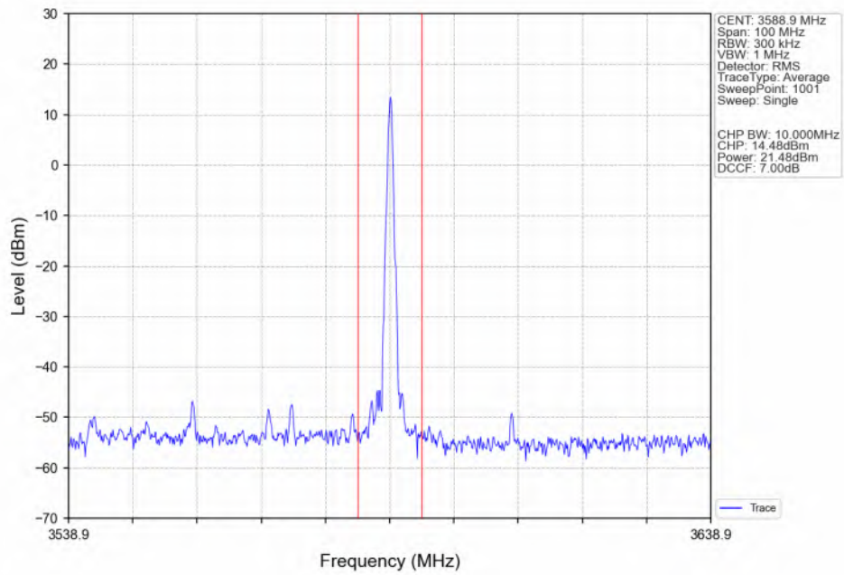
n48_30kHz_SISO_NTNV_40MHz_DFT-s-OFDM_QPSK_3570MHz_Edge_1RB_Right_Ant4
