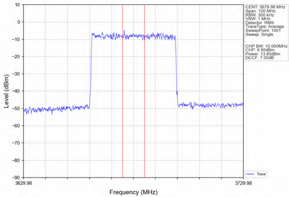
n48_30kHz_SISO_NTNV_40MHz_CP-OFDM_QPSK_3679.98MHz_Inner_Full_Ant4
