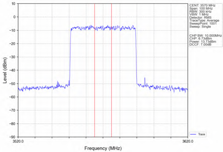
n48_30kHz_SISO_NTNV_40MHz_CP-OFDM_16QAM_3570MHz_Inner_Full_Ant4
