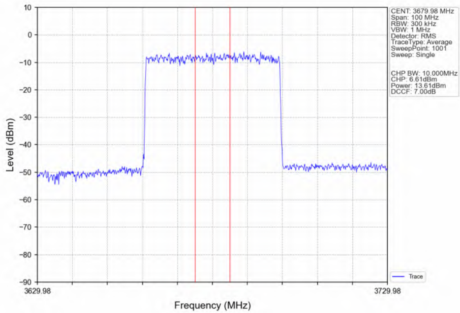
n48_30kHz_SISO_NTNV_40MHz_CP-OFDM_64_QAM_3679.98MHz_Inner_Full_Ant4
