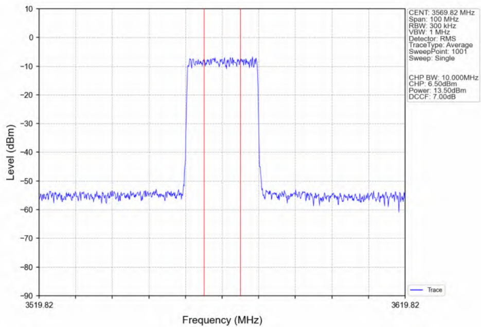
n48_30kHz_SISO_NTNV_40MHz_CP-OFDM_256_QAM_3570MHz_Inner_Full_Ant4
