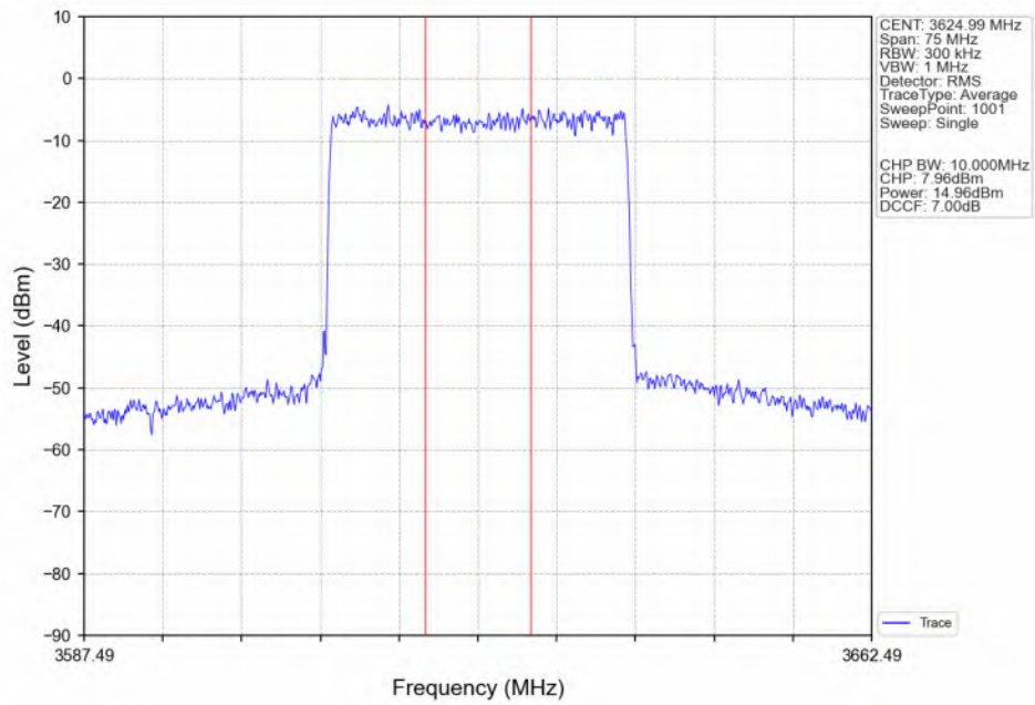
n48_30kHz_SISO_NTNV_30MHz_CP-OFDM_QPSK_3624.99MHz_Inner_Full_Ant4
