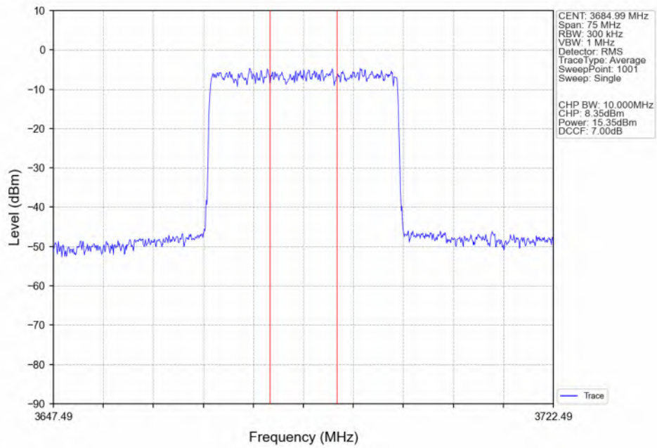
n48_30kHz_SISO_NTNV_30MHz_CP-OFDM_64_QAM_3684.99MHz_Inner_Full_Ant4
