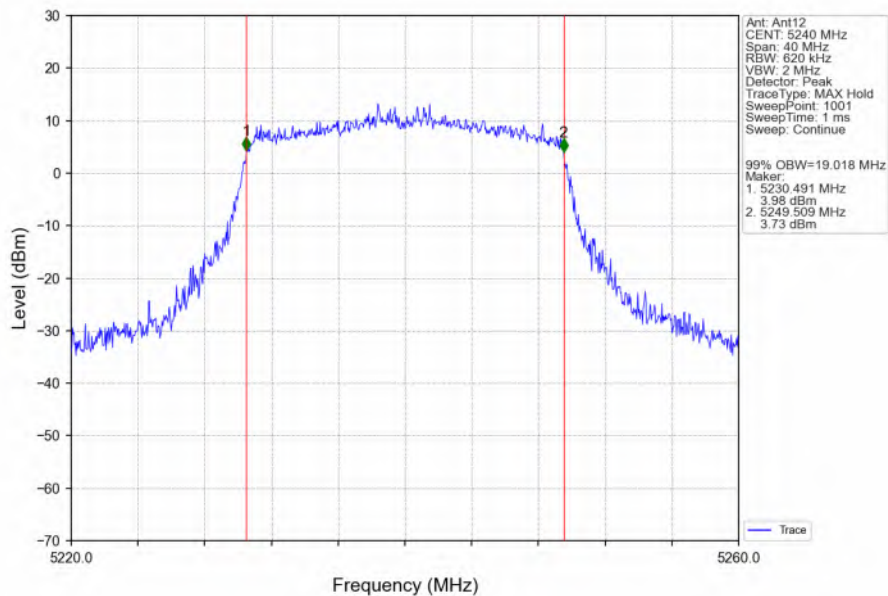
802.11ax(HEW20)_HCH_5240MHz_RU242_Left_Ant12_NTNV
