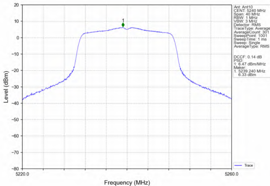
802.11ac(VHT20)_HCH_5240MHz_Ant10_NTNV
