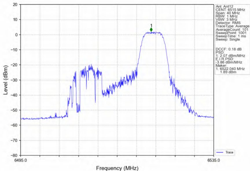
802.11ax(HEW20) HCH 6515MHz RU52 Right Ant12 NTNW
