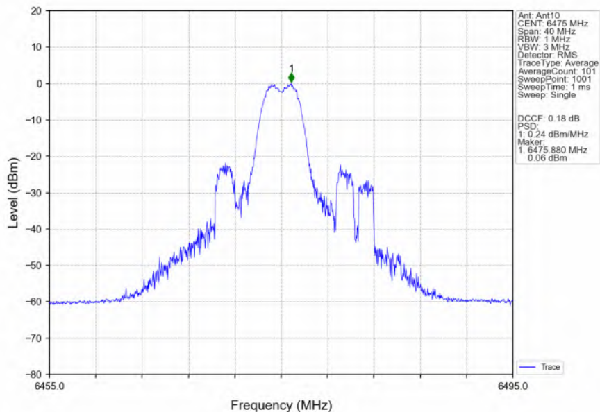
802.11ax(HEW20) MCH 6475MHz RU26 Mid_Ant10 NTN
