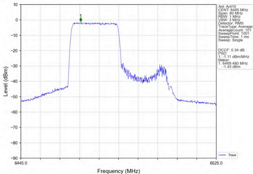
802.11ax(HEW40) MCH_6485MHz RU242 Left_Ant10 NTN
