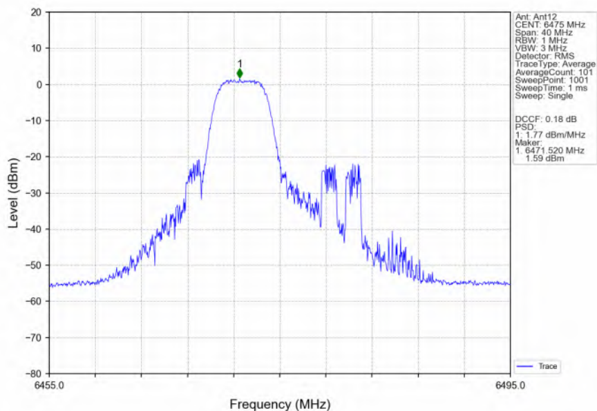
802.11ax(HEW20)_MCH_6475MHz_RU52_Mid_Ant12_NTNV
