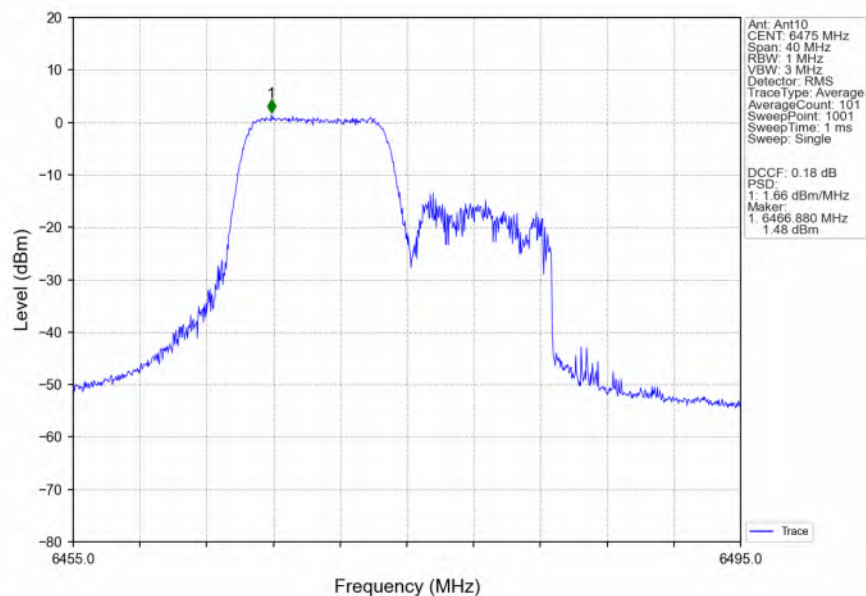
802.11ax(HEW20) MCH_6475MHz RU106 Left_Ant10_NTNV
