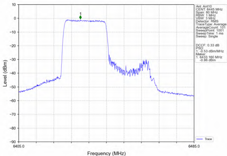
802.11ax(HEW40) LCH 6445MHz RU242 Left_Ant10 NTN
