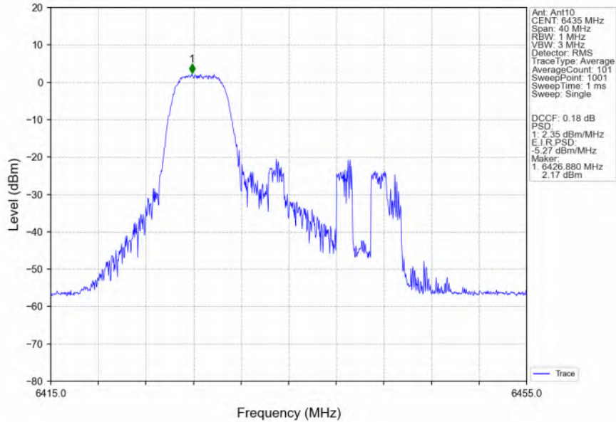
802.11ax(HEW20)_LCH_6435MHz_RU52_Left_MIMO_NTNV
