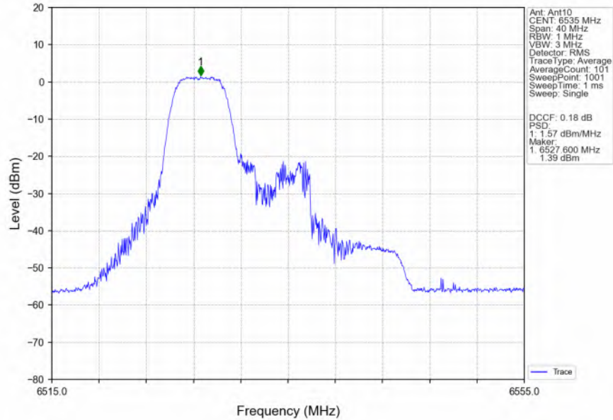
802.11ax(HEW20)_LCH_6535MHz_RU52_Left_MIMO_NTNV
