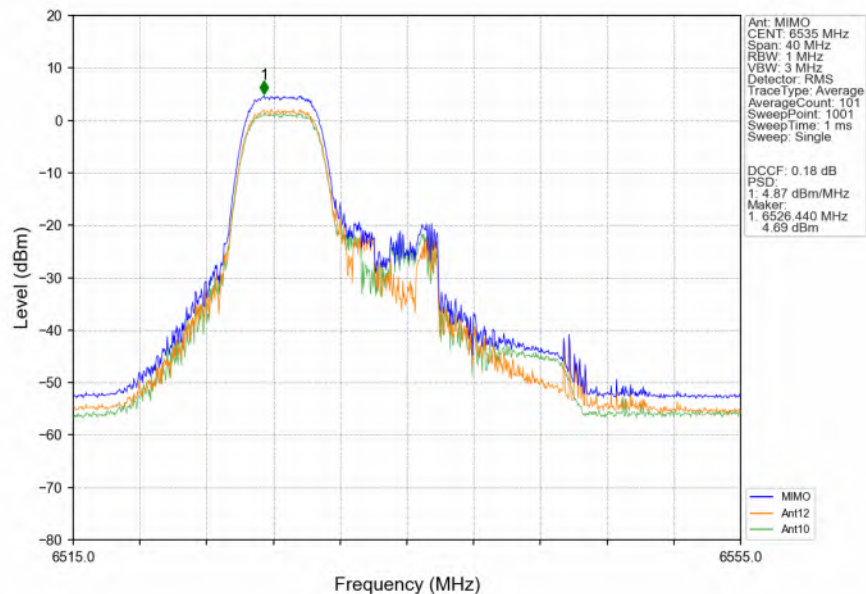
802.11ax(HEW20)_LCH_6535MHz_RU52_Left_MIMO_NTNV
