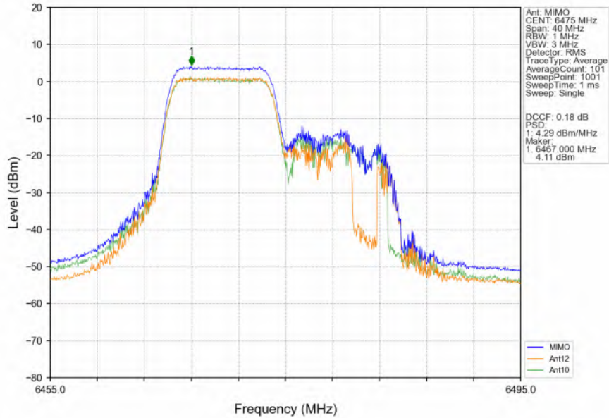
802.11ax(HEW20) MCH_6475MHz RU242 Left Ant12 NTN7
