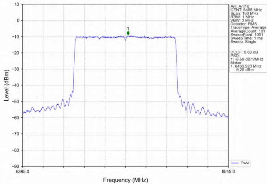
802.11ax(HEW80) LCH 6465MHz RU996 Left_MIMO_NTNV
