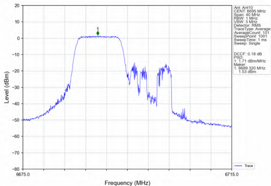
802.11ax(HEW20) MCH_6695MHz RU106 Left_Ant10_NTNV
