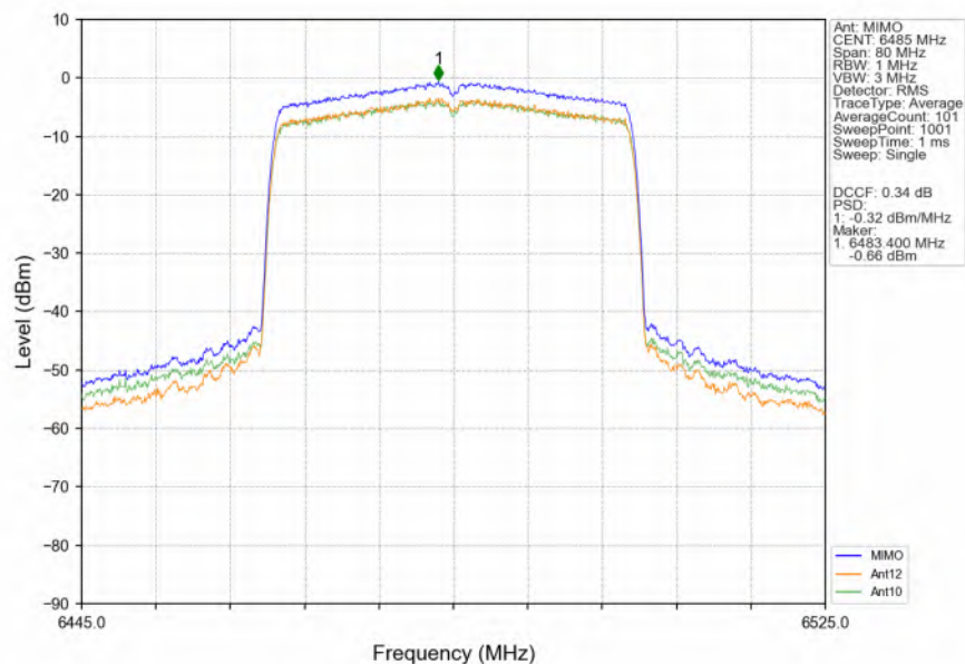
802.11ax(HEW40) MCH_6485MHz RU484 Left_MIMO_NTNV
