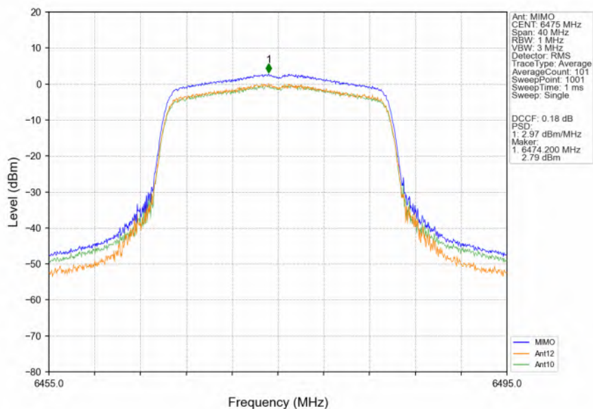
802.11ax(HEW20) MCH_6475MHz RU242 Left_MIMO_NTNV
