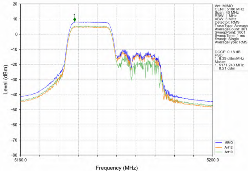
802.11ax(HEW20)_LCH_5180MHz_RU106_Left_MIMO_NTNV
