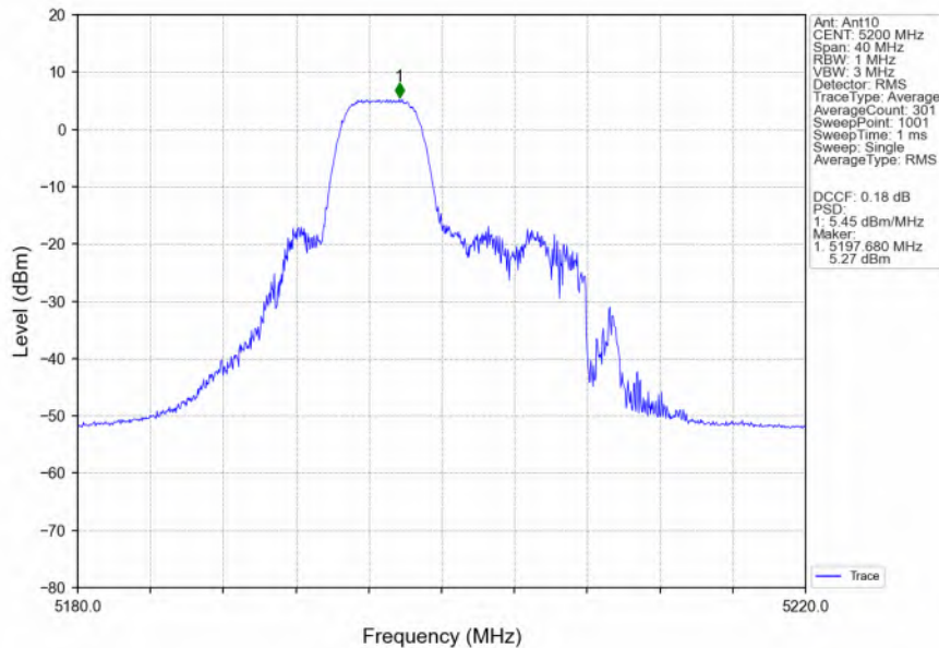
802.11ax(HEW20)_MCH_5200MHz_RU52_Mid_Ant10_NTNV
