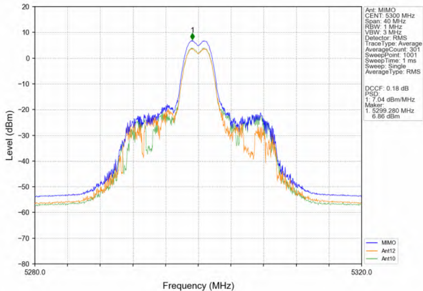
802.11ax(HEW20)_MCH_5300MHz_RU26_Mid_MIMO_NTNV
