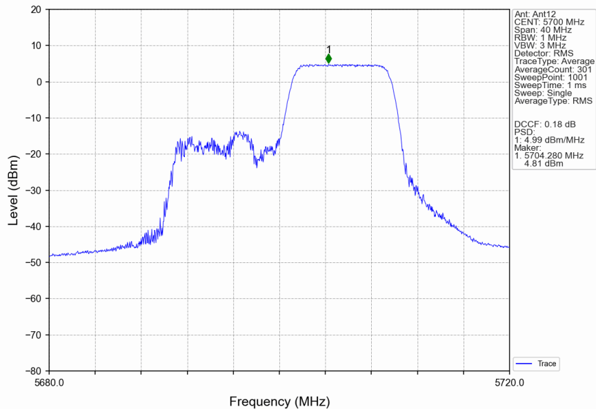
802.11ax(HEW20)_HCH_5700MHz_RU106_Right_Ant12_NTNV
