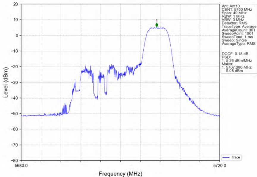
802.11ax(HEW20)_HCH_5700MHz_RU52_Right_Ant10_NTNV
