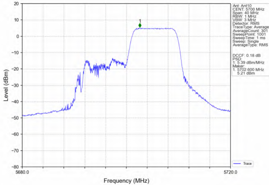
802.11ax(HEW20)_HCH_5700MHz_RU106_Right_MIMO_NTNV
