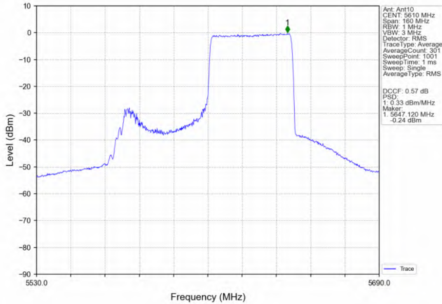
802.11ax(HEW80)_HCH_5610MHz_RU484_Right_MIMO_NTNV
