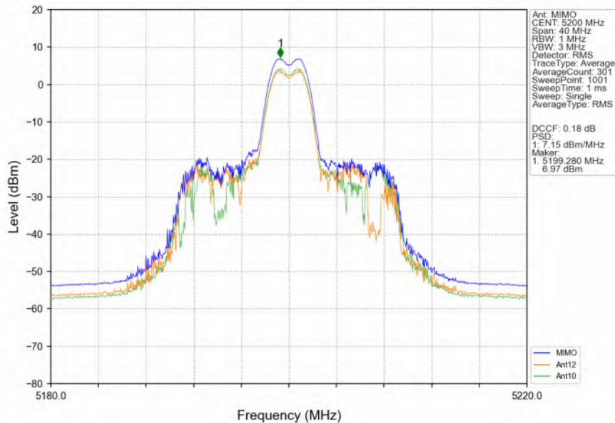
802.11ax(HEW20)_MCH_5200MHz_RU26_Mid_MIMO_NTNV
