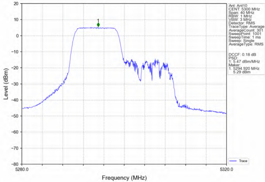
802.11ax(HEW20)_MCH_5300MHz_RU106_Left_MIMO_NTNV
