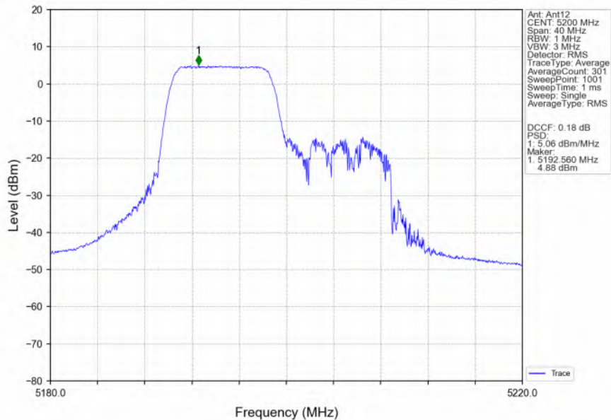
802.11ax(HEW20)_MCH_5200MHz_RU106_Left_Ant12_NTNV
