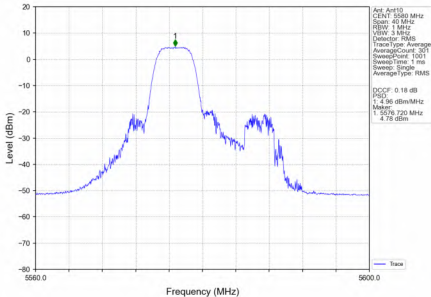
802.11ax(HEW20)_MCH_5580MHz_RU52_Mid_Ant10_NTNV
