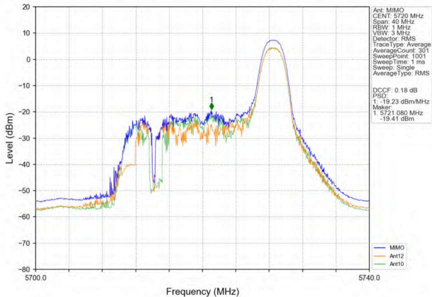
802.11ax(HEW20)_HCH_5720MHz_RU26_Right_MIMO_NTNV
