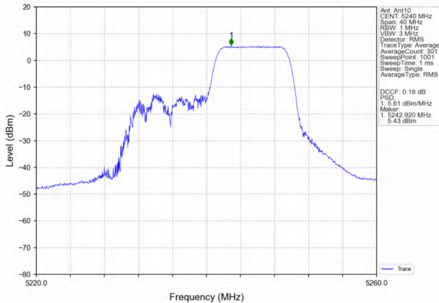
802.11ax(HEW20)_HCH_5240MHz_RU106_Right_MIMO_NTNV
