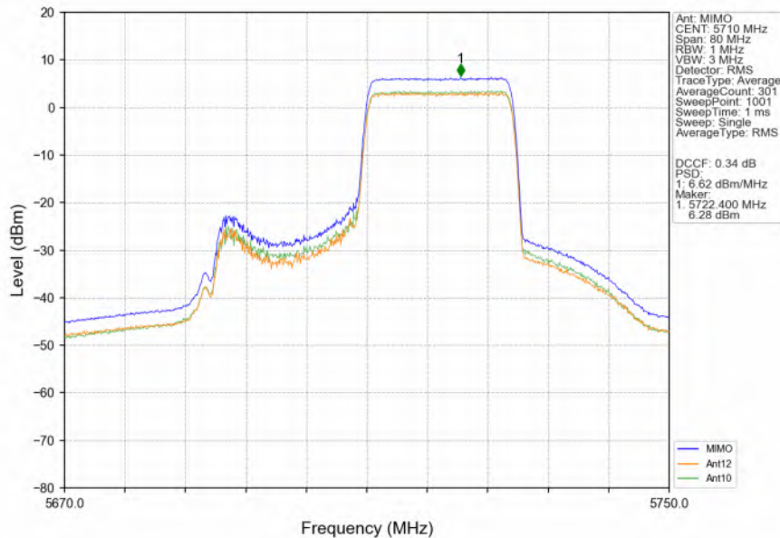
802.11ax(HEW40)_HCH_5710MHz_RU242_Right_MIMO_NTNV
