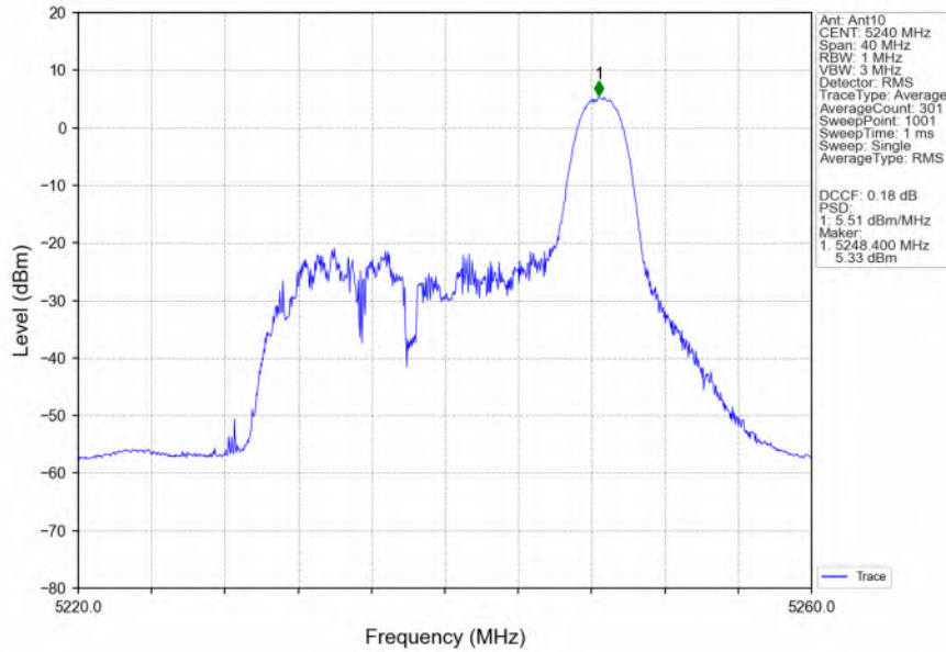
802.11ax(HEW20)_HCH_5240MHz_RU26_Right_MIMO_NTNV
