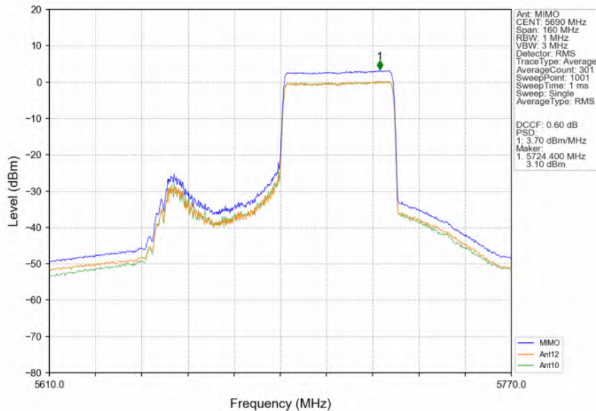
802.11ax(HEW80)_HCH_5690MHz_RU484_Right_MIMO_NTNV
