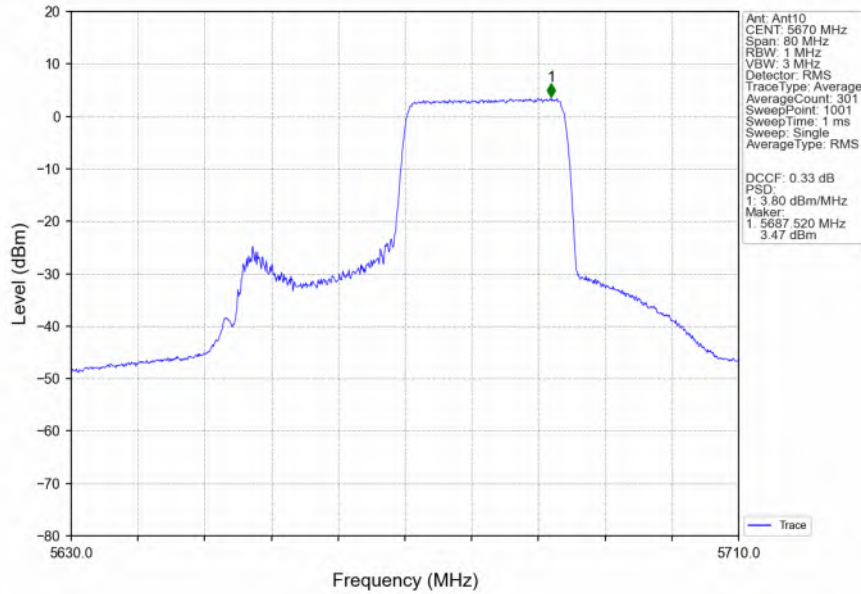
802.11ax(HEW40)_HCH_5670MHz_RU242_Right_MIMO_NTNV
