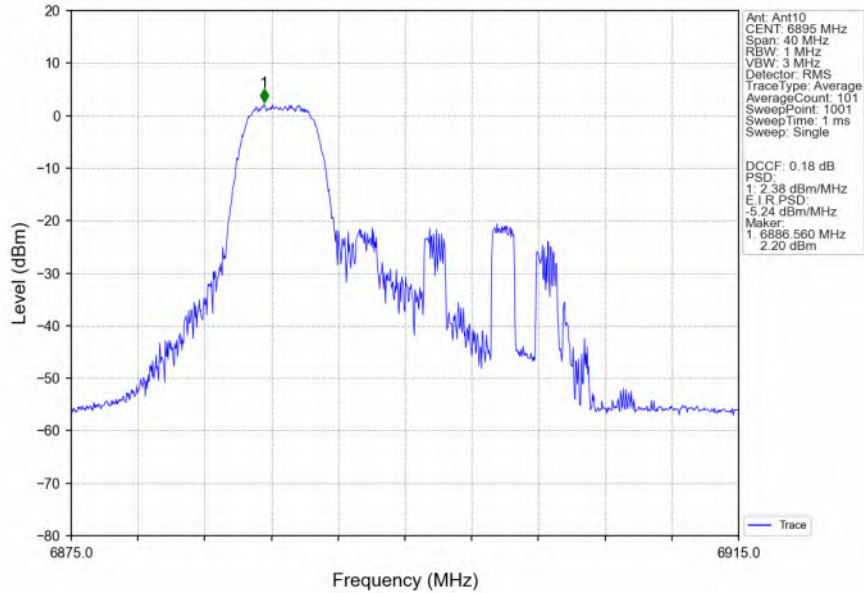
802.11ax(HEW20)_LCH_6895MHz_RU52_Left_MIMO_NTNV
