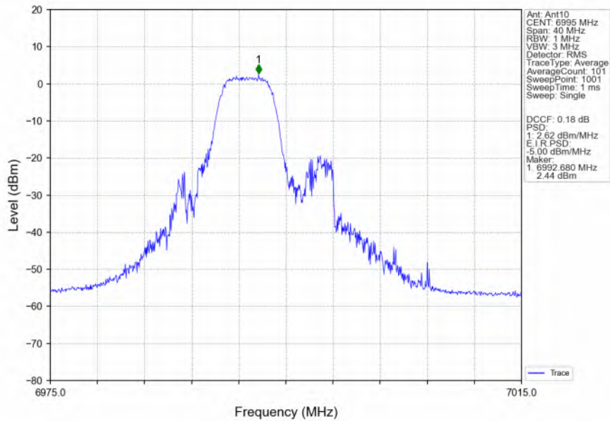
802.11ax(HEW20)_MCH_6995MHz_RU52_Mid_MIMO_NTNV
