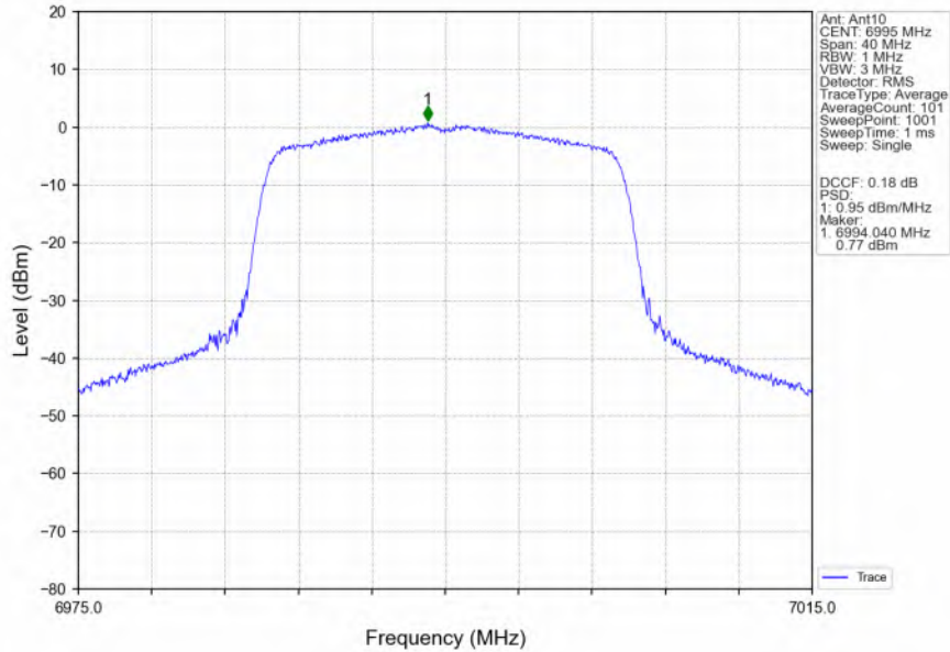
802.11ax(HEW20) MCH_6995MHz RU242 Left_MIMO_NTNV
