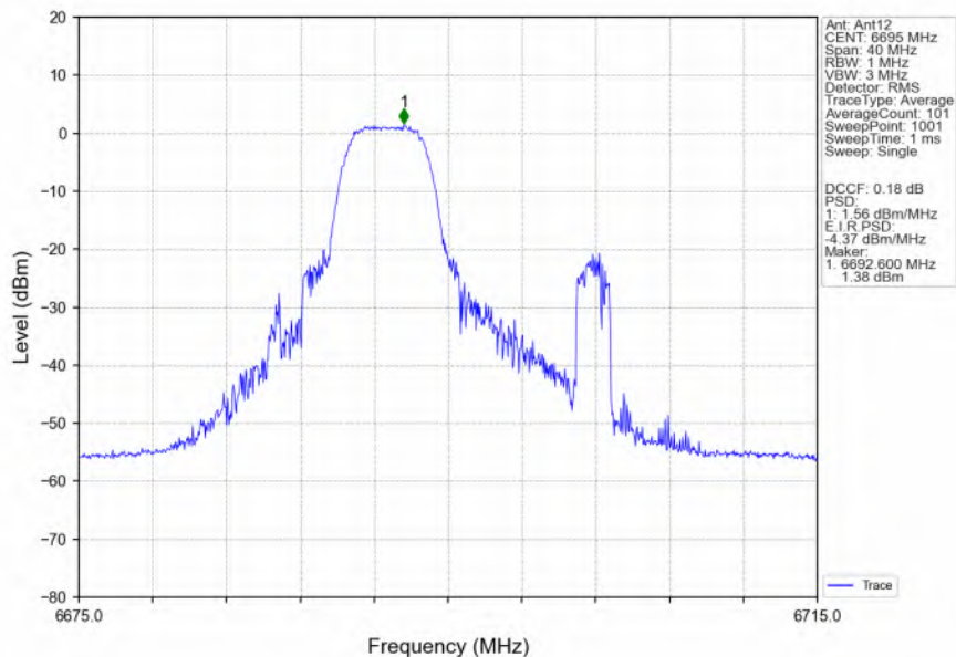
802.11ax(HEW20)_MCH_6695MHz_RU52_Mid_Ant12_NTNV
