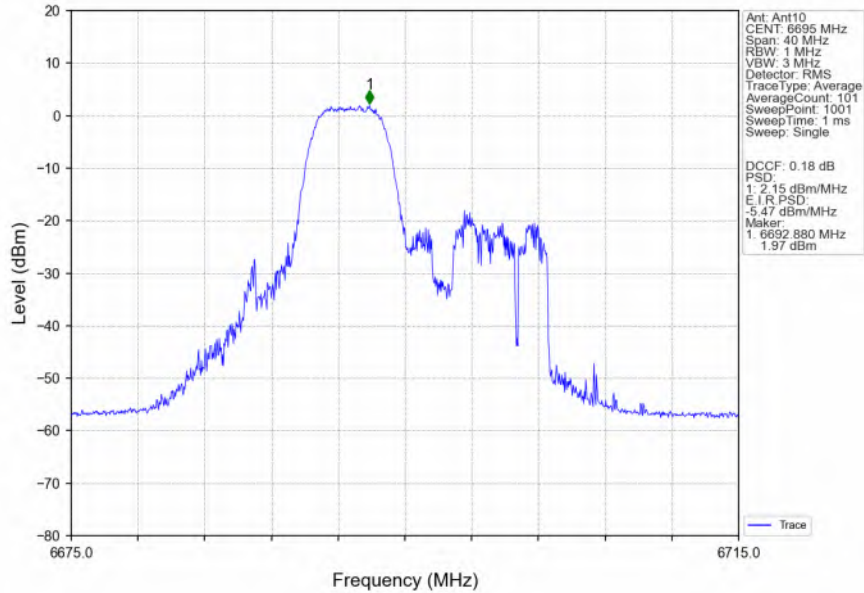
802.11ax(HEW20)_MCH_6695MHz_RU52_Mid_MIMO_NTNV
