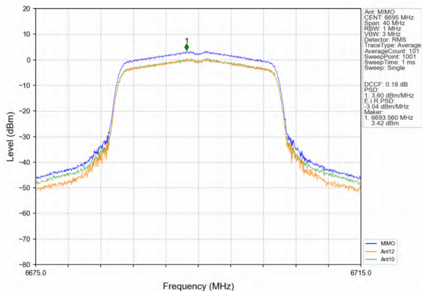
802.11ax(HEW20) MCH_6695MHz RU242 Left_MIMO_NTNV
