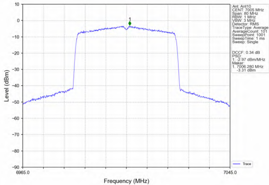
802.11ax(HEW40) MCH_7005MHz RU484 Left_MIMO_NTNV
