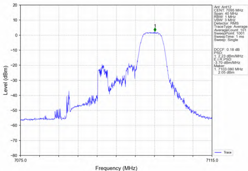
802.11ax(HEW20) HCH 7095MHz RU52 Right Ant12 NTN
