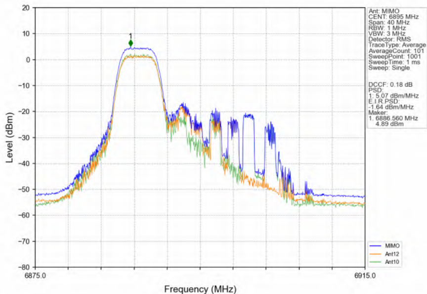
802.11ax(HEW20)_LCH_6895MHz_RU52_Left_MIMO_NTNV
