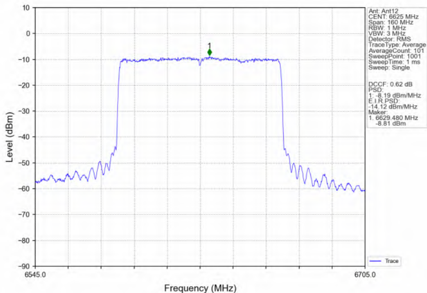
802.11ax(HEW80) LCH 6625MHz RU996 Left Ant12 NTN
