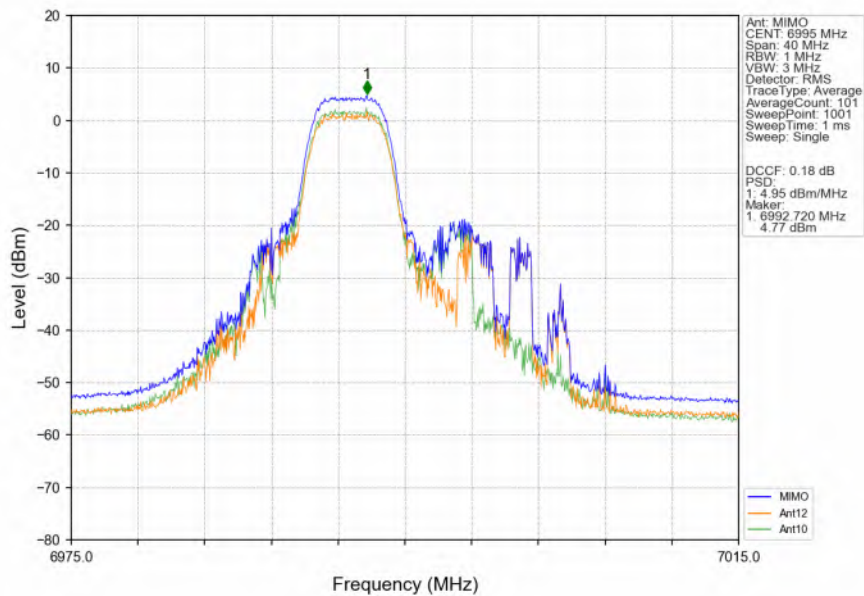
802.11ax(HEW20) MCH 6995MHz RU52 Mid MIMO NTN
