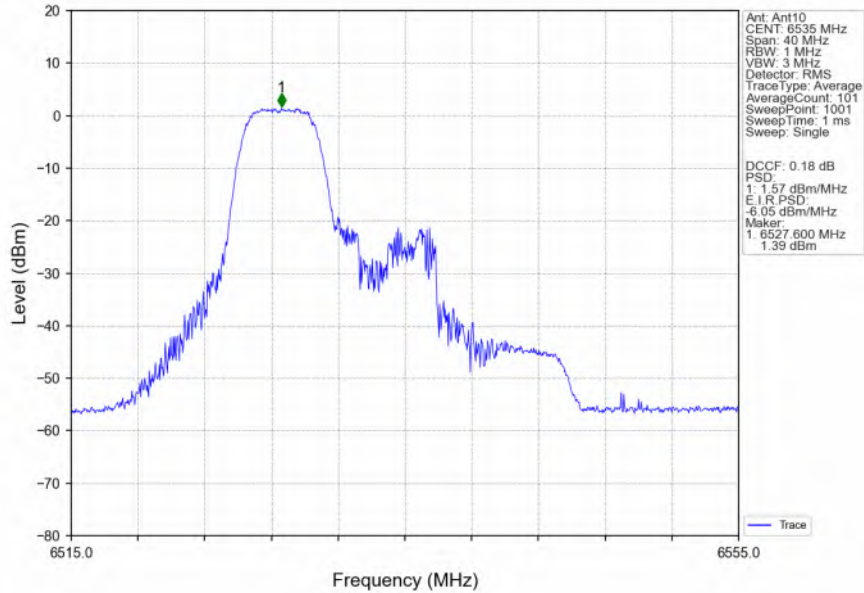
802.11ax(HEW20)_LCH_6535MHz_RU52_Left_MIMO_NTNV
