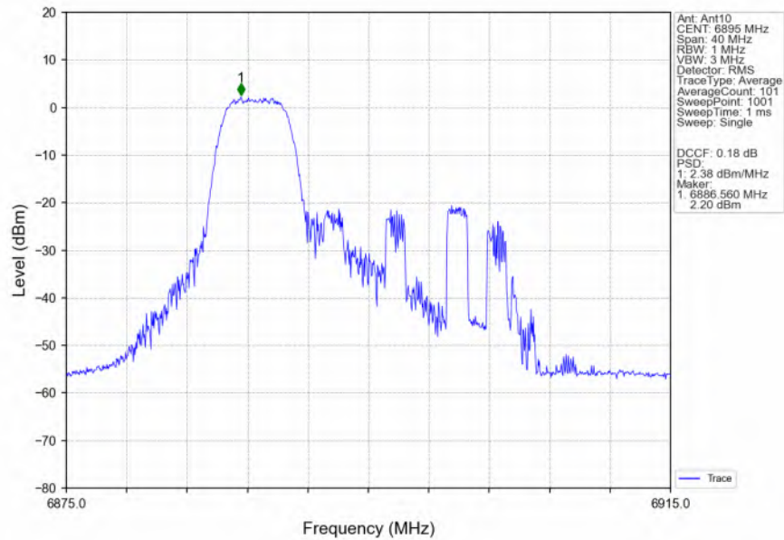
802.11ax(HEW20)_LCH_6895MHz_RU52_Left_MIMO_NTNV
