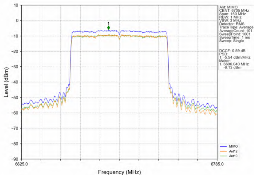
802.11ax(HEW80) MCH_6705MHz RU996 Left_MIMO_NTNV
