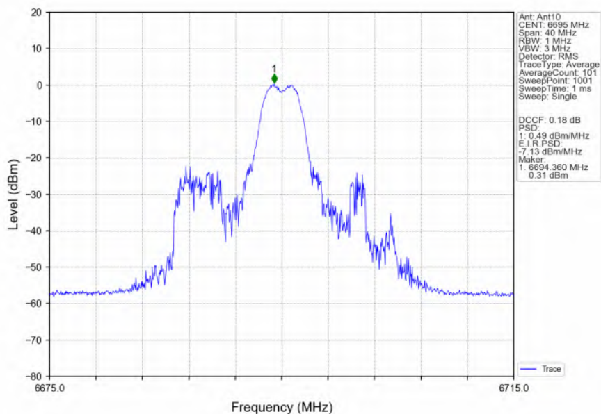
802.11ax(HEW20) MCH 6695MHz RU26 Mid_Ant10 NTN
