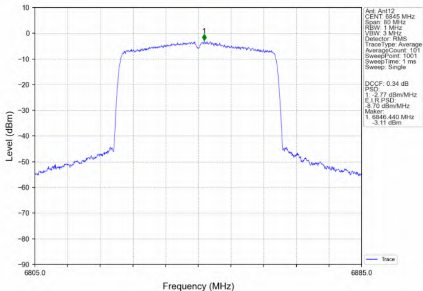
802.11ax(HEW40) HCH 6845MHz RU484 Left Ant12 NTN
