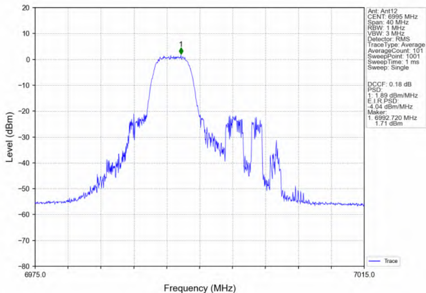
802.11ax(HEW20)_MCH_6995MHz_RU52_Mid_Ant12_NTNV
