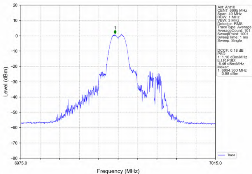
802.11ax(HEW20) MCH 6995MHz RU26 Mid_Ant10 NTN
