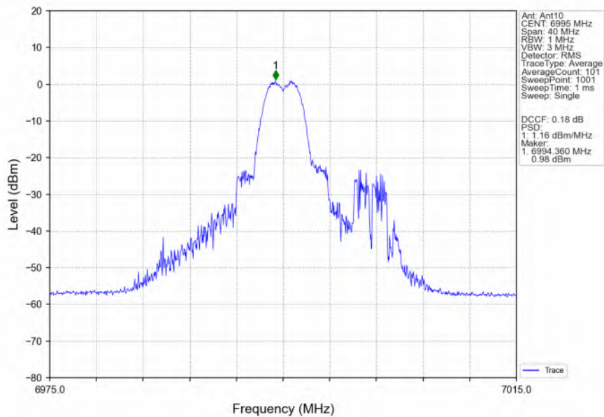
802.11ax(HEW20)_MCH_6995MHz_RU26_Mid_Ant10_NTNV
