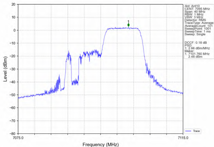
802.11ax(HEW20)_HCH_7095MHz_RU106_Right_Ant10_NTNV
