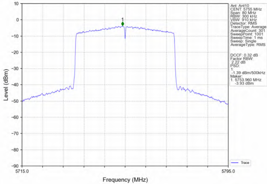
802.11ax(HEW40)_LCH_5755MHz_RU484_Left_MIMO_NTNV
