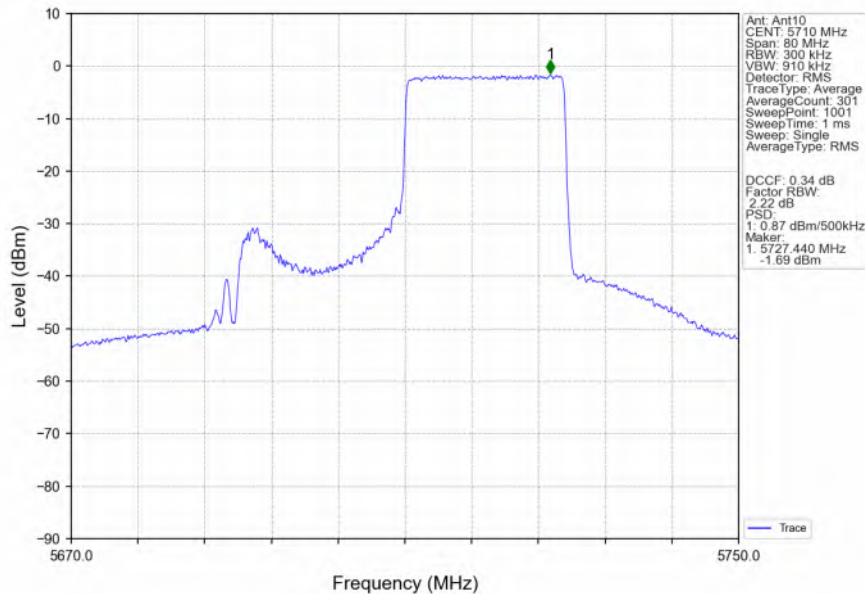
802.11ax(HEW40)_HCH_5710MHz_RU242_Right_Ant10_NTNV
