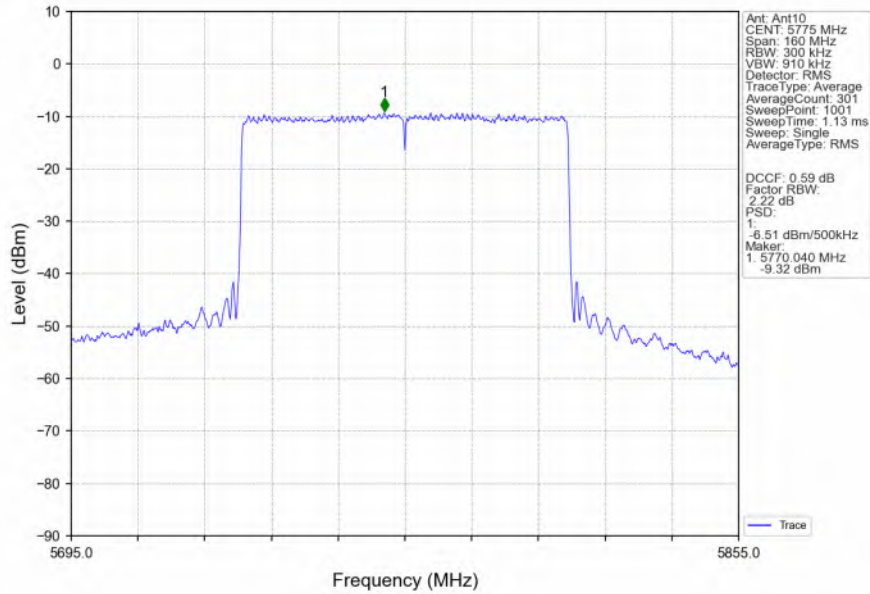
802.11ax(HEW80)_MCH_5775MHz_RU996_Left_MIMO_NTNV
