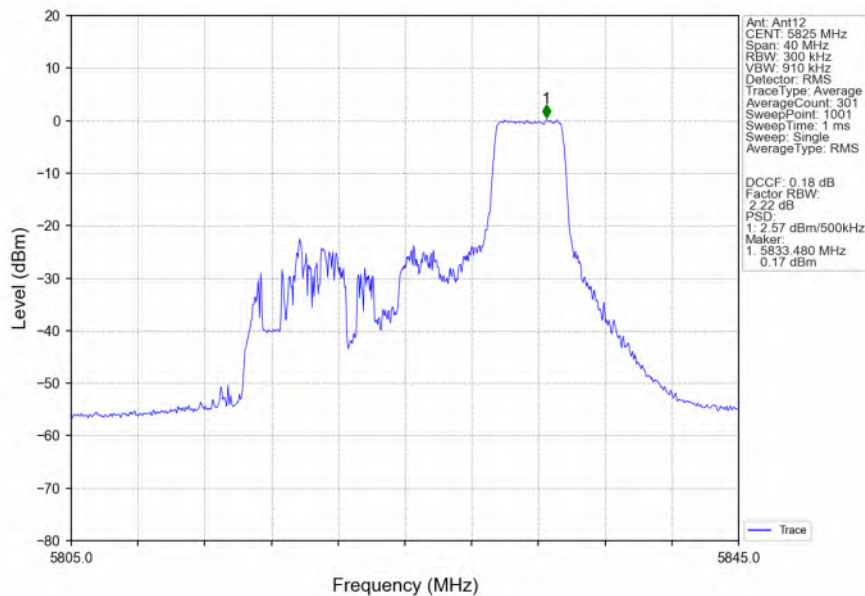
802.11ax(HEW20)_HCH_5825MHz_RU52_Right_Ant12_NTNV
