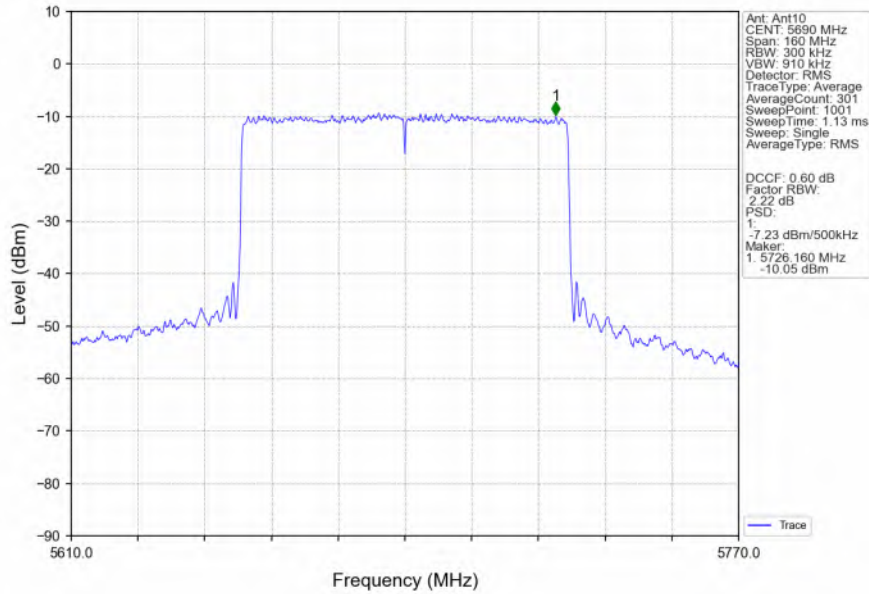
802.11ax(HEW80)_HCH_5690MHz_RU996_Left_MIMO_NTNV
