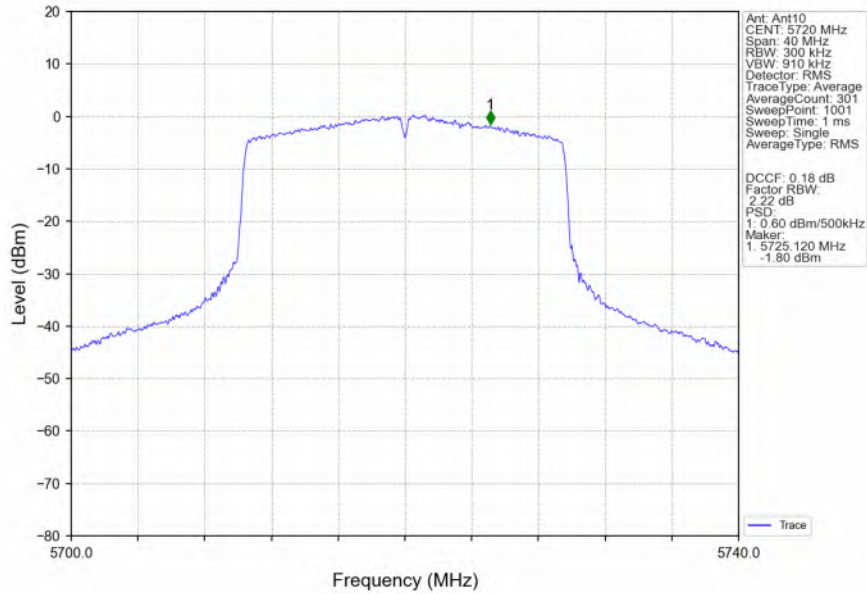
802.11ax(HEW20)_HCH_5720MHz_RU242_Left_MIMO_NTNV
