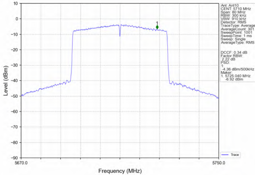
802.11ax(HEW40)_HCH_5710MHz_RU484_Left_MIMO_NTNV
