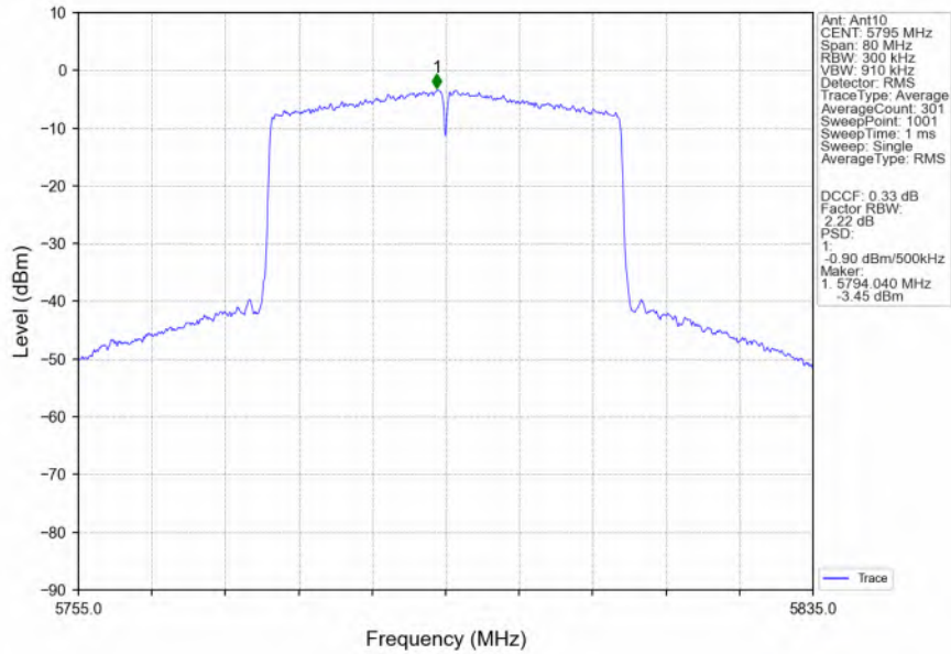
802.11ax(HEW40)_HCH_5795MHz_RU484_Left_MIMO_NTNV
