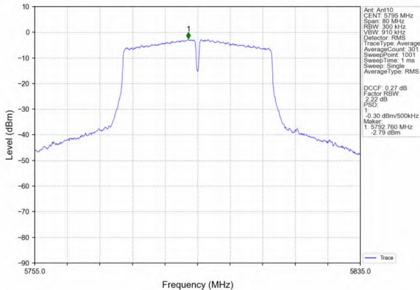
802.11ac(VHT40)_HCH_5795MHz_Ant10_NTNV
