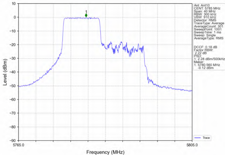
802.11ax(HEW20)_MCH_5785MHz_RU106_Left_Ant10_NTNV
