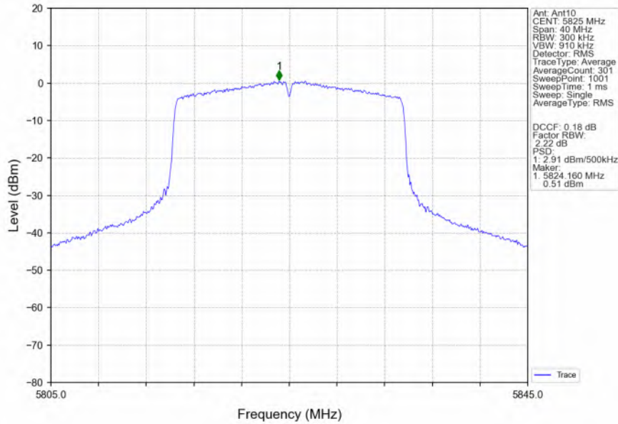
802.11ax(HEW20)_HCH_5825MHz_RU242_Left_MIMO_NTNV
