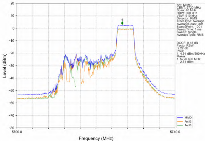
802.11ax(HEW20)_HCH_5720MHz_RU52_Right_MIMO_NTNV
