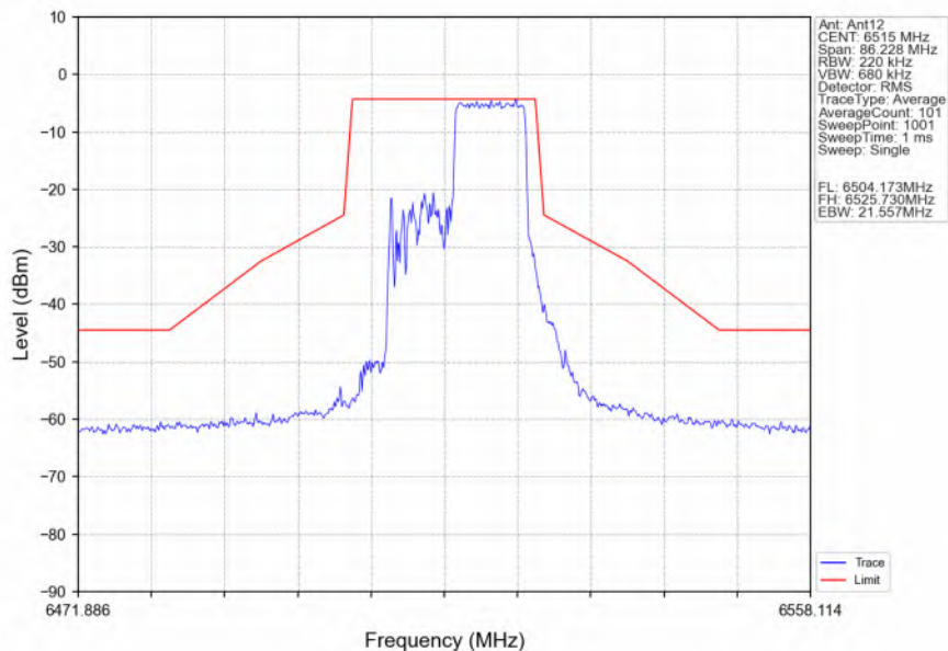
802.11ax(HEW20) HCH 6515MHz RU106 Right Ant12 NTNv
