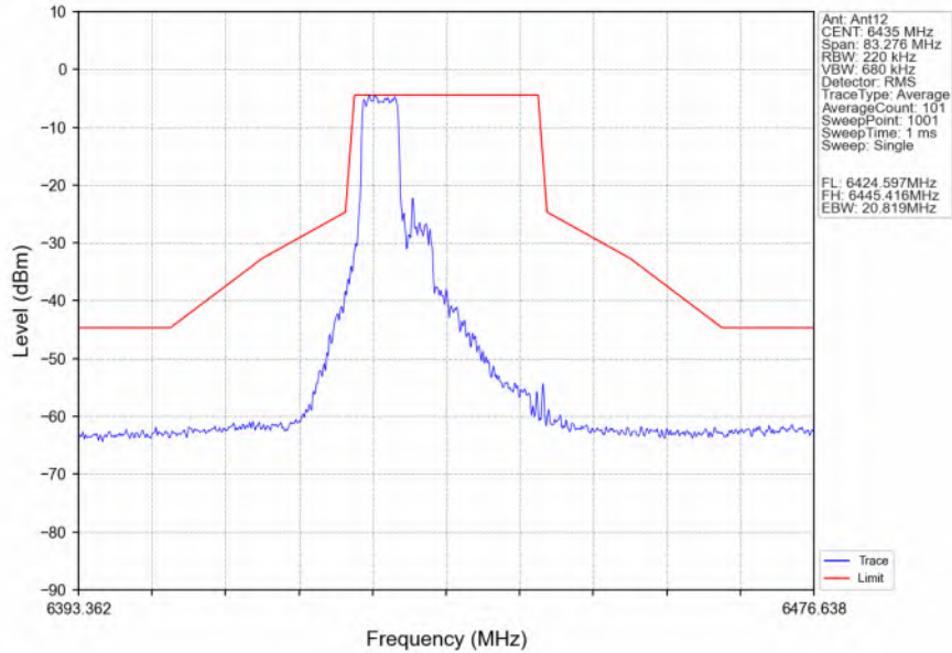
802.11ax(HEW20)_LCH_6435MHz_RU106_Left_Ant12_NTNV
