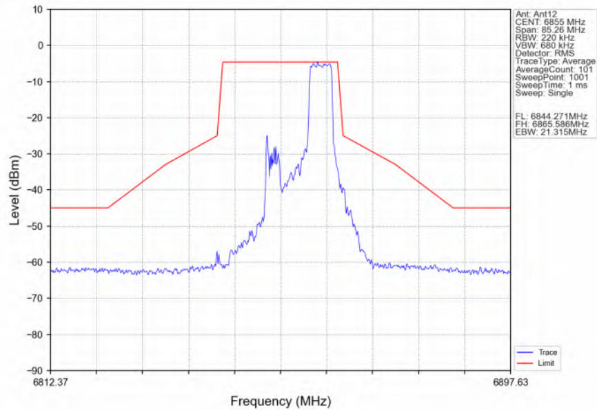
802.11ax(HEW20) HCH 6855MHz RU106 Right Ant12 NTNV
