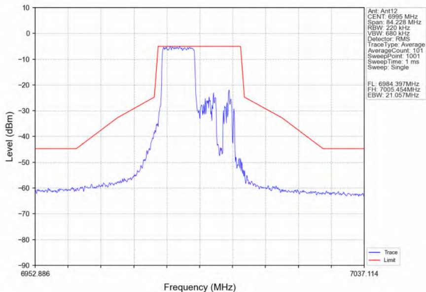
802.11ax(HEW20) MCH 6995MHz RU106 Left_Ant12 NTN
