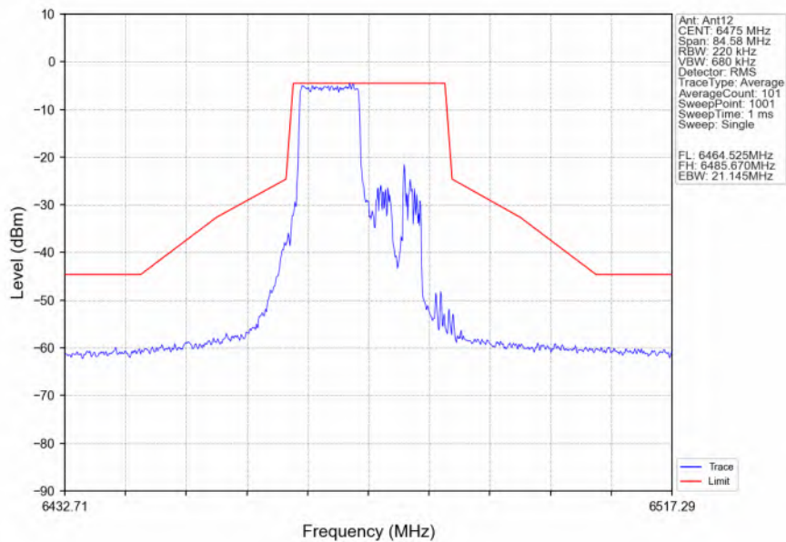
802.11ax(HEW20) MCH 6475MHz RU106 Left_Ant12 NTN
