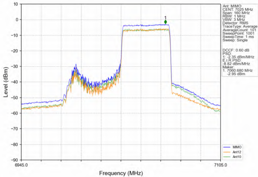
802.11ax(HEW80) HCH 7025MHz RU996 Left Ant12 NTN
