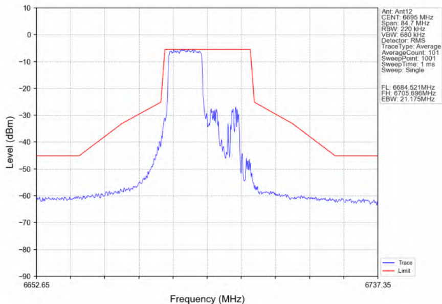
802.11ax(HEW20) MCH 6695MHz RU106 Left_Ant12 NTN
