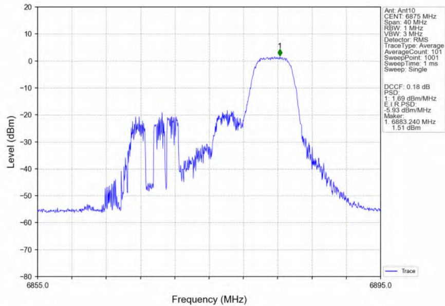
802.11ax(HEW20) HCH 6875MHz RU52 Right MIMO NTN
