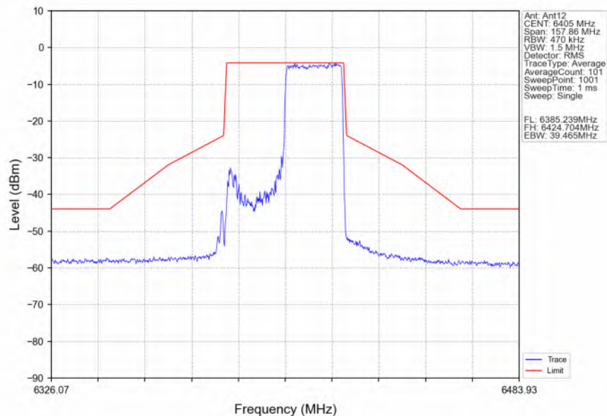
802.11ax(HEW40) HCH 6405MHz RU242 Right Ant12 NTNv
