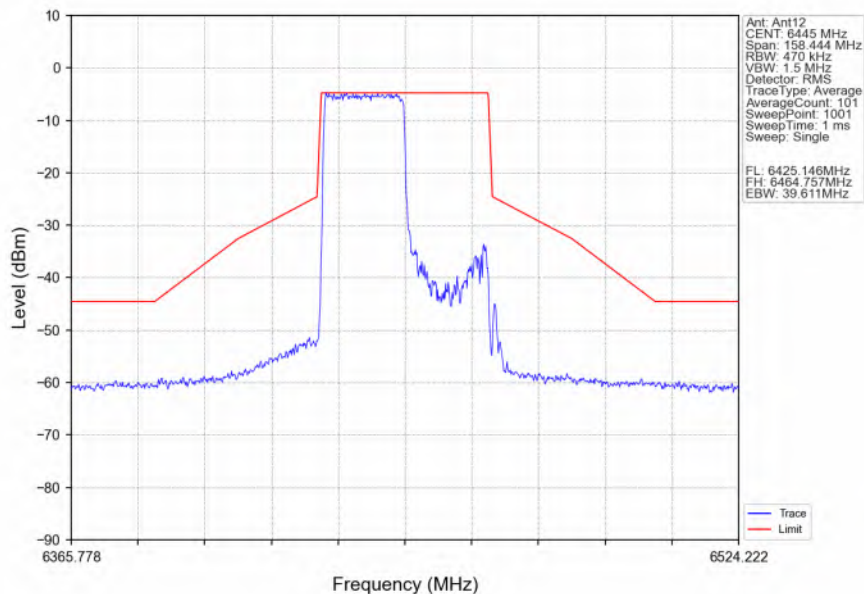
802.11ax(HEW40) LCH 6445MHz RU242 Left Ant12 NTNv
