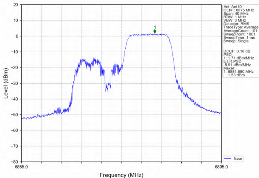
802.11ax(HEW20)_HCH_6875MHz_RU106_Right_Ant10_NTNV
