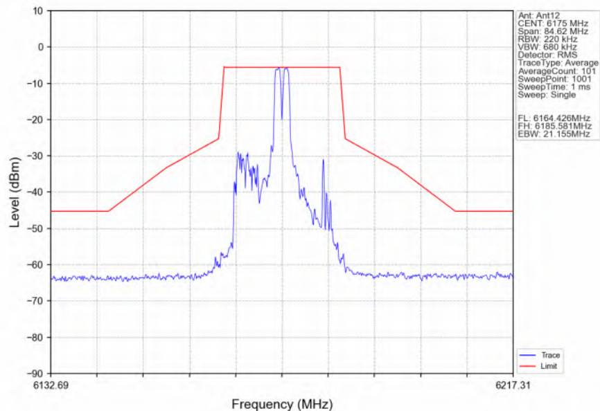
802.11ax(HEW20) MCH 6175MHz RU26 Mid_Ant12 NTN
