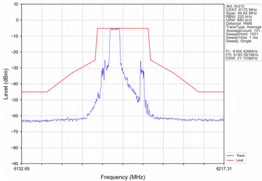
802.11ax(HEW20) MCH 6175MHz RU106 Left_Ant12 NTN
