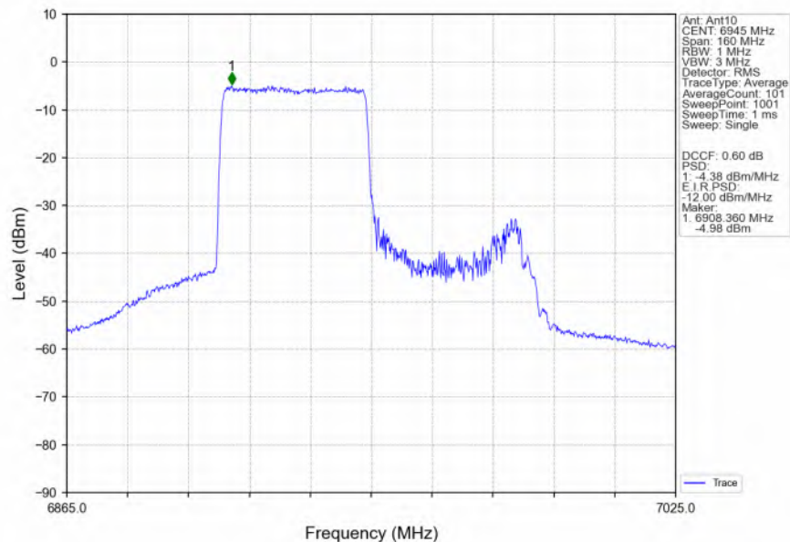
802.11ax(HEW80) LCH 6945MHz RU484 Left_Ant10 NTN
