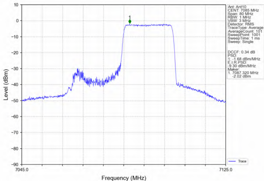
802.11ax(HEW40)_HCH_7085MHz_RU242_Right_Ant10_NTNV
