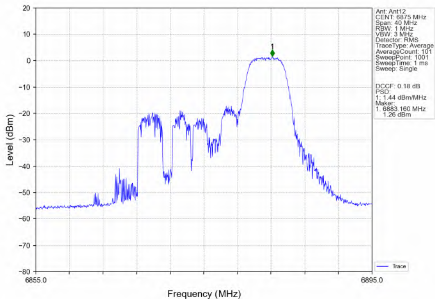
802.11ax(HEW20) HCH 6875MHz RU52 Right Ant12 NTNW
