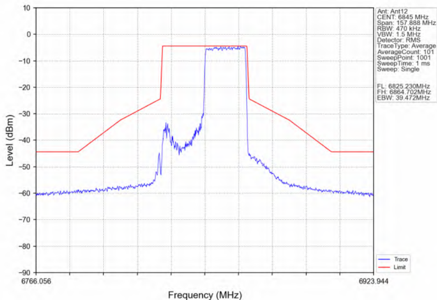
802.11ax(HEW40) HCH_6845MHz RU242 Right_Ant12_NTNV
