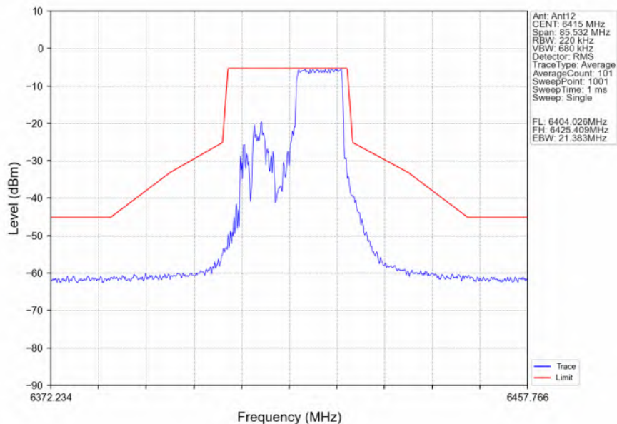
802.11ax(HEW20) HCH 6415MHz RU106 Right Ant12 NTNV
