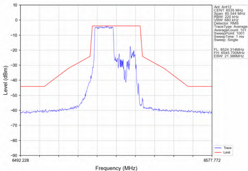
802.11ax(HEW20)_LCH_6535MHz_RU106_Left_Ant12_NTNV
