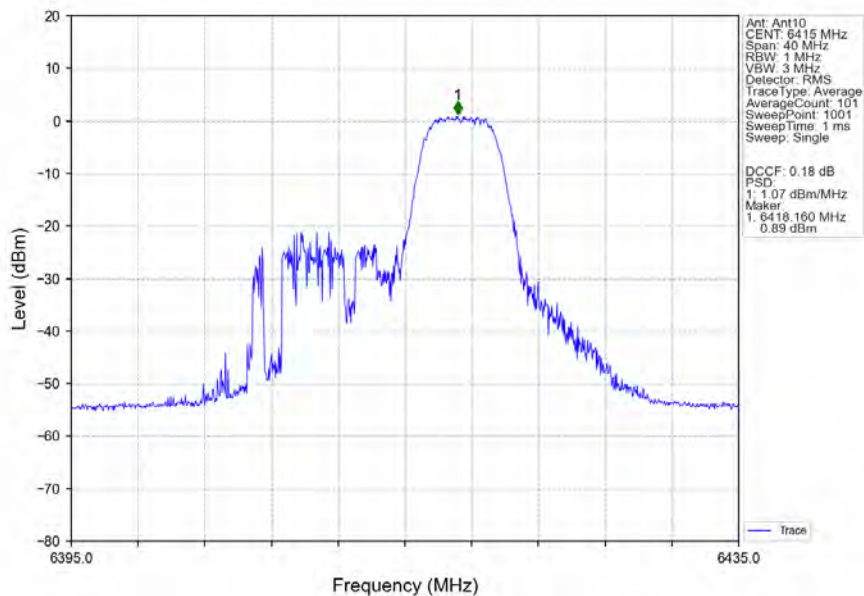
802.11ax(HEW20)_HCH_6415MHz_RU52_Right_Ant10_NTNV
