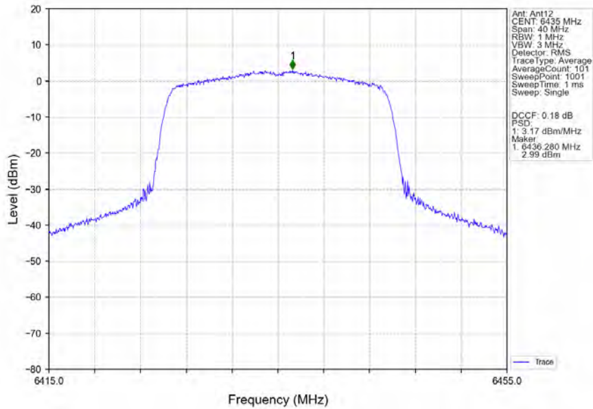
802.11ax(HEW20)_LCH_6435MHz_SU_/_MIMO_NTNV
