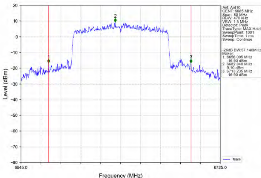
802.11ax(HEW40)_MCH_6685MHz_SU_ / _Ant10_NTNV
