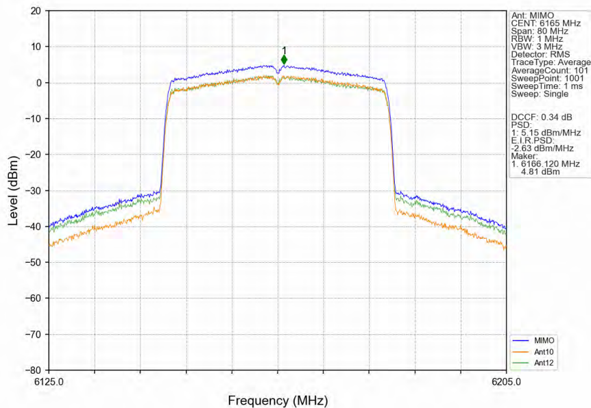
802.11ax(HEW40)_MCH_6165MHz_SU_/_MIMO_NTNV
