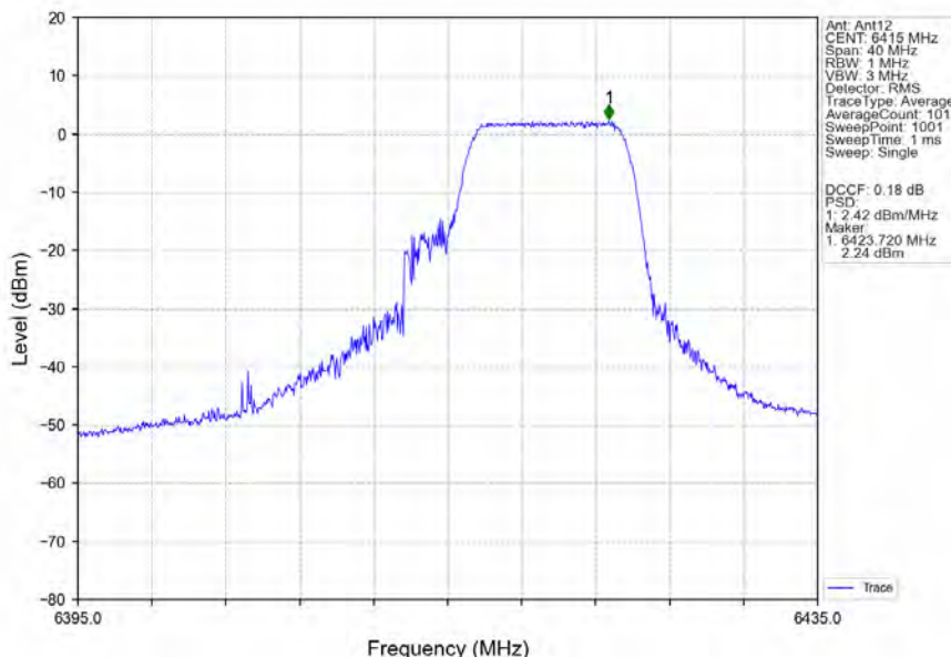
802.11ax(HEW20)_HCH_6415MHz_RU106_Right_Ant12_NTNV
