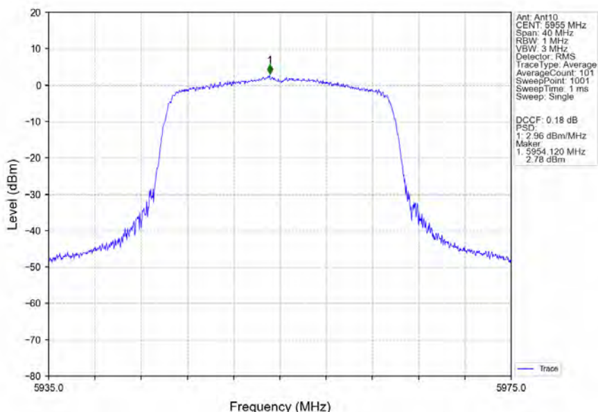
802.11ax(HEW20)_LCH_5955MHz_SU_/_Ant10_NTNV
