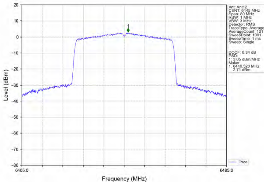
802.11ax(HEW40)_LCH_6445MHz_SU_/_Ant12_NTNV
