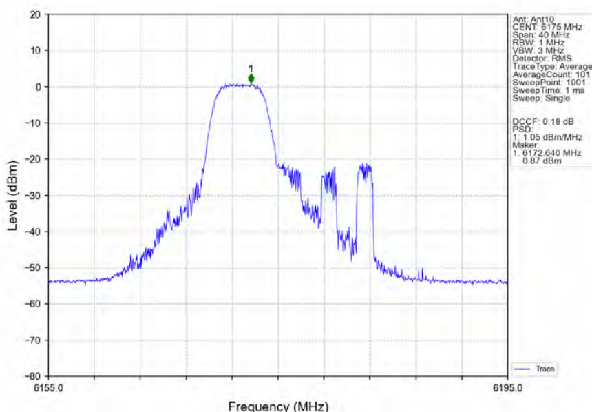
802.11ax(HEW20)_MCH_6175MHz_RU52_Mid_Ant10_NTNV
