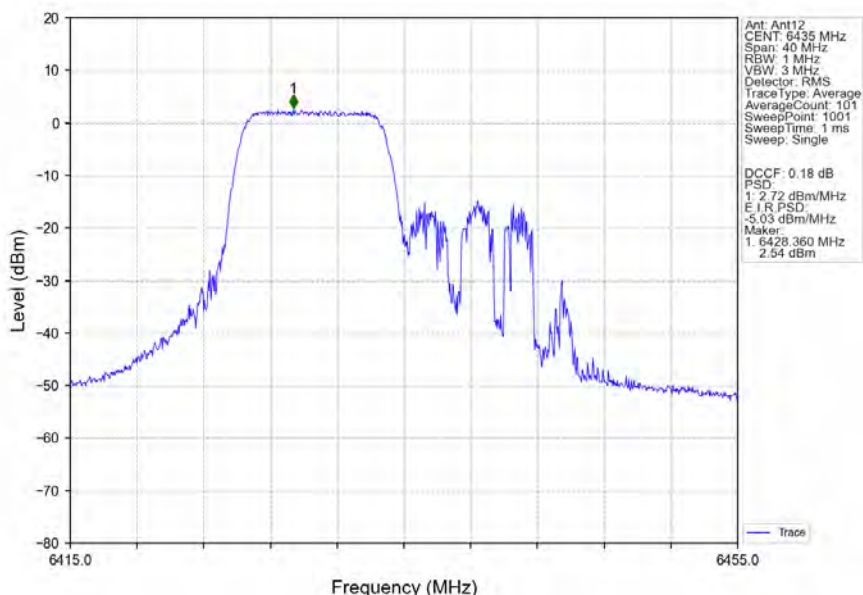
802.11ax(HEW20)_LCH_6435MHz_RU106_Left_Ant12_NTNV
