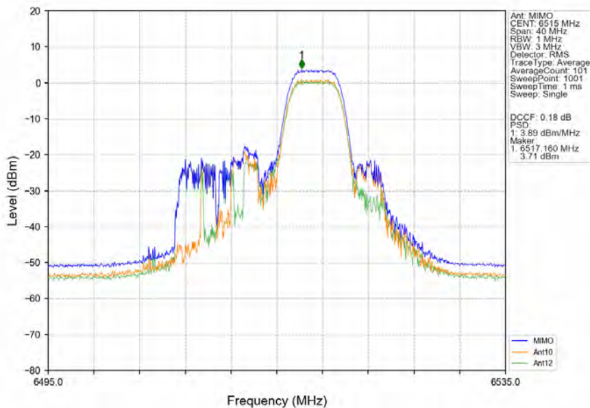
802.11ax(HEW20)_HCH_6515MHz_RU52_Right_MIMO_NTNV
