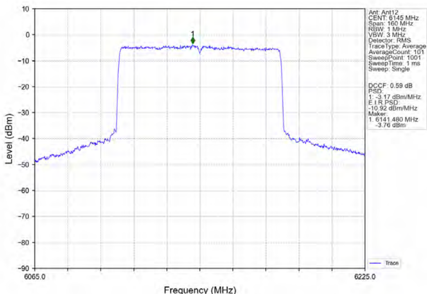
802.11ax(HEW80)_MCH_6145MHz_SU_/_Ant12_NTNV
