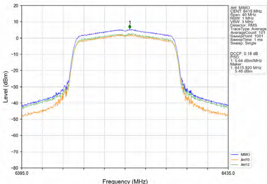
802.11ax(HEW20)_HCH_6415MHz_SU_/_MIMO_NTNV
