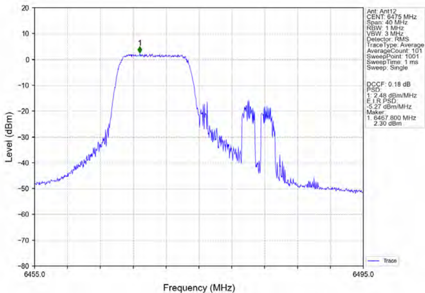
802.11ax(HEW20)_MCH_6475MHz_RU106_Left_Ant12_NTNV
