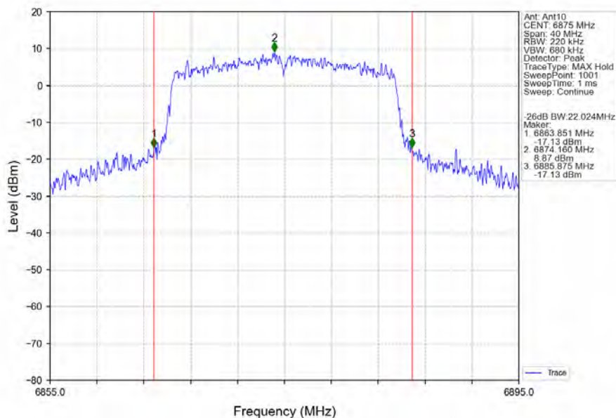
802.11ax(HEW20)_HCH_6875MHz_SU_/_Ant10_NTNV
