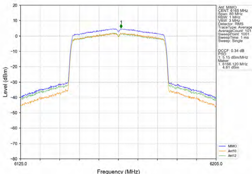
802.11ax(HEW40)_MCH_6165MHz_SU_/_MIMO_NTNV
