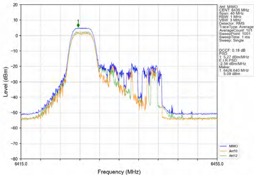
802.11ax(HEW20)_LCH_6435MHz_RU52_Left_MIMO_NTNV
