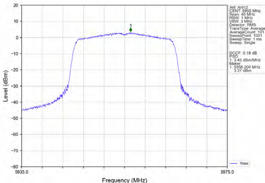
802.11ax(HEW20)_LCH_5955MHz_SU_/_MIMO_NTNV
