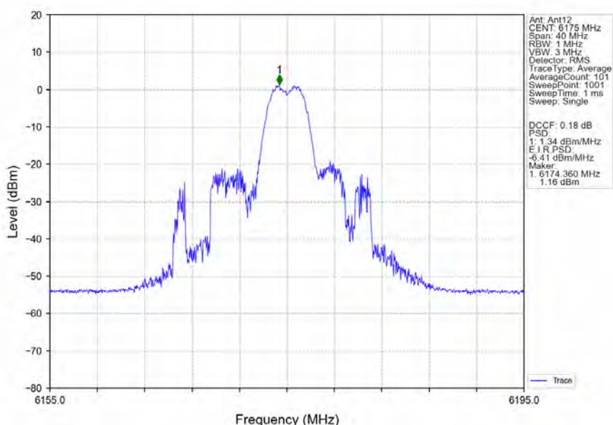
802.11ax(HEW20)_MCH_6175MHz_RU26_Mid_Ant12_NTNV
