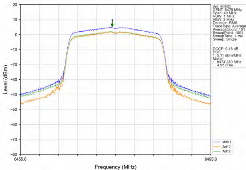
802.11ax(HEW20)_MCH_6475MHz_SU_/_MIMO_NTNV
