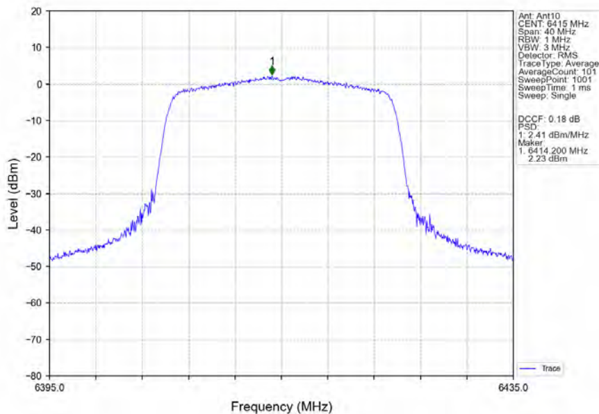
802.11ax(HEW20)_HCH_6415MHz_SU_/_Ant10_NTNV
