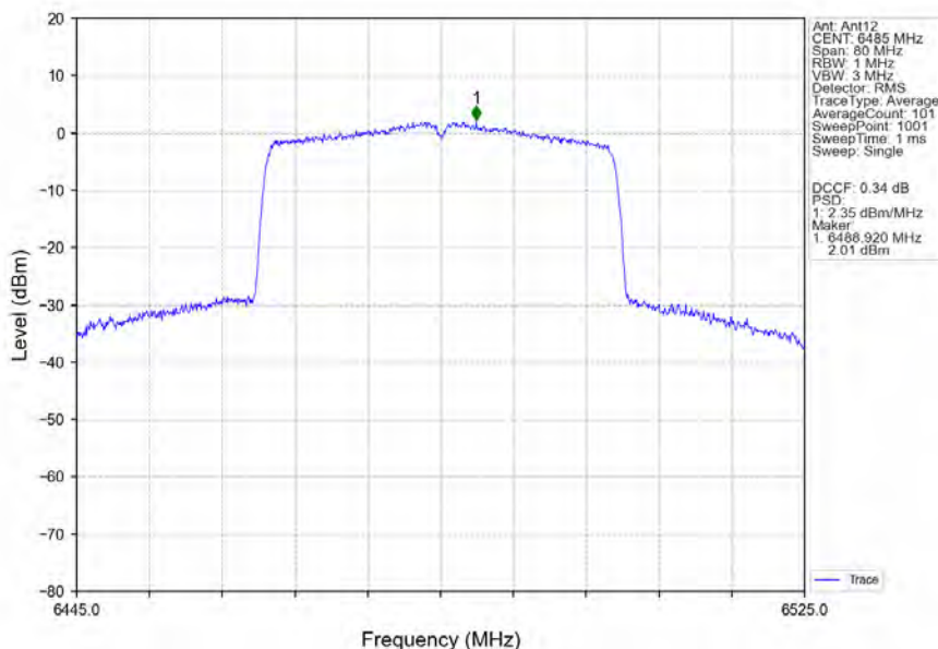
802.11ax(HEW40)_MCH_6485MHz_SU_/_MIMO_NTNV
