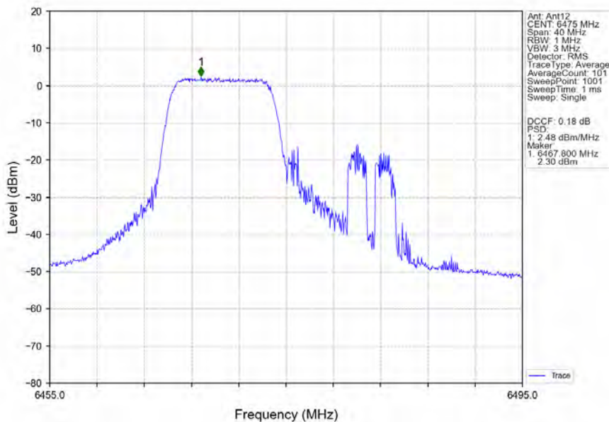
802.11ax(HEW20)_MCH_6475MHz_RU106_Left_Ant12_NTNV
