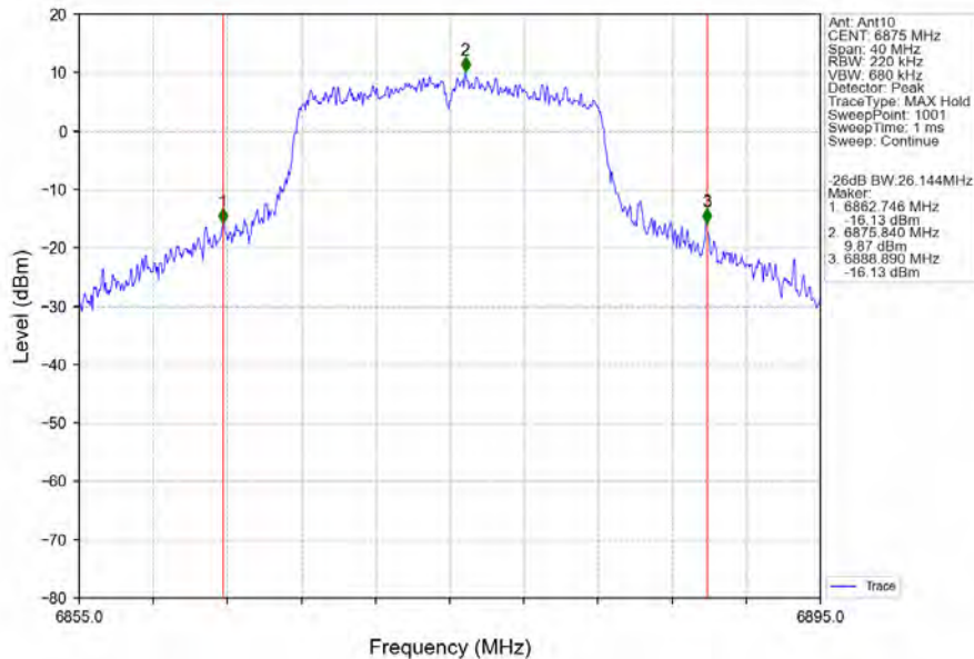
802.11ax(HEW20)_HCH_6875MHz_SU_/_Ant10_NTNV
