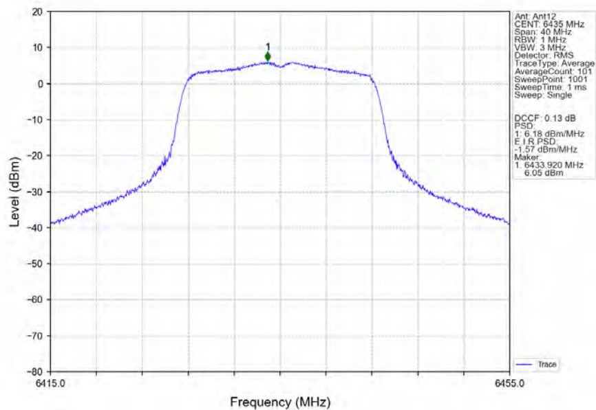
802.11a_LCH_6435MHz_Ant12_NTNV
