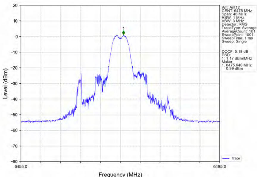
802.11ax(HEW20)_MCH_6475MHz_RU26_Mid_Ant12_NTNV
