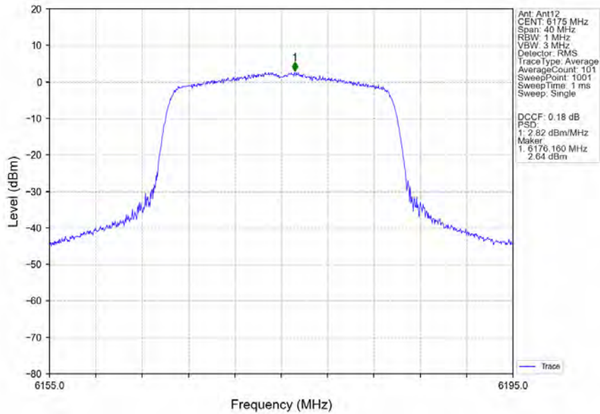
802.11ax(HEW20)_MCH_6175MHz_SU_/_MIMO_NTNV
