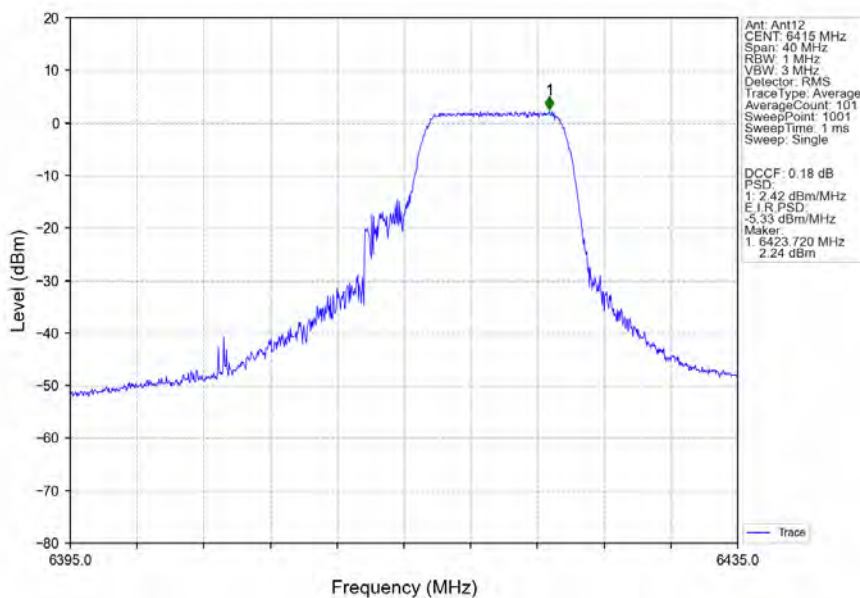
802.11ax(HEW20)_HCH_6415MHz_RU106_Right_Ant12_NTNV
