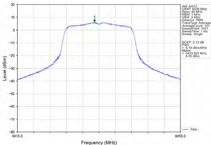
802.11a_LCH_6435MHz_Ant12_NTNV
