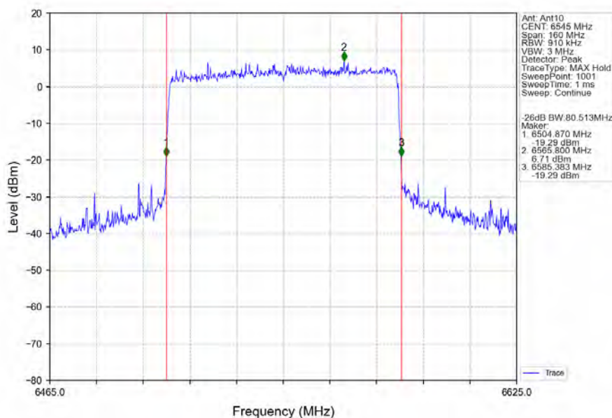
802.11ax(HEW80)_HCH_6545MHz_SU_/_Ant10_NTNV
