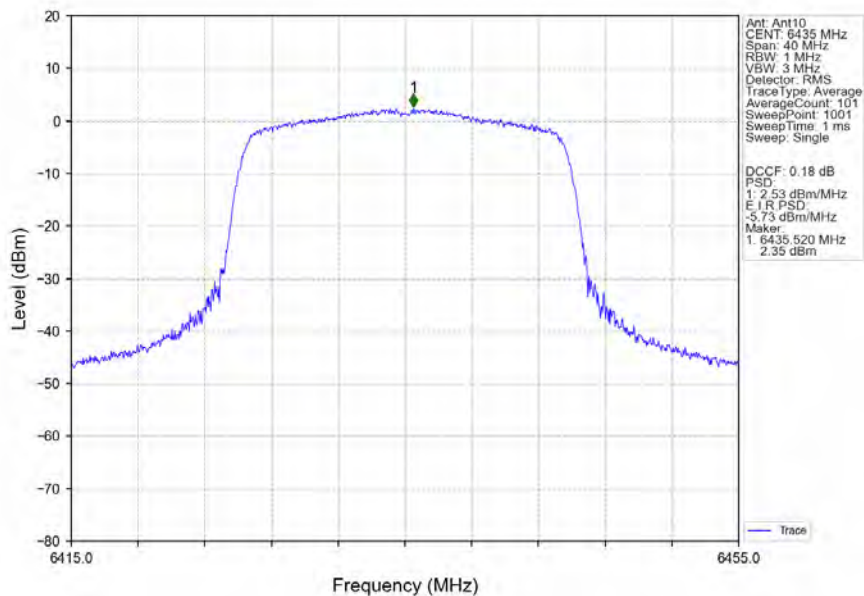
802.11ax(HEW20)_LCH_6435MHz_SU_/_Ant10_NTNV
