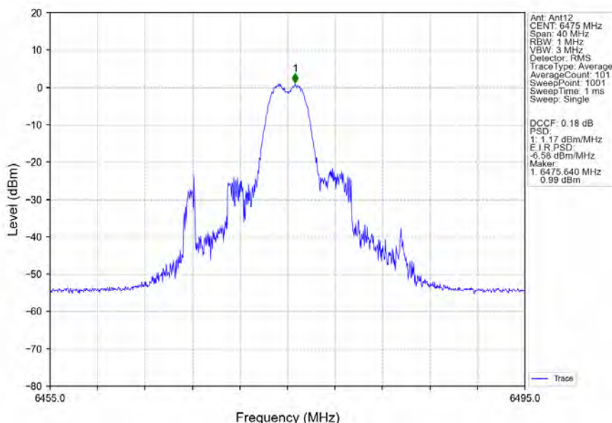
802.11ax(HEW20)_MCH_6475MHz_RU26_Mid_Ant12_NTNV
