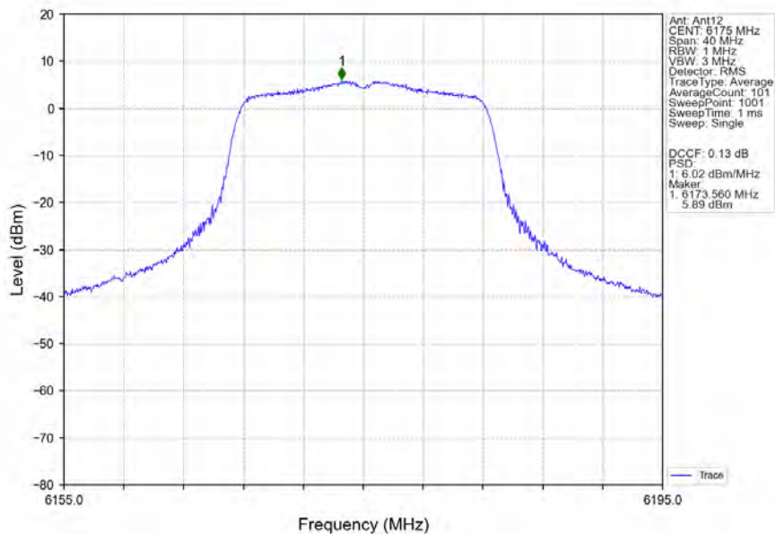
802.11a_MCH_6175MHz_Ant12_NTNV
