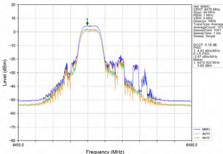
802.11ax(HEW20)_MCH_6475MHz_RU52_Mid_MIMO_NTNV
