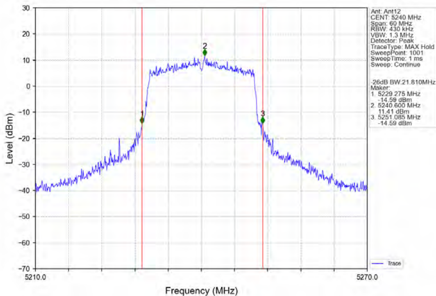
802.11ax(HEW20)_HCH_5240MHz_RU242_Left_Ant12_NTNV
