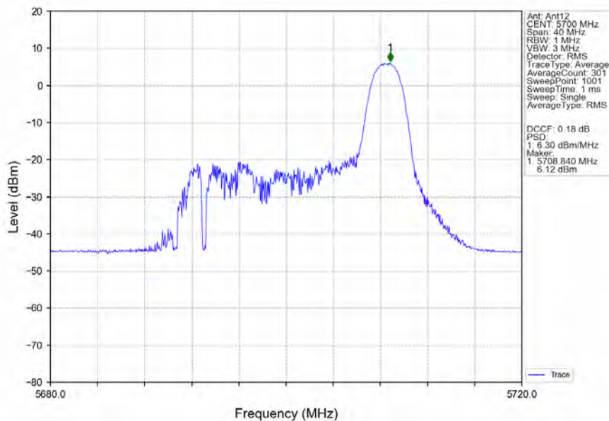
802.11ax(HEW20)_HCH_5700MHz_RU26_Right_Ant12_NTNV
