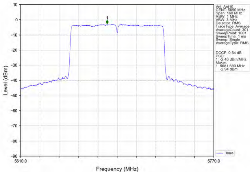
802.11ac(VHT80)_HCH_5690MHz_Ant10_NTNV
