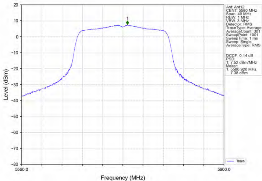
802.11ac(VHT20)_MCH_5580MHz_Ant12_NTNV
