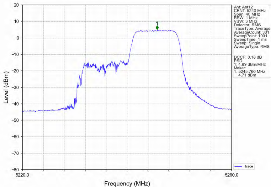
802.11ax(HEW20)_HCH_5240MHz_RU106_Right_Ant12_NTNV
