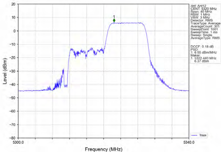
802.11ax(HEW20)_HCH_5320MHz_RU106_Right_Ant12_NTNV
