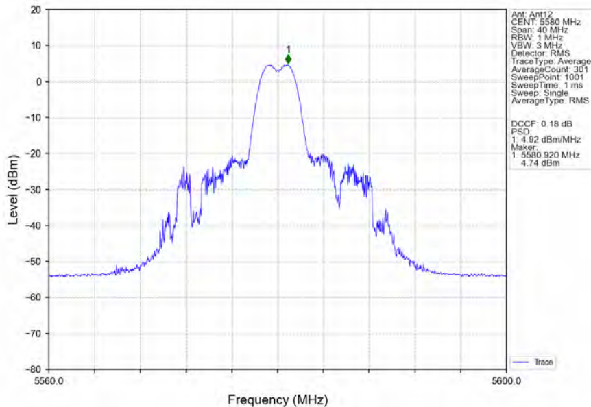
802.11ax(HEW20)_MCH_5580MHz_RU26_Mid_Ant12_NTNV
