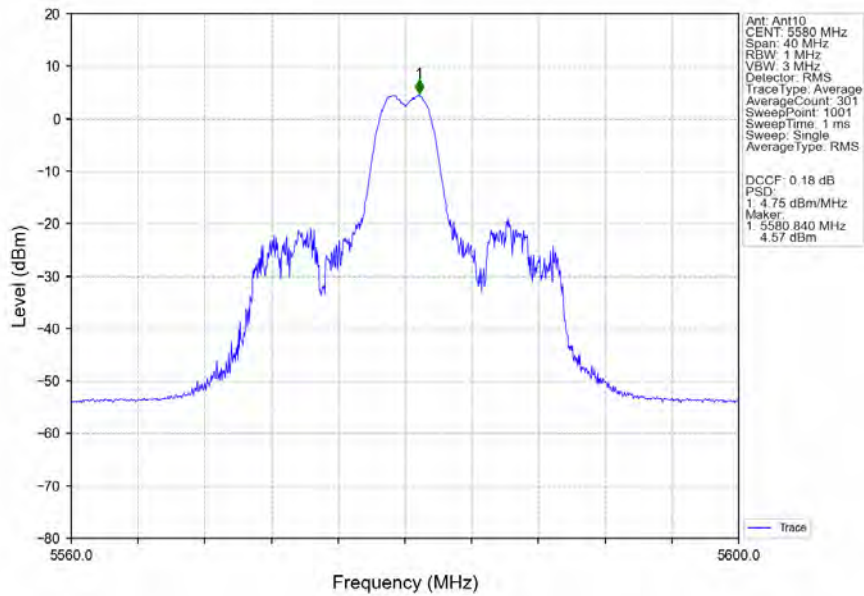
802.11ax(HEW20)_MCH_5580MHz_RU26_Mid_MIMO_NTNV
