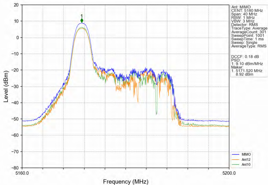
802.11ax(HEW20)_LCH_5180MHz_RU26_Left_MIMO_NTNV
