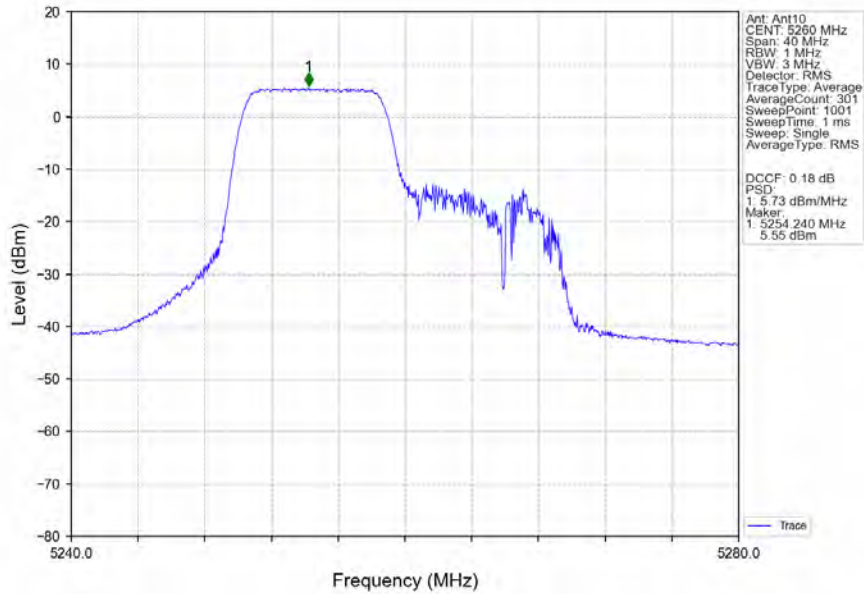
802.11ax(HEW20)_LCH_5260MHz_RU106_Left_MIMO_NTNV
