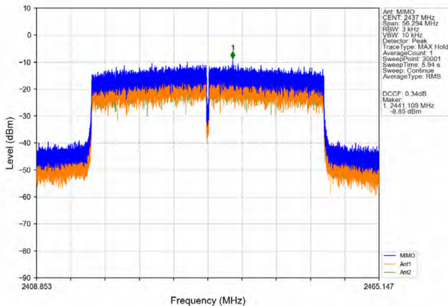
802.11ax(HEW40)_MCH_2437MHz_RU484_Left_MIMO_NTNV
