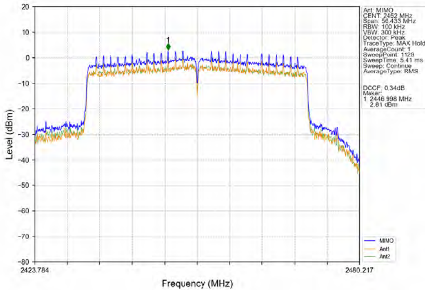
802.11ax(HEW40)_HCH_2452MHz_RU484_Left_MIMO_NTNV
