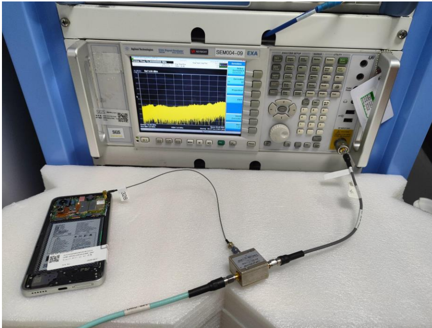
Test Setup Photo for RF conducted:
