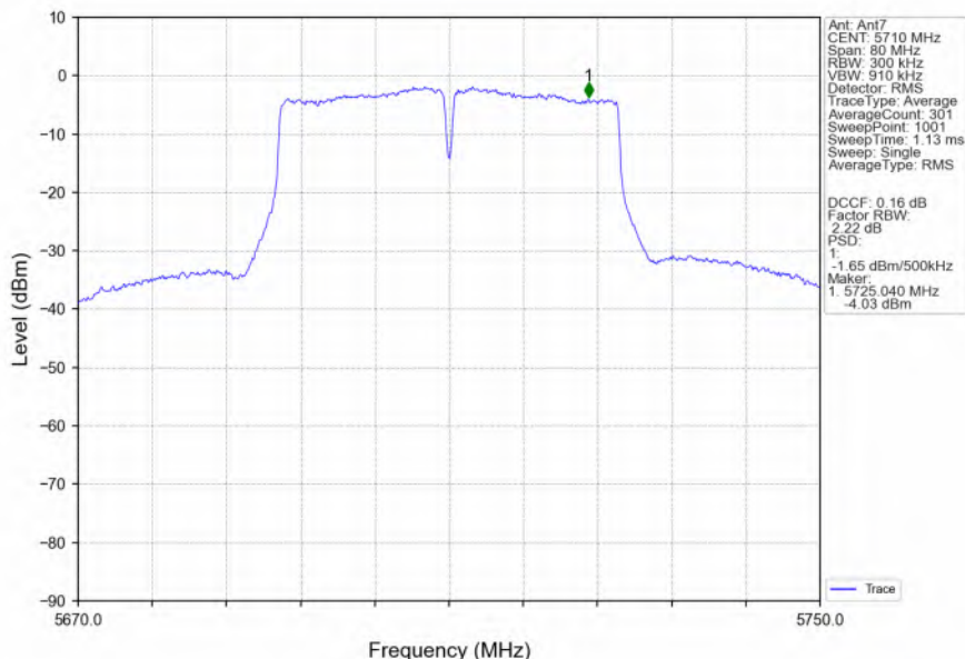
802.11ac(VHT40)_HCH_5710MHz_Ant7_NTNV
