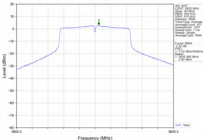
802.11ac(VHT20)_HCH_5825MHz_Ant7_NTNV
