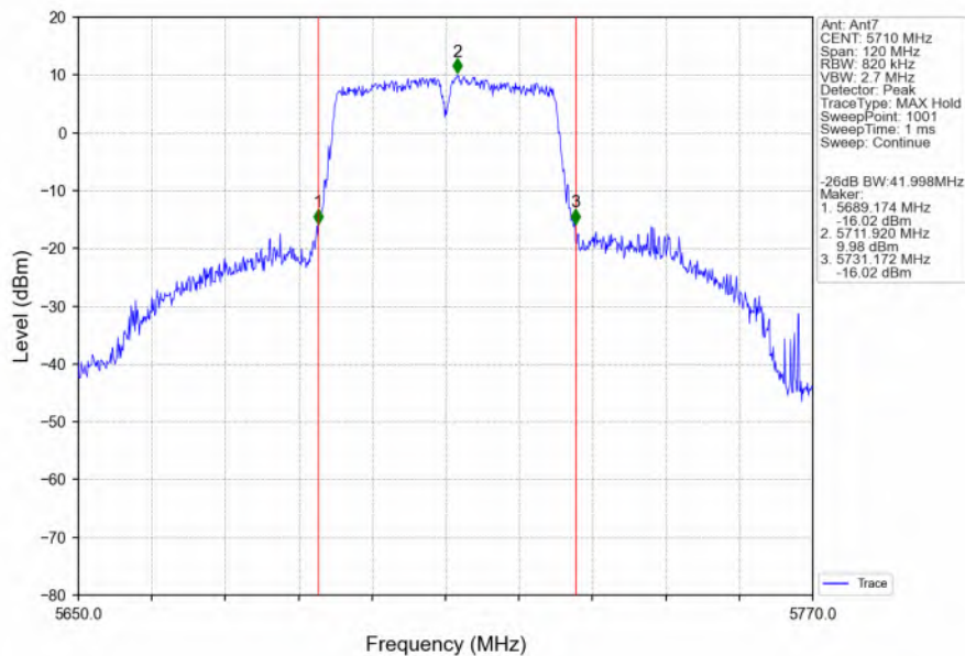
802.11ac(VHT40)_HCH_5710MHz_Ant7_NTNV
