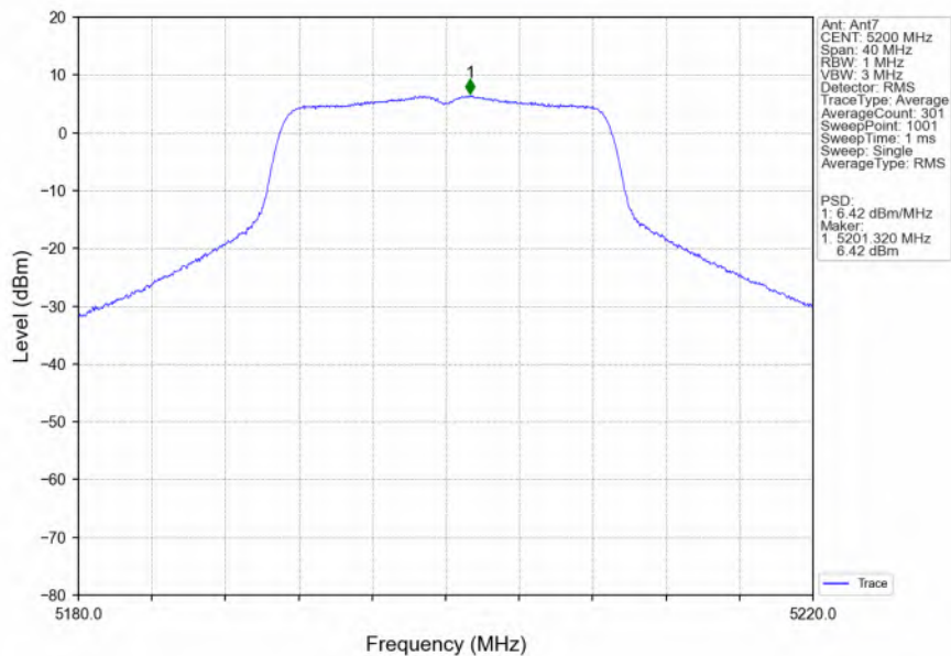
802.11n(HT20)_MCH_5200MHz_Ant7_NTNV
