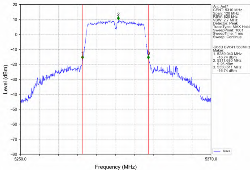
802.11ac(VHT40)_HCH_5310MHz_Ant7_NTNV
