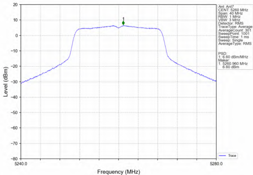
802.11ac(VHT20)_LCH_5260MHz_Ant7_NTNV
