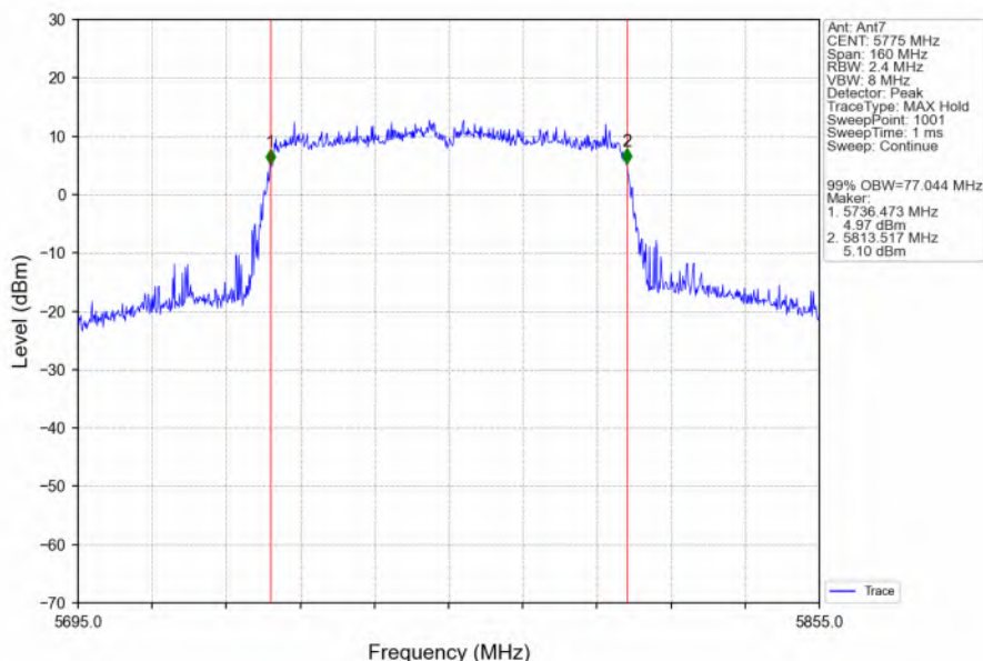
802.11ac(VHT80)_MCH_5775MHz_Ant7_NTNV
