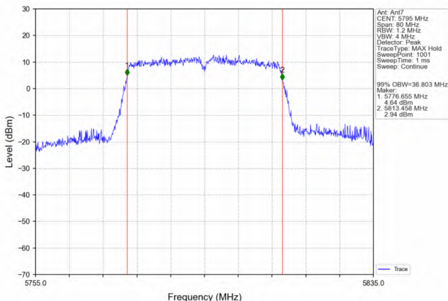
802.11ac(VHT40)_HCH_5795MHz_Ant7_NTNV
