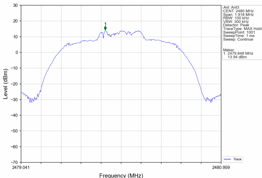
Pi/4DQPSK_2DH5_HCH_2480MHz_Ant3_NTNV
