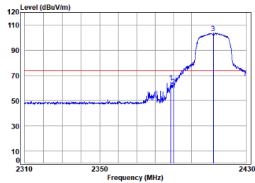
11n_HT(20M)_TX_CH_01_Horizontal-Peak
