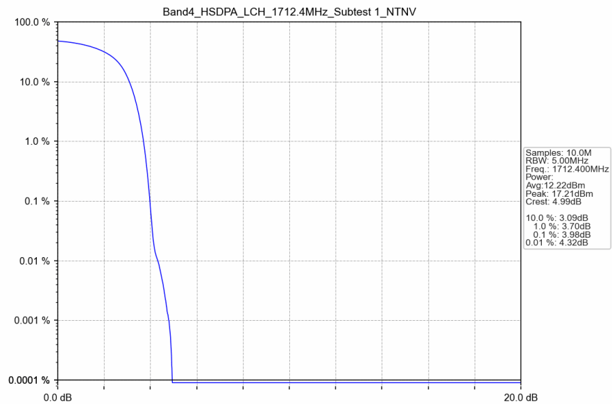
Band4_HSDPA_LCH_1712.4MHz_Subtest 1_NTNV
