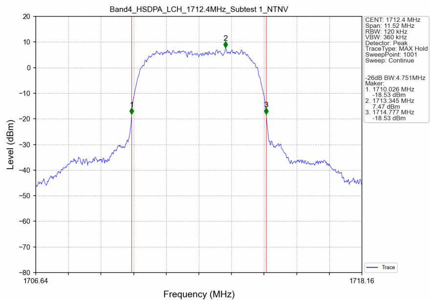
Band4_HSDPA_LCH_1712.4MHz_Subtest 1_NTNV
