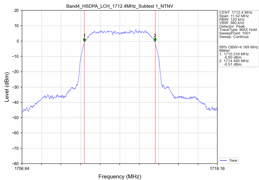
Band4_HSDPA_LCH_1712.4MHz_Subtest 1_NTNV
