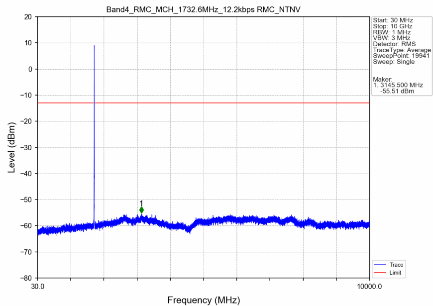
Band4_RMC_MCH_1732.6MHz_12.2kbps RMC_NTNV
