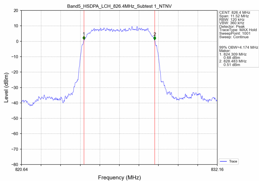
Band5_HSDPA_LCH_826.4MHz_Subtest 1_NTNV
