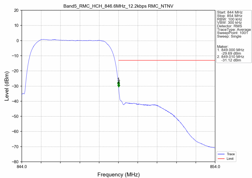
Band5_RMC_HCH_846.6MHz_12.2kbps RMC_NTNV
