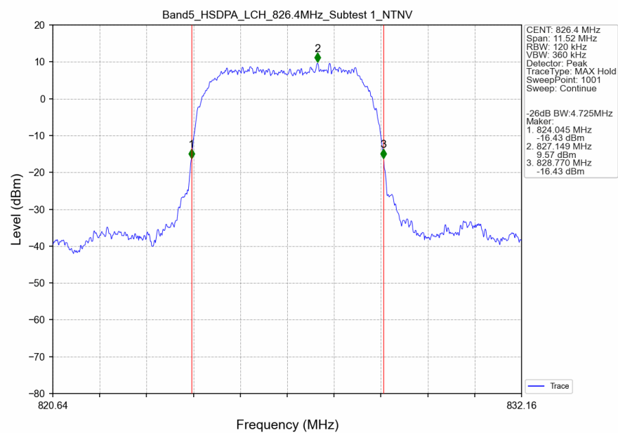
Band5_HSDPA_LCH_826.4MHz_Subtest 1_NTNV
