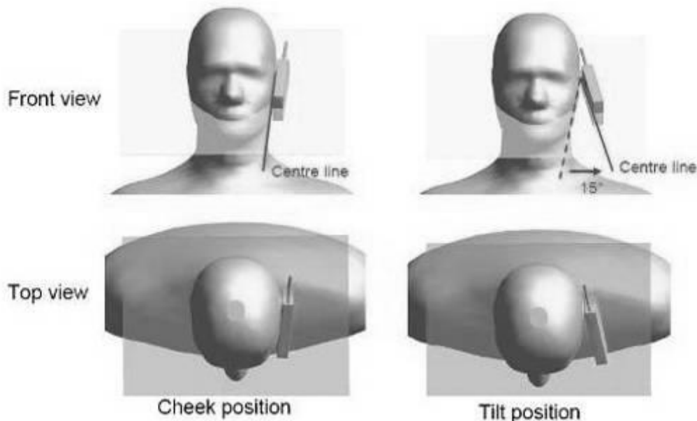
F-9. Definition of the reference lines and points, on the phone and on the phantom and initial position
