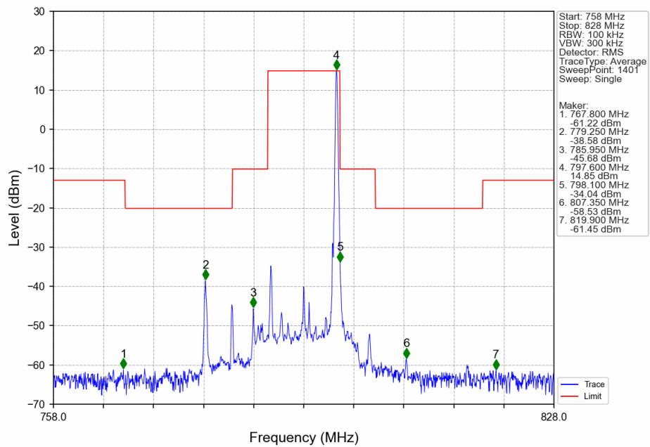
n14_15kHz_SISO_NTNV_10MHz_CP-OFDM_256_QAM_793MHz_Edge_1RB_Right_Ant0
