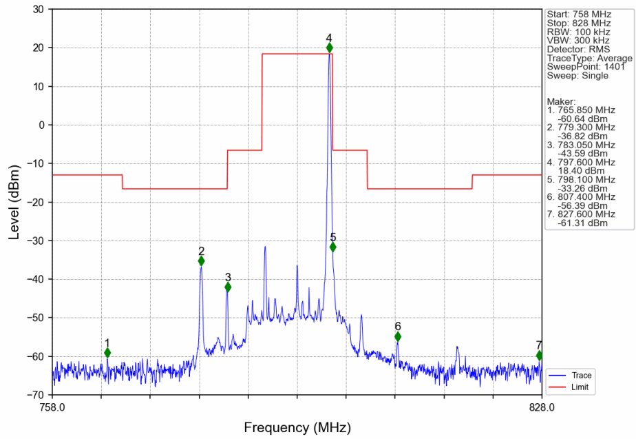
n14_15kHz_SISO_NTNV_10MHz_CP-OFDM 64 QAM_793MHz_Edge_1RB_Right_Ant0
