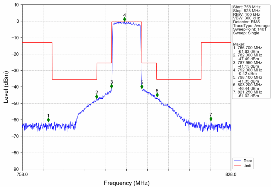
n14_15kHz_SISO_NTNV_10MHz_CP-OFDM 256 QAM_793MHz_Outer_Full_Ant0
