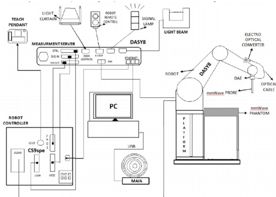
Fig. 1. The SPEAG Robotic Diagram
