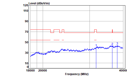
11ac_80M_Straddle_TX_CH_138_Horizontal
