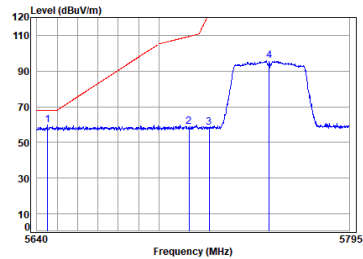
11ac_VHT(40M)_TX_CH_151_Vertical
