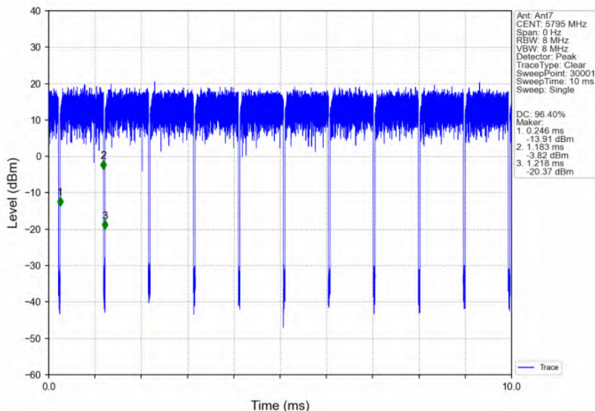
802.11ac(VHT40)_HCH_5795MHz_Ant7_NTNV
