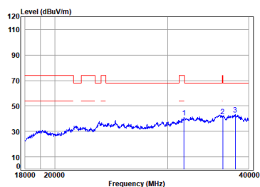
11a_TX_CH_52_Vertical.gif
