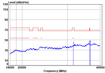
11ac_40M_Straddle_TX_CH_142_Vertical
