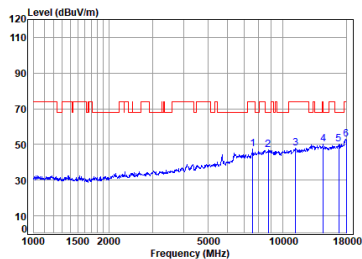
11ac_80M_Straddle_TX_CH_138_Horizontal-Peak
