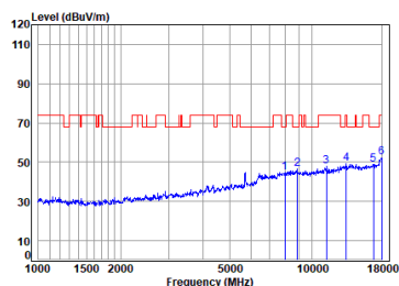
11ac_40M_Straddle_TX_CH_142_Horizontal-Peak
