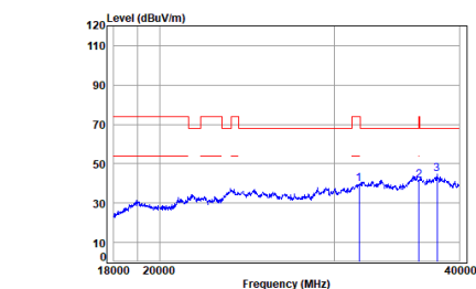
11a_TX_CH_64_Horizontal.gif
