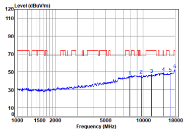
11a_TX_CH_165_Vertical-Peak
