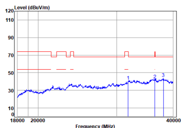
11a_TX_CH_48_Vertical.gif
