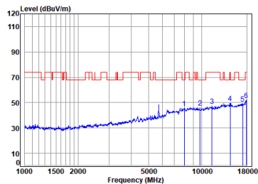
11a_Straddle_TX_CH_144_Horizontal-Peak
