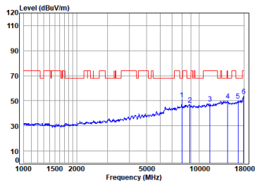
11ac_80M_Straddle_TX_CH_138_Vertical-Peak
