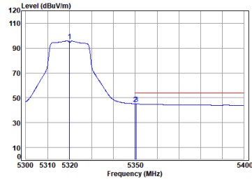
11ac_VHT(20M)_TX_CH_64_Horizontal-Avg
