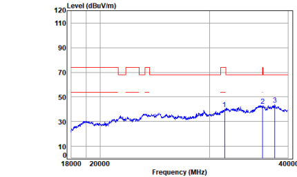
11ac_40M_Straddle_TX_CH_142_Horizontal
