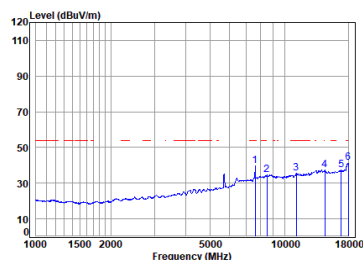
11ac_40M_Straddle_TX_CH_142_Horizontal-Avg
