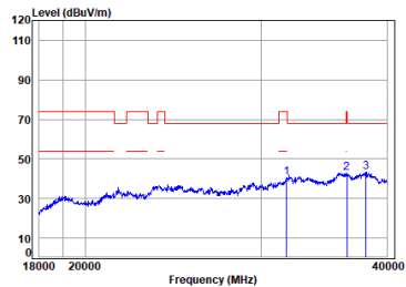
11ac_80M_Straddle_TX_CH_138_Vertical
