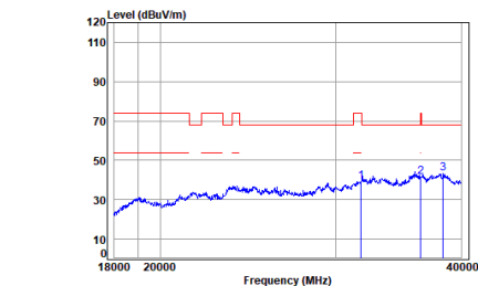
11a_TX_CH_100_Horizontal
