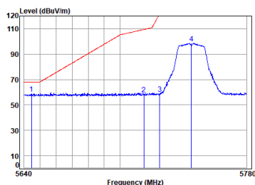
11ac_VHT(20M)_TX_CH_149_Vertical
