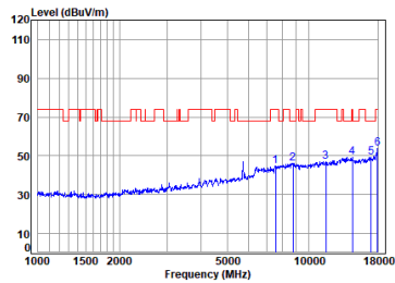
11a_Straddle_TX_CH_144_Vertical-Peak
