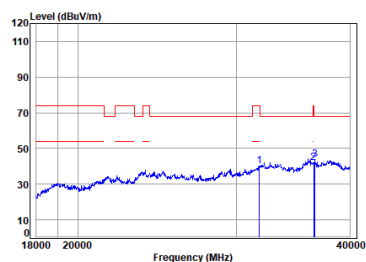
11a_TX_CH_64_Vertical.gif
