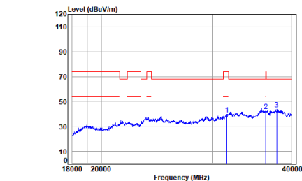
11a_TX_CH_149_Horizontal
