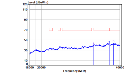
11a_TX_CH_140_Horizontal
