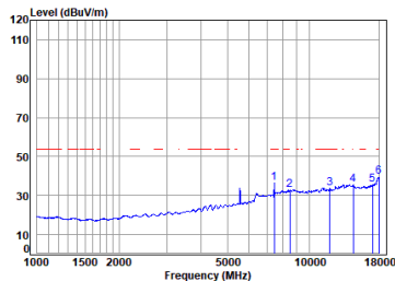
11a_TX_CH_116_Vertical-Avg
