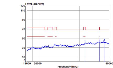
11a_TX_CH_60_Horizontal.gif
