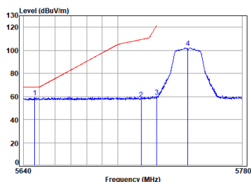
11ac_VHT(20M)_TX_CH_149_Horizontal
