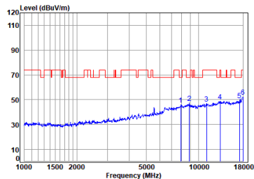
11a_TX_CH_116_Vertical-Peak
