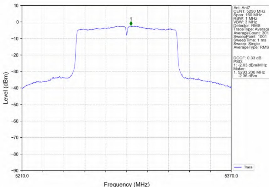
802.11ac(VHT80)_MCH_5290MHz_Ant7_NTNV
