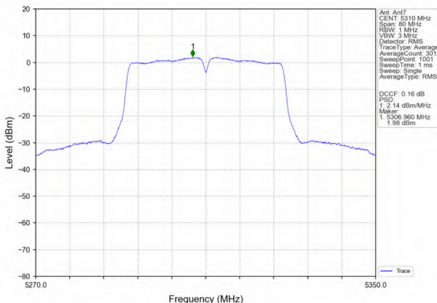
802.11ac(VHT40)_HCH_5310MHz_Ant7_NTNV
