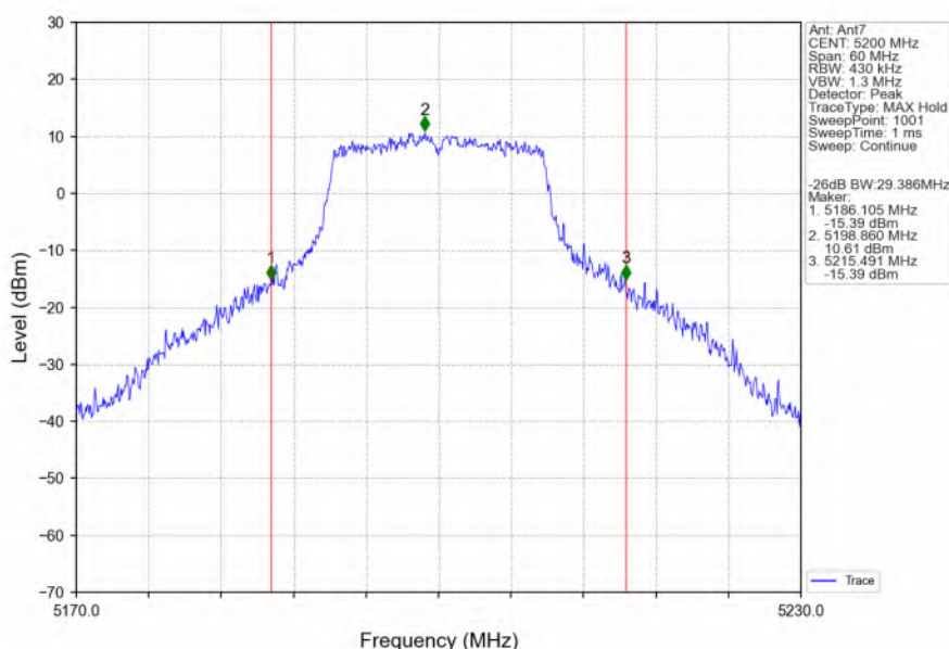
802.11ac(VHT20)_MCH_5200MHz_Ant7_NTNV
