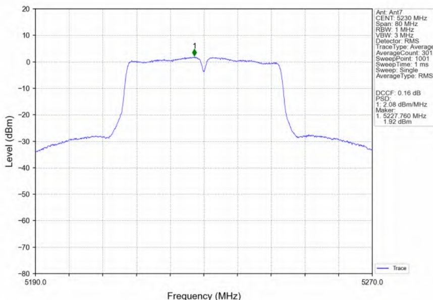
802.11ac(VHT40)_HCH_5230MHz_Ant7_NTNV
