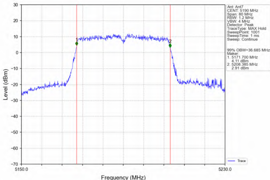
802.11ac(VHT40)_LCH_5190MHz_Ant7_NTNV
