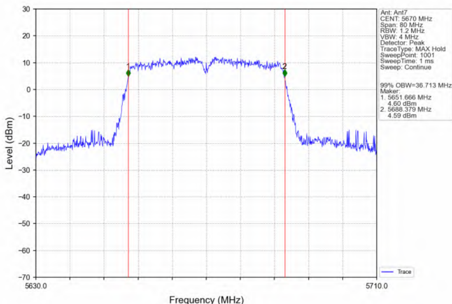
802.11ac(VHT40)_HCH_5670MHz_Ant7_NTNV
