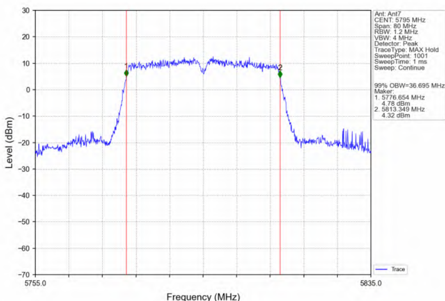
802.11ac(VHT40)_HCH_5795MHz_Ant7_NTNV
