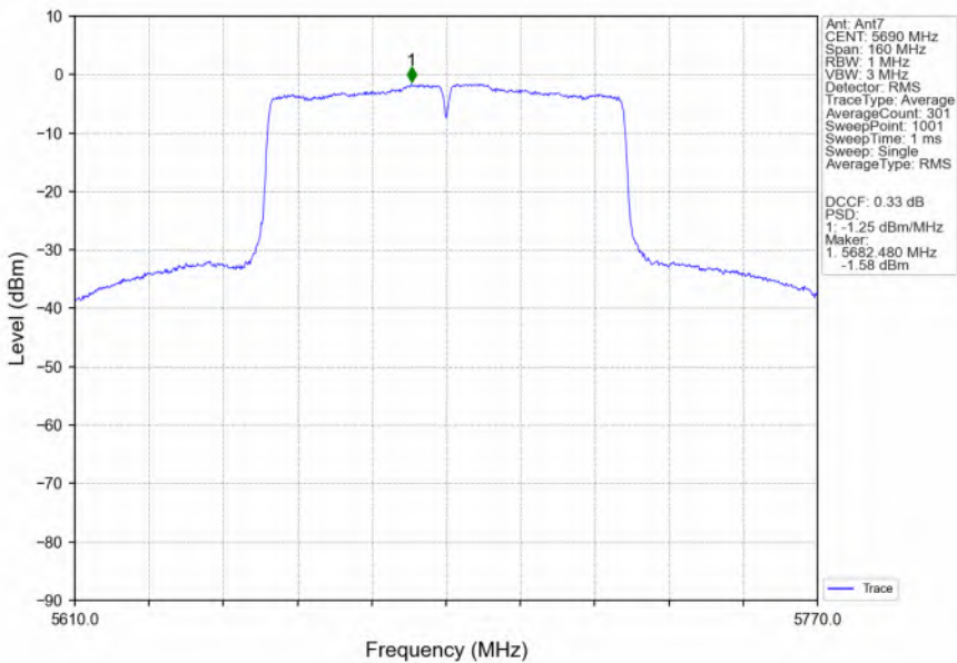
802.11ac(VHT80)_HCH_5690MHz_Ant7_NTNV
