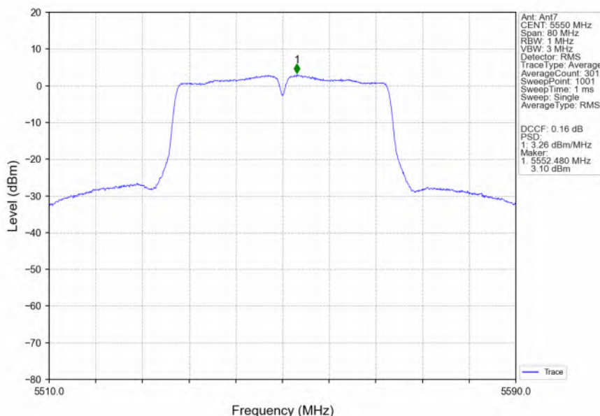
802.11ac(VHT40)_MCH_5550MHz_Ant7_NTNV
