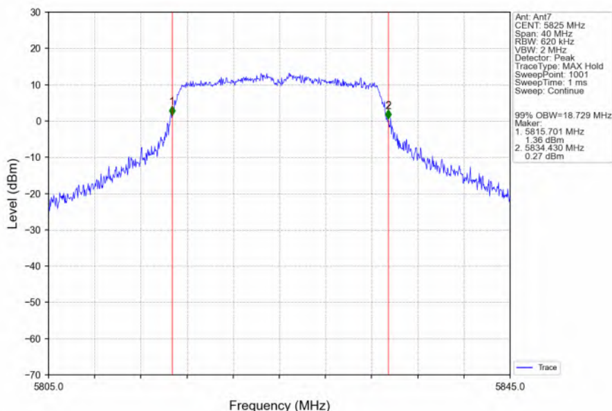
802.11ac(VHT20)_HCH_5825MHz_Ant7_NTNV
