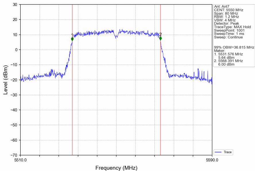
802.11n(HT40)_MCH_5550MHz_Ant7_NTNV
