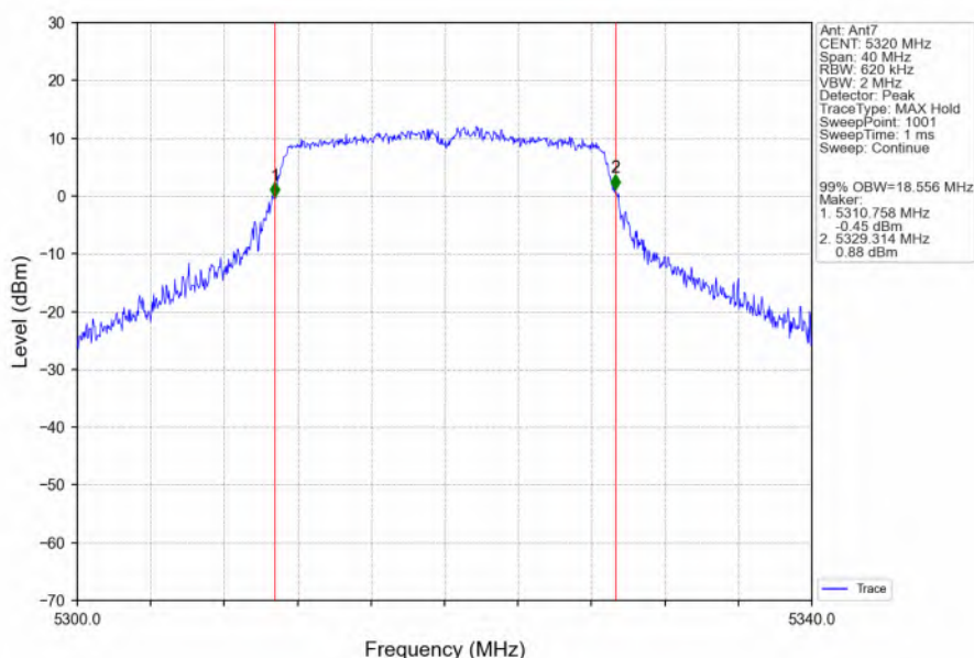
802.11ac(VHT20)_HCH_5320MHz_Ant7_NTNV
