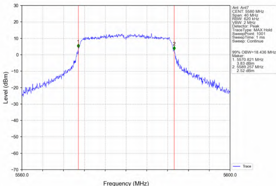
802.11ac(VHT20)_MCH_5580MHz_Ant7_NTNV
