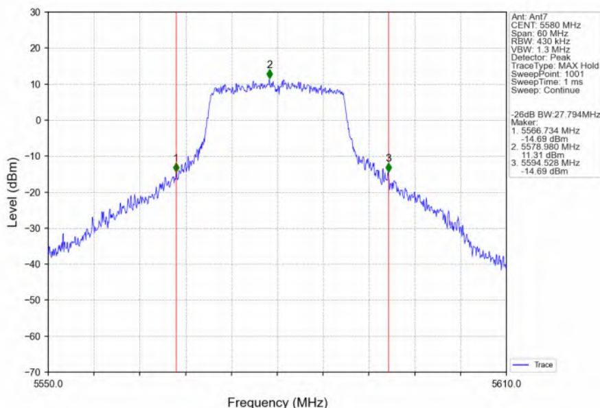
802.11ac(VHT20)_MCH_5580MHz_Ant7_NTNV
