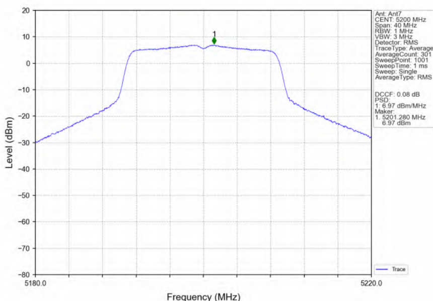
802.11ac(VHT20)_MCH_5200MHz_Ant7_NTNV
