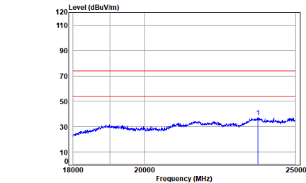
BT_DH5_TX_CH_00_Horizontal
