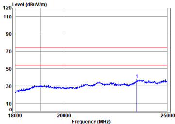
BLE_1M_TX_CH_39_Vertical
