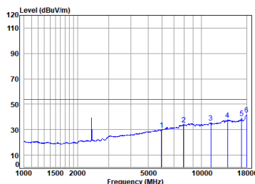
BLE_1M_TX_CH_00_Horizontal-Avg
