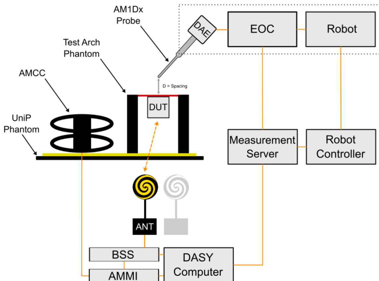
Fig. 1. The SPEAG Robotic Diagram
