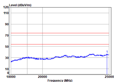
11g_TX_CH_11_Vertical
