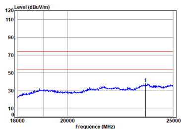
11g_TX_CH_01_Vertical
