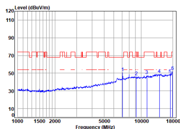
11a_TX_CH_60_Vertical
