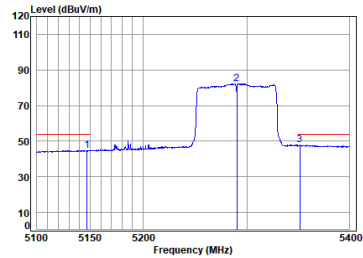
11ac_VHT(80M)_TX_CH_58_Vertical-Avg
