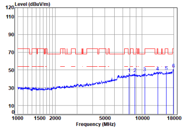
11ac_40M_Straddle_TX_CH_142_Vertical
