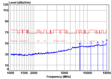
11ac_40M_Straddle_TX_CH_142_Horizontal
