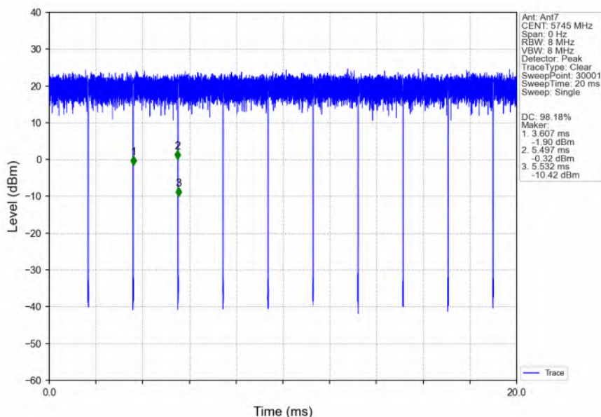
802.11ac(VHT20)_LCH_5745MHz_Ant7_NTNV
