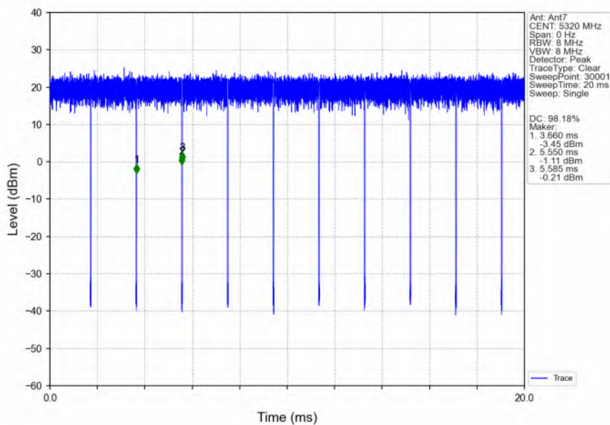
802.11ac(VHT20)_HCH_5320MHz_Ant7_NTNV
