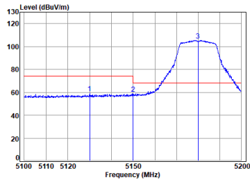
11ac_VHT(20M)_TX_CH_36_Horizontal-Peak
