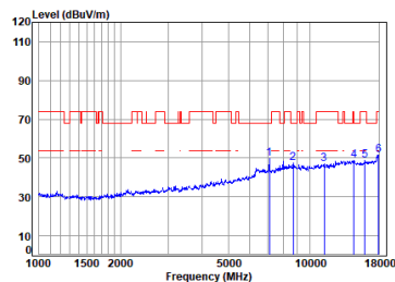
11a_TX_CH_64_Vertical
