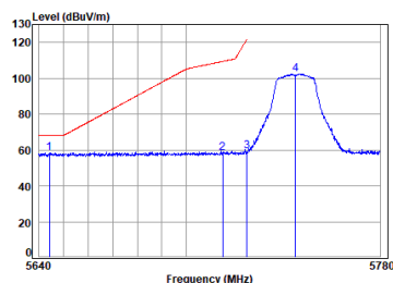
11a_TX_CH_149_Vertical
