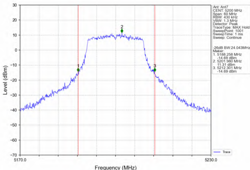
802.11ac(VHT20)_MCH_5200MHz_Ant7_NTNV
