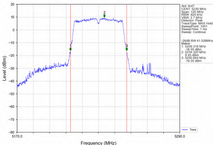
802.11ac(VHT40)_HCH_5230MHz_Ant7_NTNV
