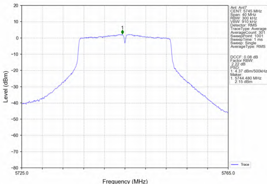
802.11ac(VHT20)_LCH_5745MHz_Ant7_NTNV
