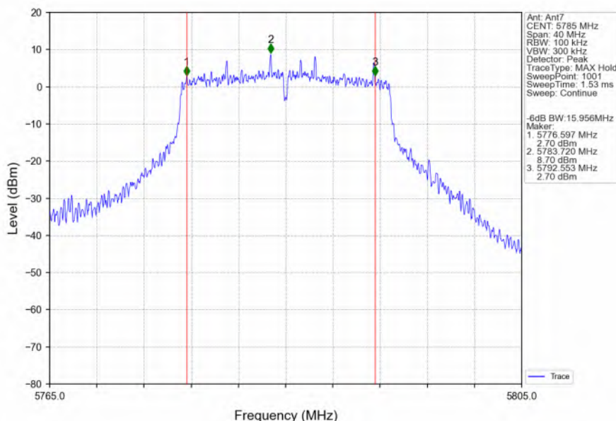
802.11ac(VHT20)_MCH_5785MHz_Ant7_NTNV
