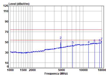
11g_TX_CH_11_Vertical
