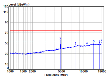
11g_TX_CH_06_Vertical
