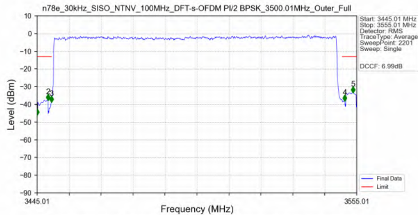
n78e_30kHz_SISO_NTNV_100MHz_DFT-s-OFDM PI/2 BPSK_3500.01MHz_Outer_Full_Ant2
