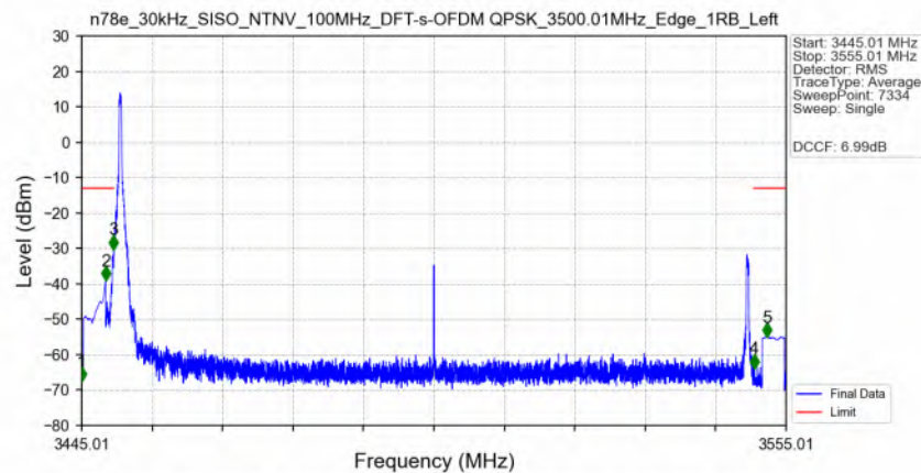
n78e_30kHz_SISO_NTNV_100MHz_DFT-s-OFDM QPSK_3500.01MHz_Edge_1RB_Left_Ant2
