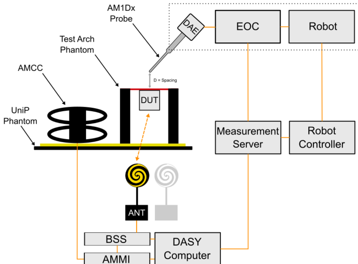
Fig. 1. The SPEAG Robotic Diagram
