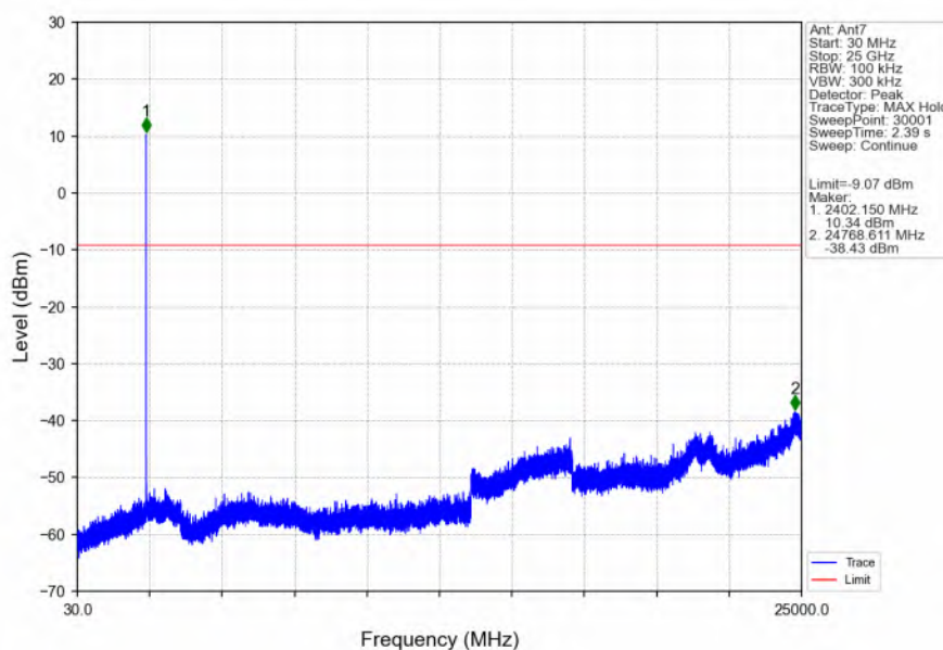
GFSK_DH5_LCH_2402MHz_Ant7_NTNV
