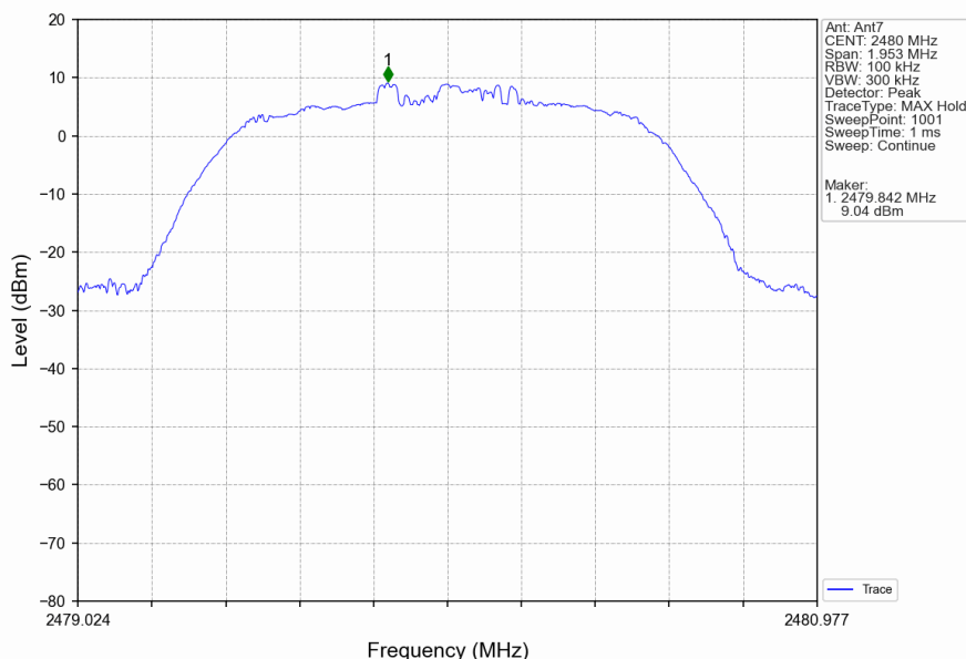
Pi/4DQPSK_2DH5_HCH_2480MHz_Ant7_NTNV
