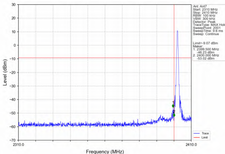
GFSK_DH5_LCH_2402MHz_Ant7_NTNV
