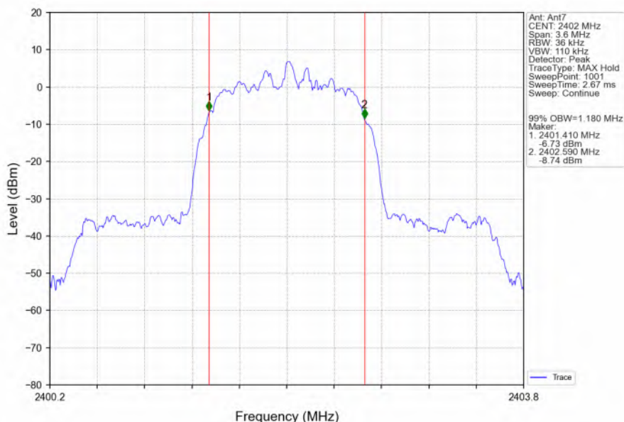
Pi/4DQPSK_2DH5_LCH_2402MHz_Ant7_NTNV
