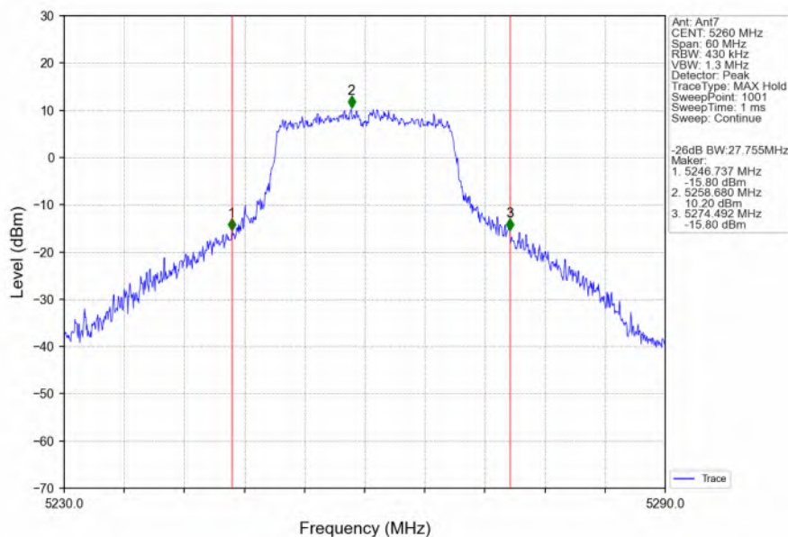
802.11ac(VHT20)_LCH_5260MHz_Ant7_NTNV
