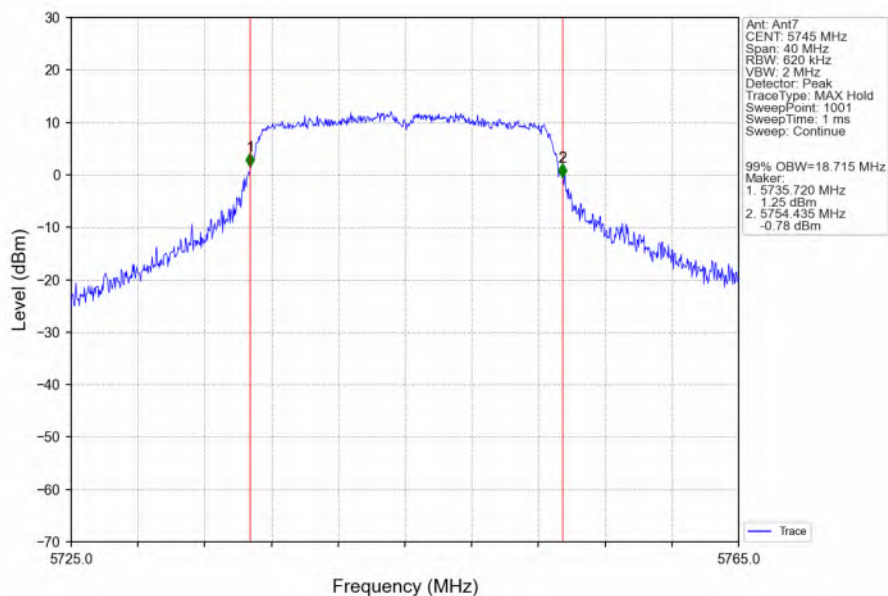
802.11ac(VHT20)_LCH_5745MHz_Ant7_NTNV
