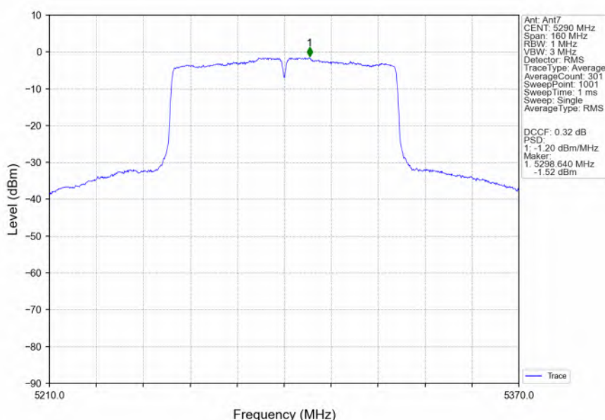
802.11ac(VHT80)_MCH_5290MHz_Ant7_NTNV
