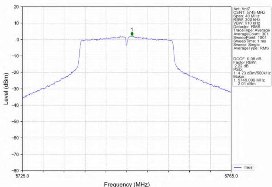
802.11ac(VHT20)_LCH_5745MHz_Ant7_NTNV
