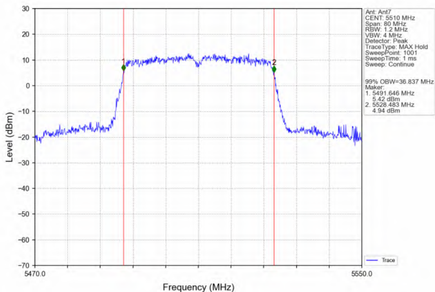
802.11ac(VHT40)_LCH_5510MHz_Ant7_NTNV
