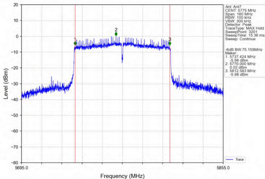
802.11ac(VHT80)_MCH_5775MHz_Ant7_NTNV
