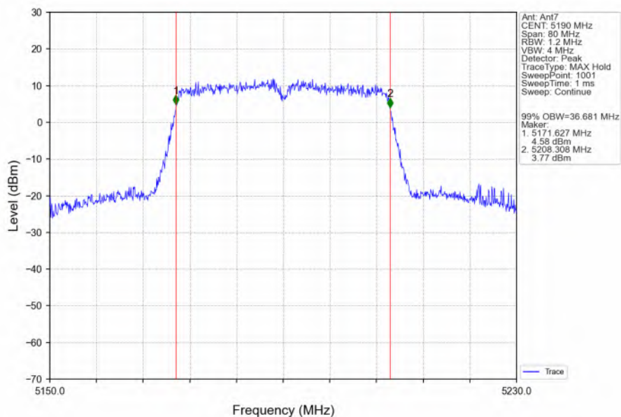
802.11ac(VHT40)_LCH_5190MHz_Ant7_NTNV
