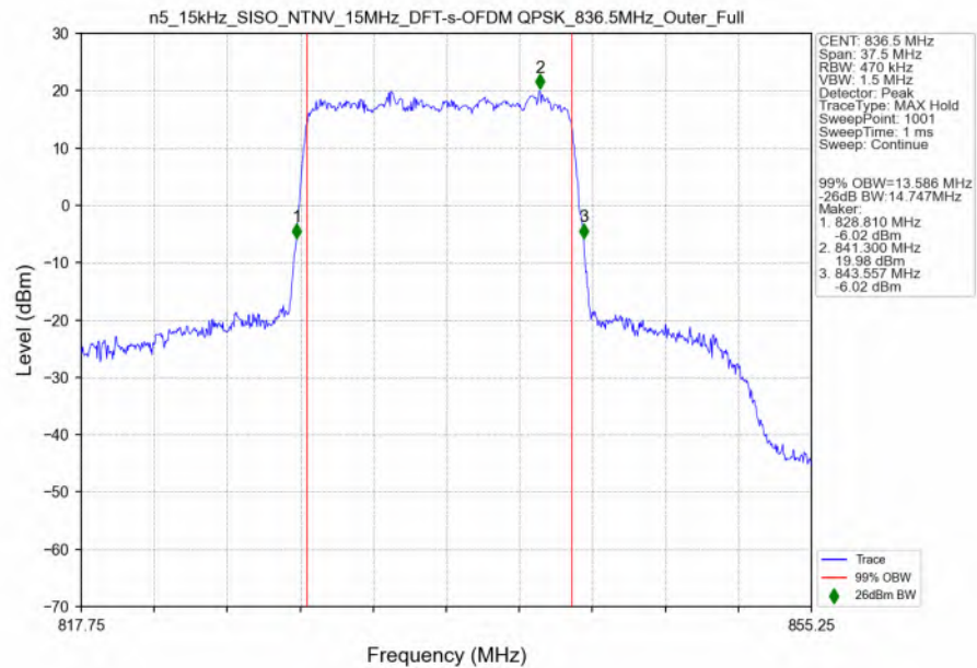
n5_15kHz_SISO_NTNV_15MHz_DFT-s-OFDM QPSK_836.5MHz_Outer_Full_Ant0
