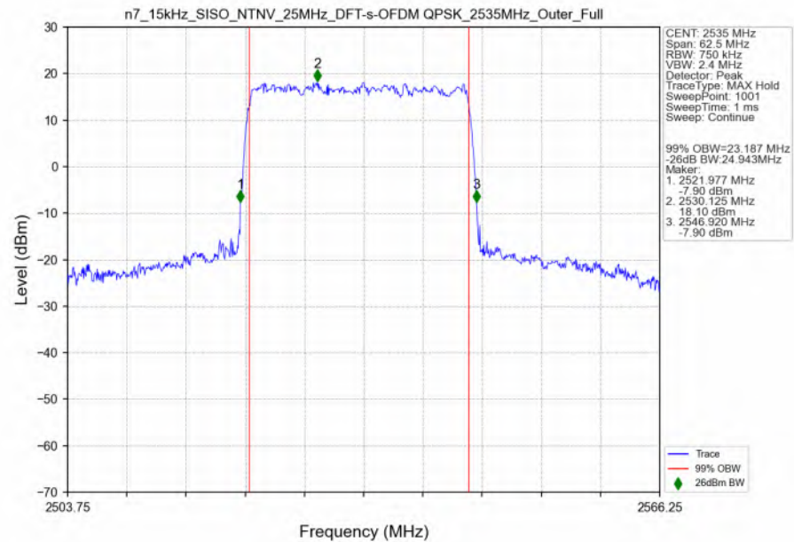
n7_15kHz_SISO_NTNV_25MHz_DFT-s-OFDM QPSK_2535MHz_Outer_Full_Ant4
