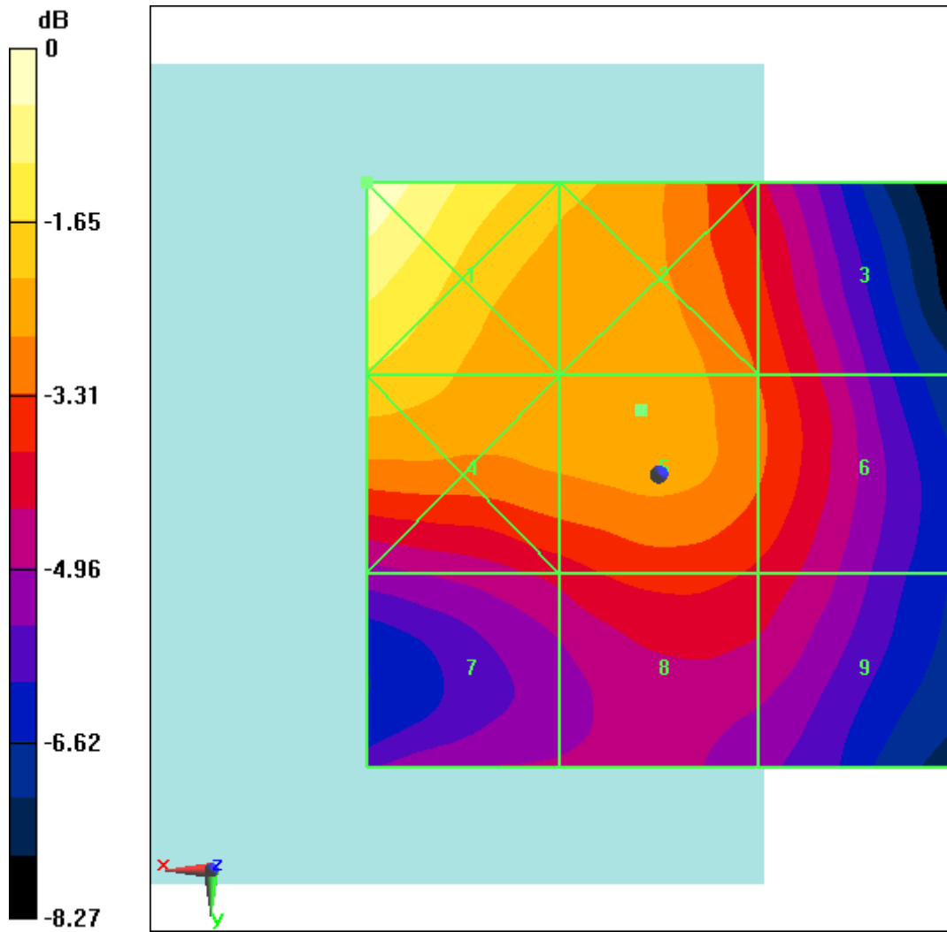
Fig B.11 HAC RF E-Field LTE Band41 QPSK CH39750
