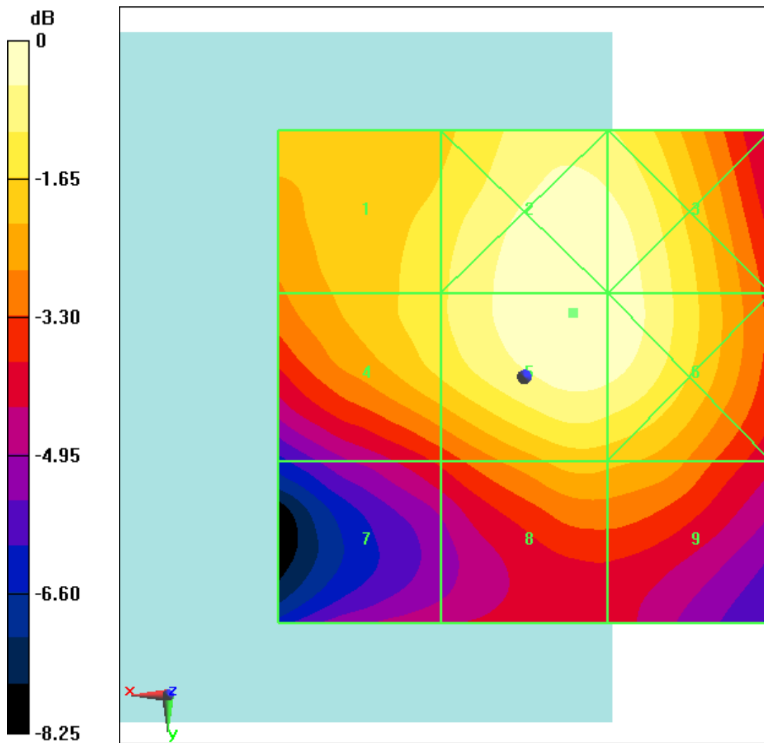
Fig B.21 HAC RF E-Field LTE Band41 64QAM CH39750
