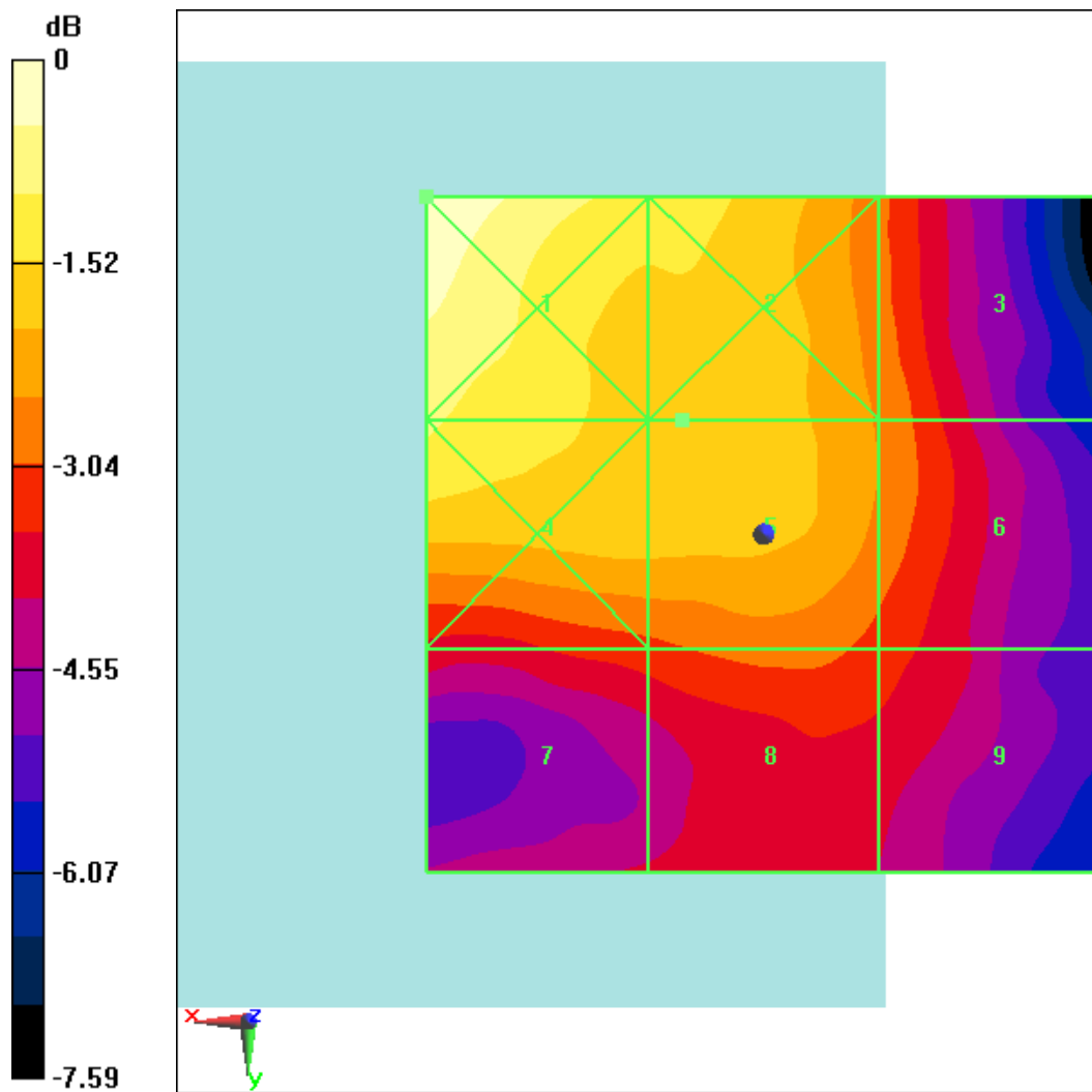
Fig B.13 HAC RF E-Field LTE Band41 16QAM CH41055
