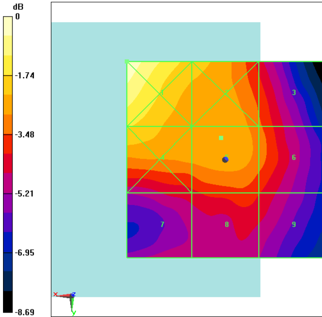
Fig B.16 HAC RF E-Field LTE Band41 16QAM CH39750
