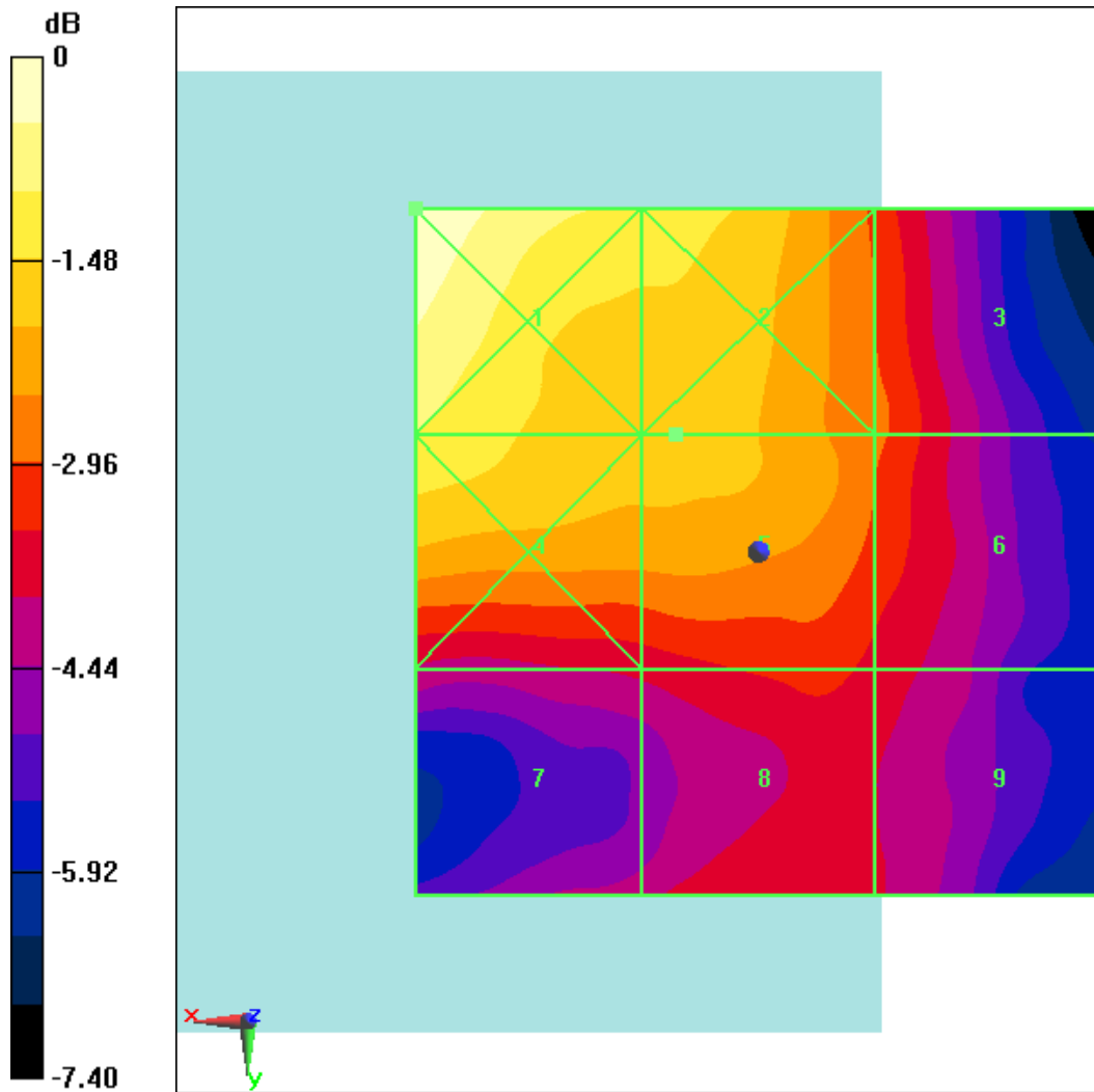
Fig B.14 HAC RF E-Field LTE Band41 16QAM CH40620
