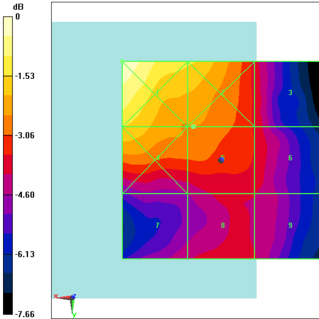
Fig B.15 HAC RF E-Field LTE Band41 16QAM CH40185
