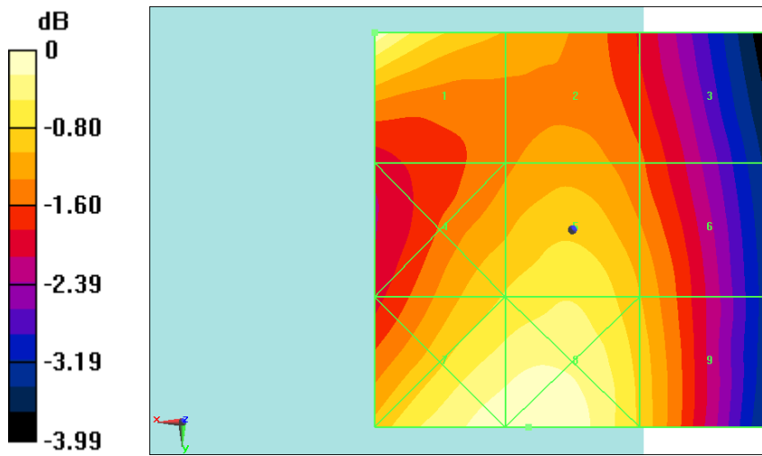
Fig B.1 HAC RF E-Field GSM 850 Low
