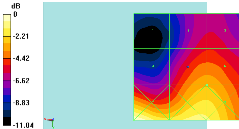
Fig B.8 HAC RF E-Field WiFi2.4G 11M
