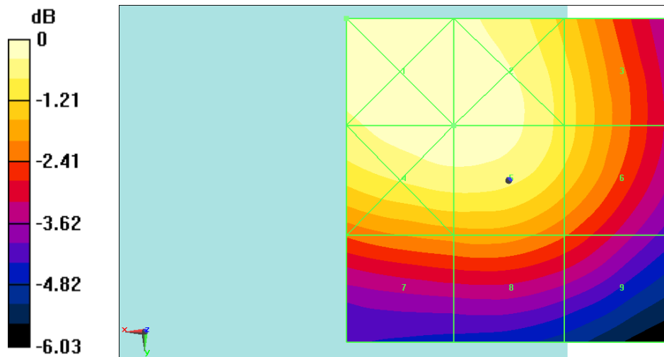
Fig B.7 HAC RF E-Field LTE Band41 Power Class 3 QPSK CH41490
