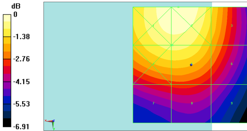
Fig B.6 HAC RF E-Field LTE Band41 Power Class 2 16QAM CH41490
