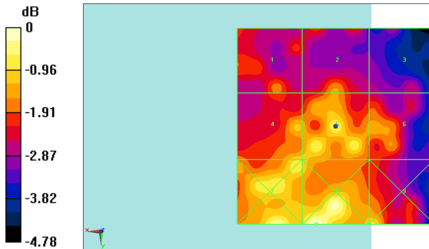
Fig B.3 HAC RF E-Field CDMA BC0 low
