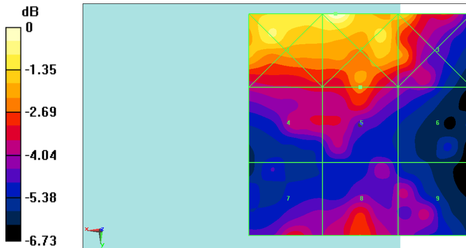
Fig B.4 HAC RF E-Field CDMA BC1 Low
