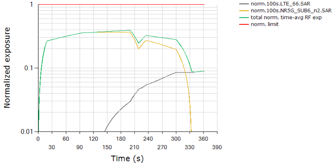
Total Normalized Time-averaged RF Exposure Tech: LTE, Band 66 / Tech: NR5G SUB6, Band n2
