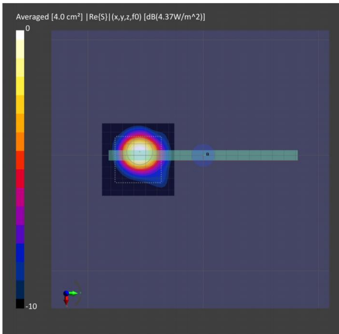
Figure 8-2: 4cm2-averaged power density distribution measured at input.power.limit of 3.18dBm on the back surface for n261 beam 27
