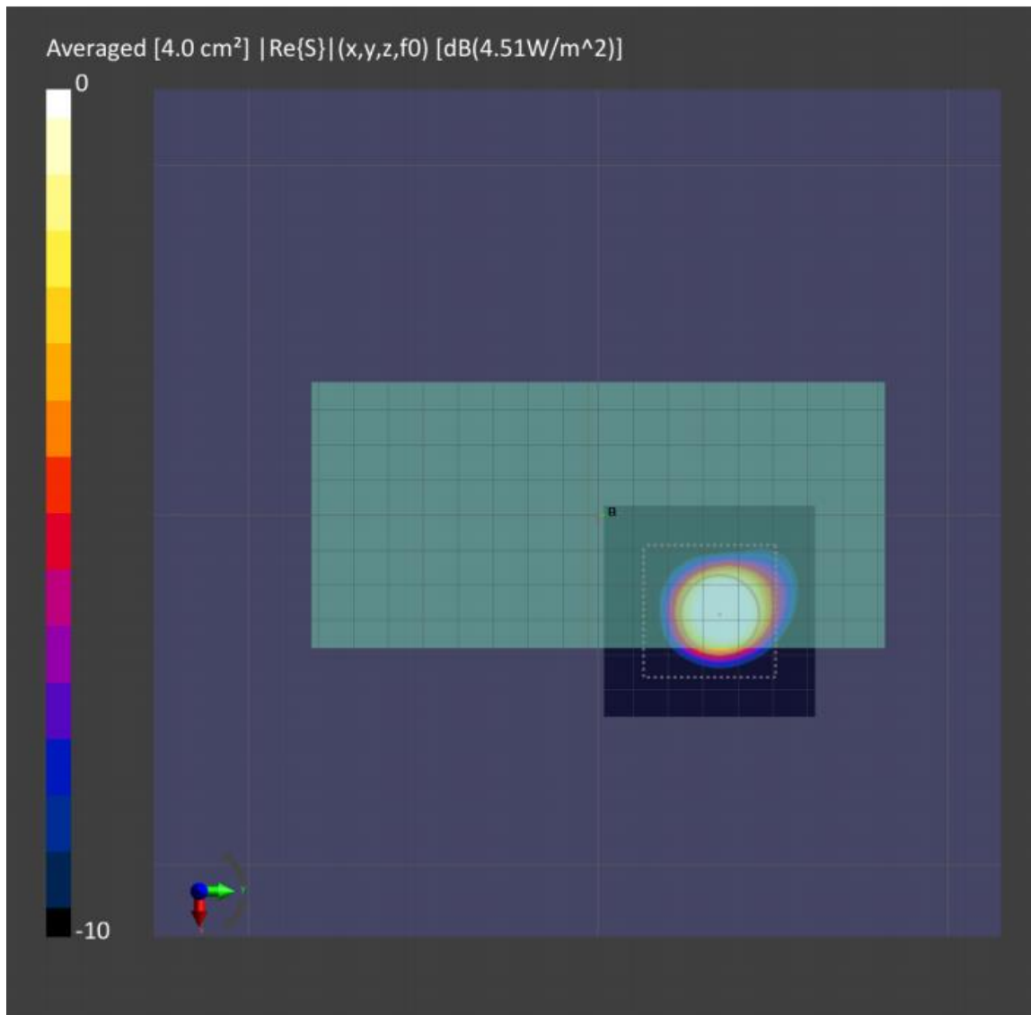
Figure 8-3: 4cm2-averaged power density distribution measured at input.power.limit of 11.97 dBm on the Back for n260 beam 0
