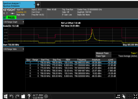
N14(10M)_DFT-s-OFDM_QPSK_Edge_1RB_Left_Mid_CH
