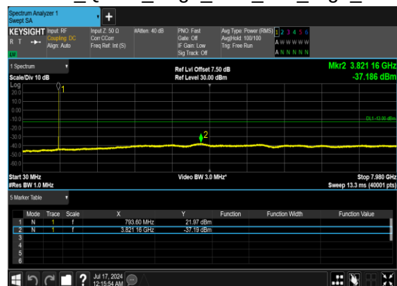
N14(5M)_DFT-s- OFDM_QPSK_Edge_1RB_Left_High_CH
