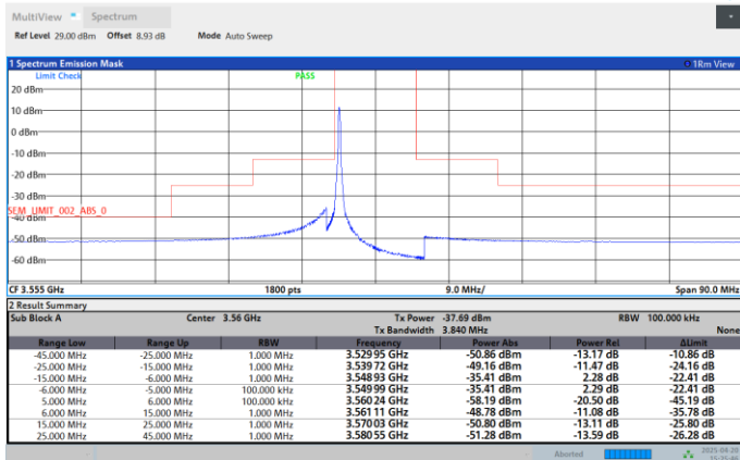
Band48-10MHz-64QAM-3555-50RB#0-PASS
