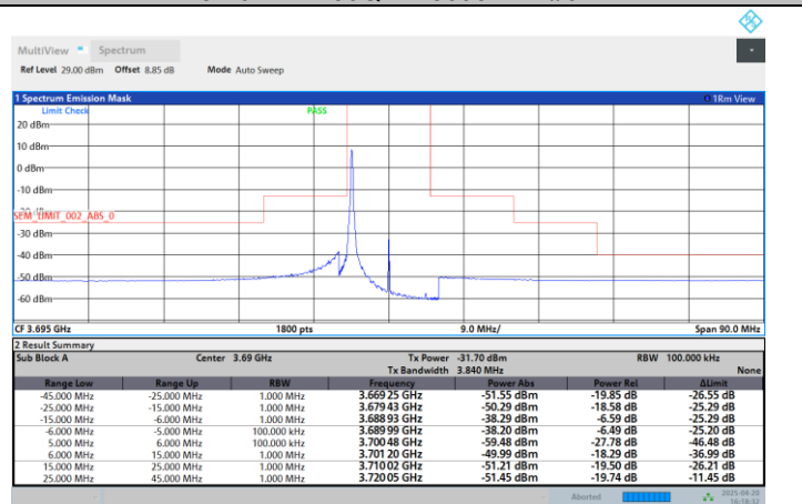
Band48-10MHz-256QAM-3695-50RB#0-PASS
