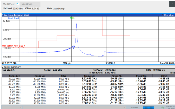
Band48-15MHz-QPSK-3557.5-75RB#0-PASS
