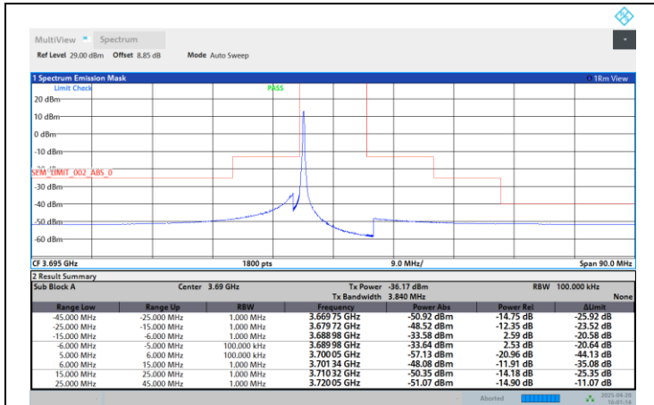
Band48-10MHz-QPSK-3695-50RB#0-PASS
