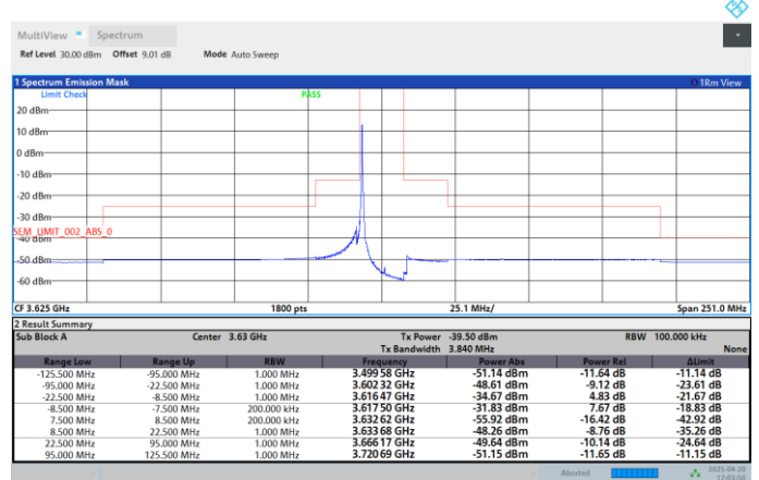
Band48-15MHz-QPSK-3625-75RB#0-PASS
