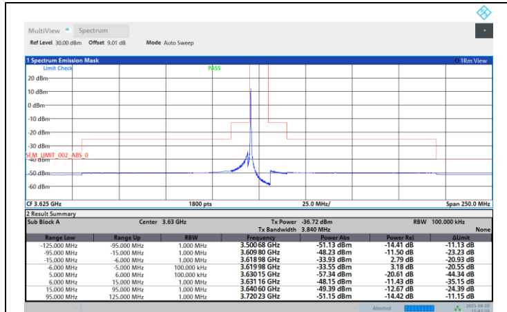
Band48-10MHz-16QAM-3625-50RB#0-PASS
