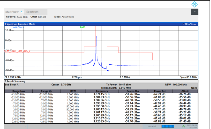
Band48-5MHz-256QAM-3697.5-25RB#0-PASS
