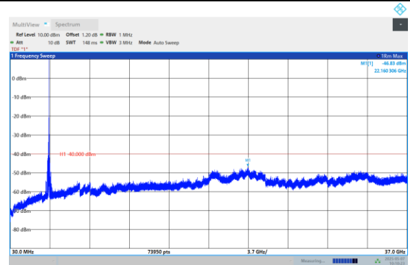
Band48-10MHz-QPSK-3555-1RB#0-Range:30~37000M Hz
