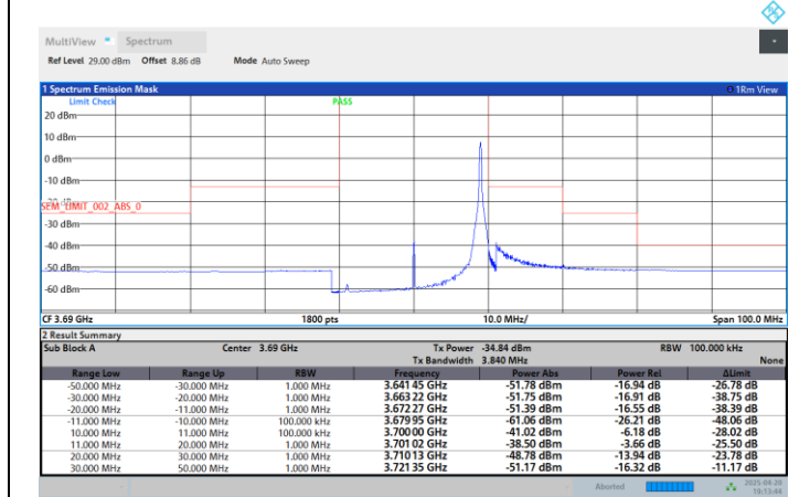
Band48-20MHz-256QAM-3690-1RB#99-PASS
