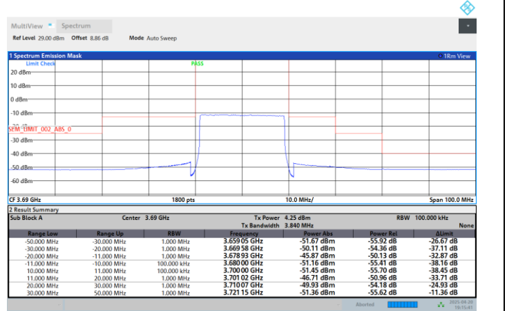
Band48-20MHz-256QAM-3690-100RB#0-PASS
