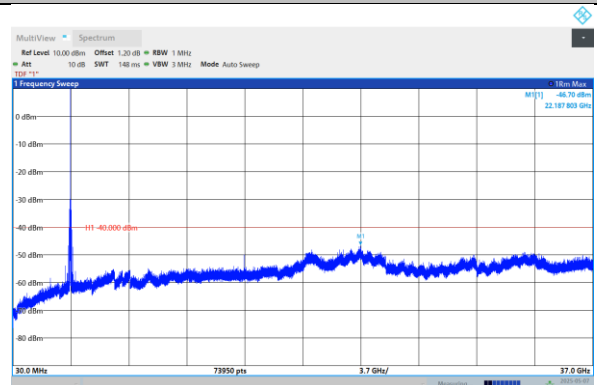
Band48-15MHz-QPSK-3625-1RB#0-Range:30~37000M Hz
