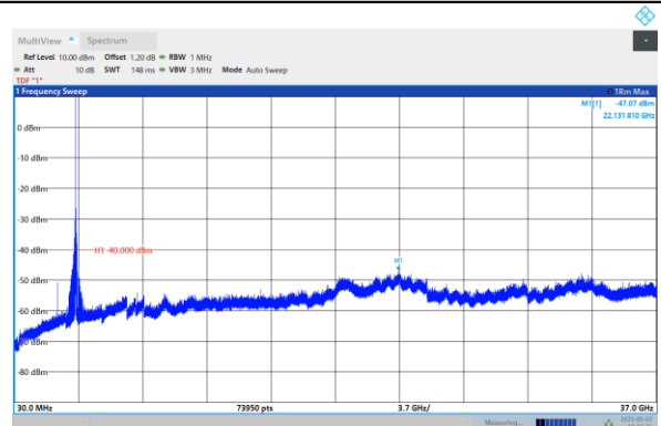
Band48-10MHz-QPSK-3695-1RB#0-Range:30~37000M Hz
