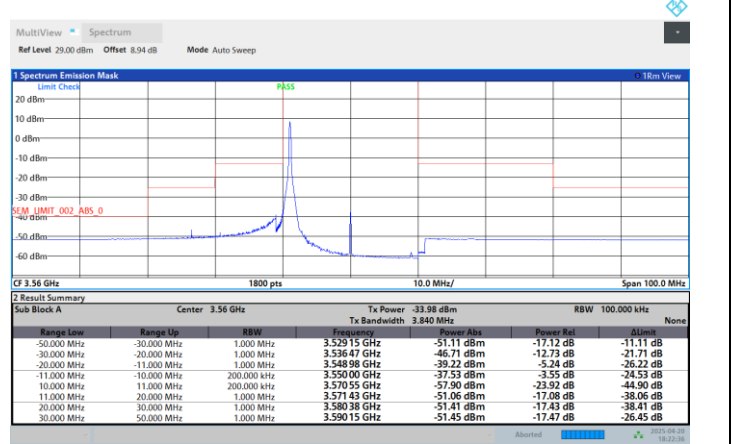
Band48-20MHz-256QAM-3560-100RB#0-PASS
