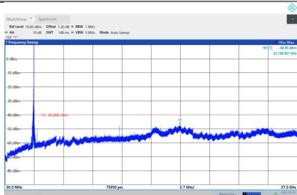
Band48-15MHz-QPSK-3557.5-1RB#0-Range:30~37000 MHz
