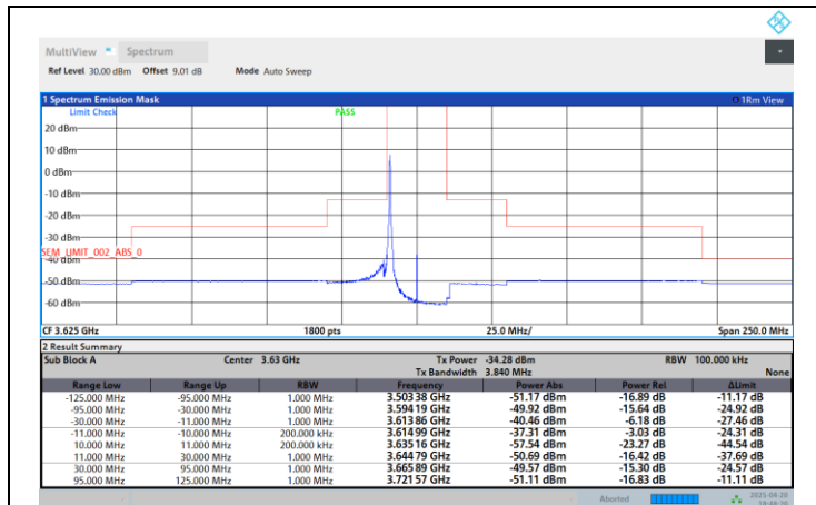
Band48-20MHz-256QAM-3625-100RB#0-PASS
