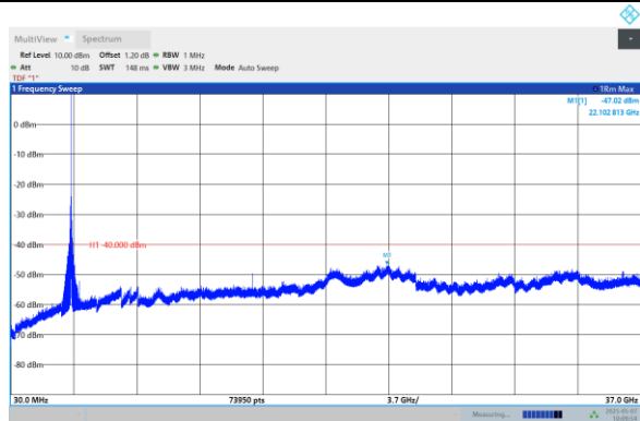
Band48-5MHz-QPSK-3697.5-1RB#0-Range:30~37000M Hz
